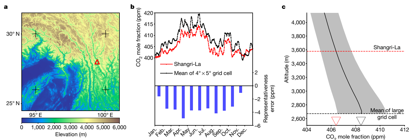
Fig. 2 | Representativeness of site Shangri-La in the inversion system.
