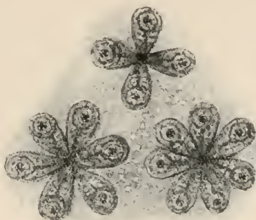
FIG. 122.— Botryllus rubens . Systems of from four to seven individuals. Enlarged.
