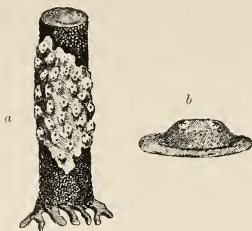
FIG. 108.— Distoma variolosum . (After Gaertner, loc. cit. ) a , a colony, natural size; b , a single individual, enlarged.
