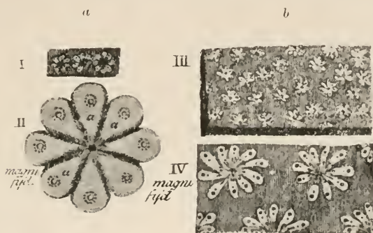
FIG. 125.—Borlase's two species of Botryllus referred by him to Alcyonium . Natural size and magnified. a, B. Schlosseri . b, ? B. smaragdus . (After Borlase, loc. cit. )
