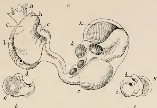
FIG. 105.—Individuals of Didemnum candidum . Enlarged. (Savigny,* pl. xx, ff. 1 2 -4.) a . Details of an individual seen from the right side, much enlarged. b . Another individual deprived of its thorax and less enlarged than the preceding; its intestine and ovary differently disposed. Seen from the left side. c . The same reversed. B , branchial aperture; C , mantle; C , atrial aperture; c , stomach; d , intestine; h , anterior (branchial) tubercle; K , ovary; k , excrement contained in the intestine; l , dorsal lamina.
