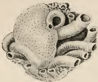
FIG. 101.— Didemnum gelatinosum , fixed on a mass of Serpula . Natural size. (M. Edwards, pl. vii, f. 5.)
