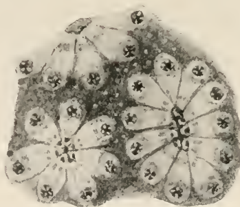
FIG. 123.— Botryllus virescens . Systems of from seven to eleven individuals. Enlarged.
