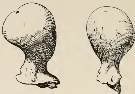
FIG. 99.—? Aplidium ficus . Two colonies, one half natural size. (After Mercati, loc. cit. )
