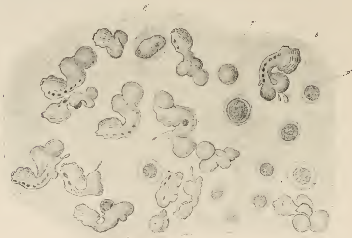
FIG. 103.—Part of a colony of Didemnum gelatinosum , enlarged. a , common tegumentary tissue; b , an individual immersed in the tissue; p' , an egg only a little developed; p'' , an egg more developed. (M. Edwards, pl. vii, f. 5a.)
