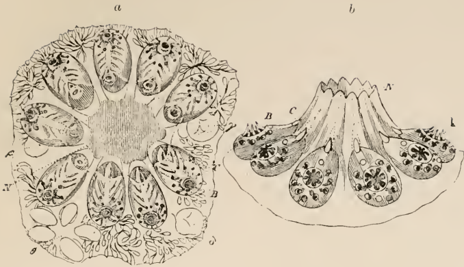
FIG. 127.—Systems of individuals of Botryllus polycyclus . Much enlarged. (Savigny, pl. xxi, ff. 1 1 and 1 2 .) a . A system in a state of contraction, seen from above. b . A system in a state of dilatation, seen from the side. B , branchial aperture; C , atrial aperture; N , common excretory cavity; k , tentacular filaments; \beta , \gamma , \delta , \theta , systems commencing to develop.
