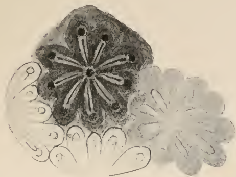
FIG. 129.— Botryllus miniatus . Systems, enlarged.
