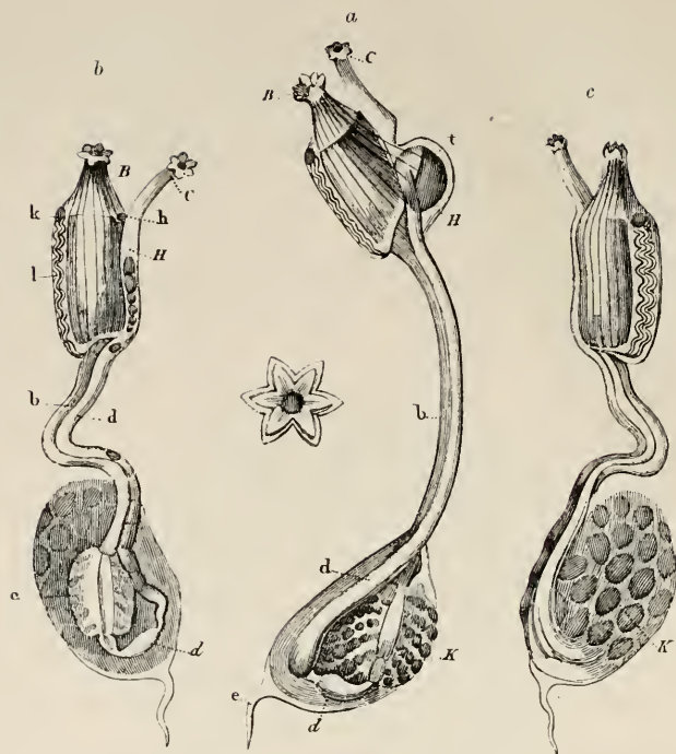
FIG. 107.—Individuals of Distoma rubrum . Much enlarged. (Savigny, pl. xiii, ff. 1 4, 8, 9 .) a . An individual seen from the right side; with branchial aperture further enlarged. b . Another individual differing in the forward bend of the intestine and the curvature of the peduncle of the abdomen. c . The same reversed. B , branchial aperture; h , oesophagus; C , atrial aperture; c , caecum of the stomach; d , intestine; d , swelling of the intestine near the pylorus; e , prolongation of the mantle in the base of the test, or in its peduncle; H , anal aperture; h , anterior (branchial) tubercle; K , ovary; k , posterior tubercle; l , dorsal lamina; t , an isolated germ being protruded from the anal aperture.
