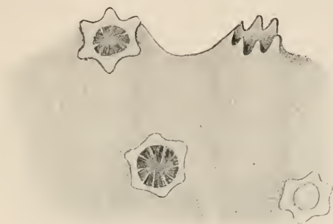
FIG. 111.—Part of a colony of Leptoclinum gelatinosum . Enlarged. (M. Edwards, pl. viii, f. 1 a.)
