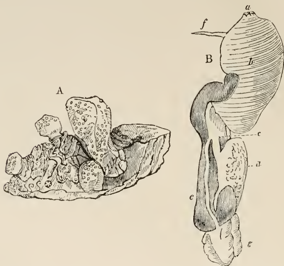
FIG. 96.— Amaroucium fallax . A, a group, natural size. B, a single individual, \times about 16. (After Johnston, loc. cit. ) a, branchial aperture; b, branchial sac; c, oesophagus; d, stomach; e, intestine; f, atrial aperture; g, ovary.
