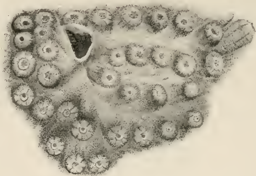
FIG. 132.— Botrylloides rotifera . Part of a colony enlarged. (M. Edwards, pl. vi, f. 1 a.)
