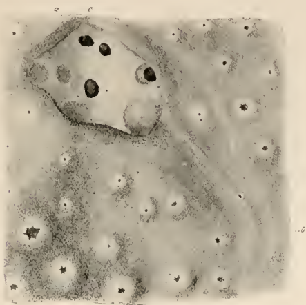
FIG. 110.—Part of a colony of Leptoclinum fulgens . (M. Edwards, pl. viii, f. 5 a.)
