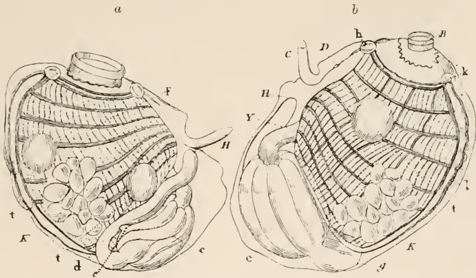
FIG. 128.—Individual of Botryllus polycyclus . Much enlarged. (Savigny, pl. xxi, ff. 1 3 and 1 4 .) a . Right side. b . Left side. B , branchial aperture; C , atrial aperture; c , stomach; c , caecum of the stomach; D , nerve-ganglion; d , intestine; F , branchial sac; g , intestinal loop; H , anal aperture; h , anterior (branchial) tubercle; K , ovary; k , posterior tubercle; l , dorsal lamina; t , “egg or germ” out of the ovary and approaching maturity; Y , oesophagus.
