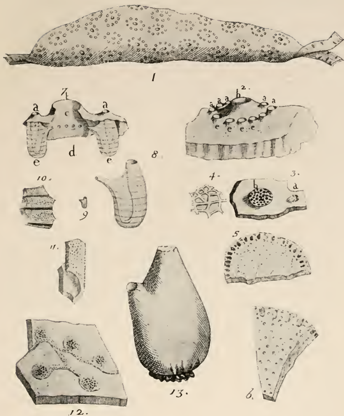
FIG. 115.—Structure of Botryllidae. “ Botryllus stellatus ” Renier in ‘Opusc. scelti Scienze,’ xvi (1793), pl. i; Polycyclus Renieri Lamarck in ‘Mém. du Mus.’ I (1815), p. 340. 1. A colony adhering to two fronds of Zostera , natural size. 2. A system, enlarged. a , branchial apertures; b , common excretory orifice; c , individuals. 3. Part of the same, viewed from above. b , common excretory orifice; d , branchial aperture. 4. A portion of the net-like bottom of b , fig. 3, further enlarged. 5. Transverse section of the colony, natural size. 6. Part of the same, enlarged. 7. Section of a system, enlarged. a , branchial apertures; c , common excretory canal; d , atrial apertures; e , individuals. 8. A single individual, further enlarged. 9. The same, natural size. 10. Part of the tunic (as seen in fig. 8), much enlarged. 11. A portion of the same, seen in profile, further enlarged. 12. Part of the common envelope, much enlarged, showing (probably) germs secreted in it. 13. An Ascidia , about natural size, introduced for comparison.
