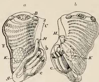
FIG. 114.—Structure of Botryllidæ. Botrylloides rosaceus (Sav.) M. Edw. (Savigny, pl. xx, ff. 3 2 , 3 3 .) a . An individual seen from the right side; the tunic supposed to be transparent and the branchial sac visible. b . Another individual seen from the left side. B , branchial aperture; C , atrial aperture; c , stomach; F , branchial sac; g , intestinal loop; H , anal aperture; K , ovary.
