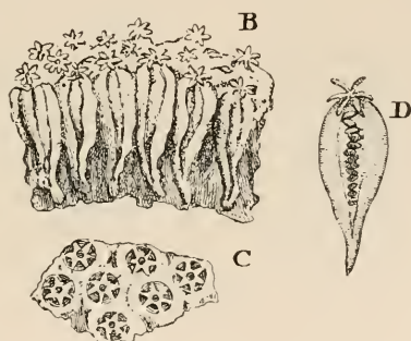
FIG. 98.— Aplidium ficus . Magnified. (After Ellis, loc. cit. ) B, section through part of the colony; C, face view of part of the colony; D, a single individual.
