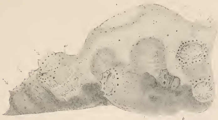
FIG. 113.— Leptoclinum Listerianum . \times 20 . (After Lister, loc. cit. ) “ a a , ledges on the interior of the branchial sac, each ending at a moveable spiral process in front, seen in two of the animals; b , the heart of one of them; c , vent of the same, with the viscera imperfectly seen.” The arrows, indicating the direction of the currents, show the branchial apertures and excretory orifices.
