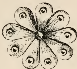
FIG. 119.—Face view of a system of Botryllus Schlosseri . Magnified. (After Ellis, loc. cit. , pl. xiv, f. C.)
