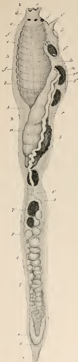
FIG. 93.—Isolated individual of Amaroucium argus . Much enlarged. (M. Edwards, pl. iii, f. 1.)
