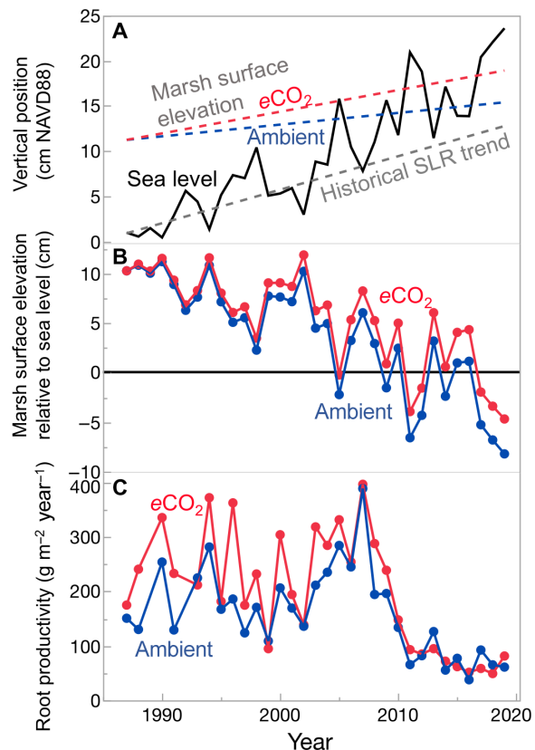
Fig. 6. Elevation trends in relation to root production. (A) Absolute elevations of marsh plots and sea level. Marsh elevations are based on elevation surveys and elevation change estimates modeled from an adjacent e\text{CO}_2 experiment, yielding rates for e\text{CO}_2 (red dashed line) and ambient \text{CO}_2 (blue dashed line) plots. The sea-level trace (black line) represents annual mean sea level for each growing season (May to July) from the Annapolis gauge. The historical rate of sea-level rise based on a linear fit of the 93-year record from the Annapolis NOAA gauge ( 3.7 \text{ mm year}^{-1} , dashed gray line) is plotted at the same starting point for comparison to the actual mean sea level over the interval of this study, 1987–2019. (B) Estimated marsh elevations relative to sea level for e\text{CO}_2 (red symbols) and ambient \text{CO}_2 (blue symbols). In a given year, marsh elevations below 0 are lower than sea level during the growing season. (C) Root production in e\text{CO}_2 (red symbols) and ambient (blue symbols) plots over 33 years.
