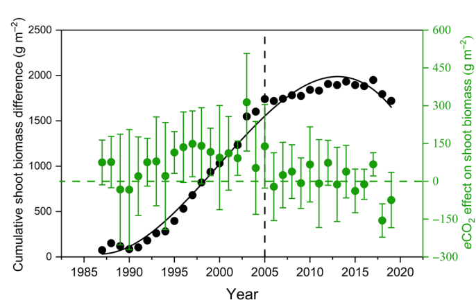
Fig. 2. Shoot biomass responses to e\text{CO}_2 . Shoot biomass responses to e\text{CO}_2 exposure from 1987 to 2019 plotted as both the annual difference in the mean biomass of the elevated (E) and ambient (A) treatments (right y axis in green symbols) and the cumulative difference in mean biomass of the two treatments over time (left y axis in black symbols). Cumulative shoot biomass data were fit to years of treatment with a fourth-order quadratic equation ( Y = 1170 + 3850X - 930X^2 - 826X^3 + 343X^4 , R^2 = 0.99 , P < 0.001 ).
