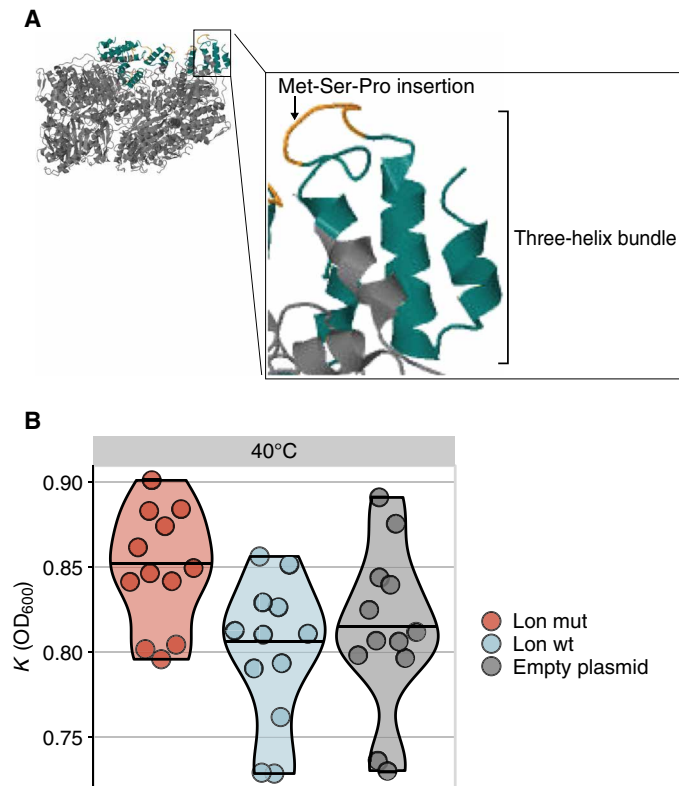
Fig. 3. Mutations in Lon protease are key for adaptation to high temperature. (A) Homology modeling of the three-amino acid (Met-Ser-Pro) insertion mutation (orange) of P. haloplanktis Lon protease (amino acids 253 to 775) using SWISS-MODEL and PDB structure 6v11 ( https://www.rcsb.org/structure/6V11 ) as a template. The structure is a homohexamer in which four of the six monomers are bound to ADP (adenosine 5'-diphosphate). The insertion occurs in a region known as the three-helix bundle in the N-terminal domain, which is colored in turquoise. (B) Maximum population density ( K ) in E. coli BL21 strain carrying an empty plasmid (gray), a plasmid expressing the wild-type Lon protease from P. haloplanktis (blue), or a plasmid expressing the mutated (Met-Ser-Pro insertion) Lon protease from P. haloplanktis (red). We performed 12 biological replicate measurements for each E. coli and plasmid combination (circles). mut, mutant; wt, wild type.
