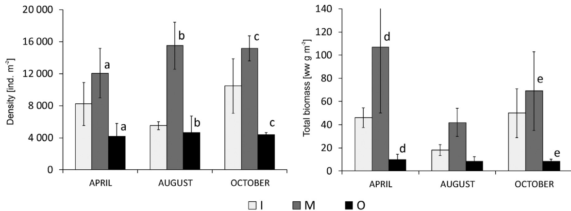
Figure 3 Density [ind. m -2 ] and total biomass [ww g m -2 ] of zoobenthos in the inner (I), middle (M), and outer zone (O) of the reed stand in the Vistula Lagoon. Small letters denote significant difference (Post-hoc Kruskal-Wallis test, p < 0.05 ) between areas marked with the same letter. No letter aside bar means no significant difference in density or biomass. Whiskers denote Standard Error.
