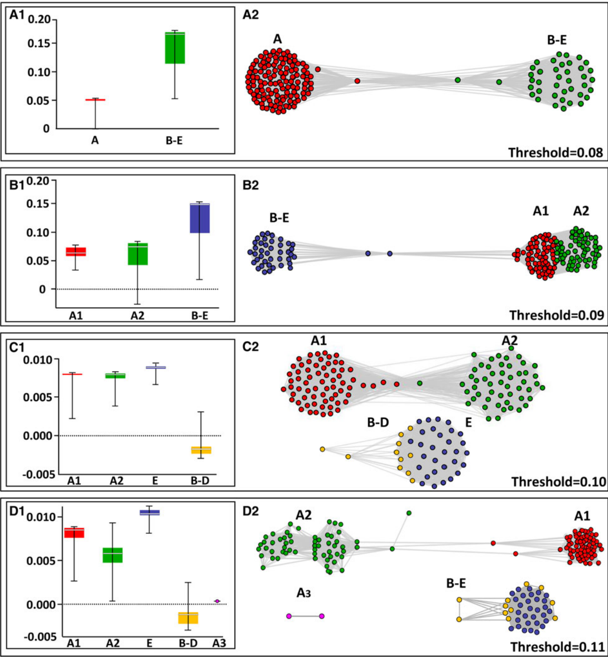
Fig. 4. NetStruct test results based on network theory for different threshold values. The left panels reflect the analysis results of strength of association distribution, using box whisker plots, with the strength of association values on the vertical axis. The spacing line in each box denotes the median. The right panels show the distribution of the haplotypes within the clades. Each circle represents one haplotype.
