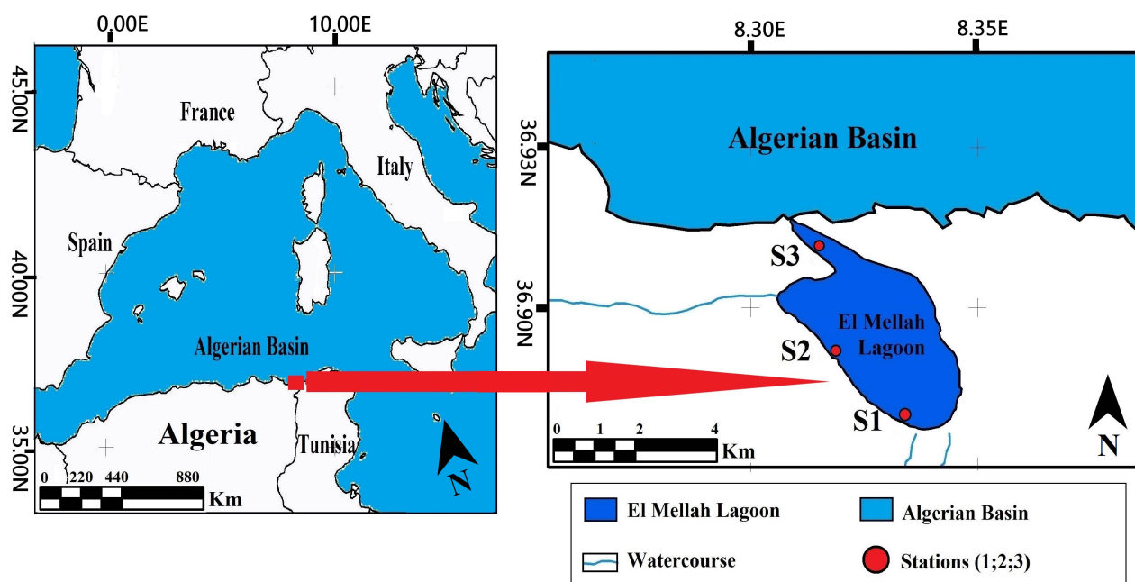
Figure 2. The location of the study area in the Mediterranean Sea and the location of the sampling stations in El Mellah Lagoon (Algeria, southern coast of the Algerian Basin) (Station 1: 36.87722N; 8.33083E; Station 2: 36.88722N; 8.31444E; Station 3: 36.90944N; 8.31444E).
