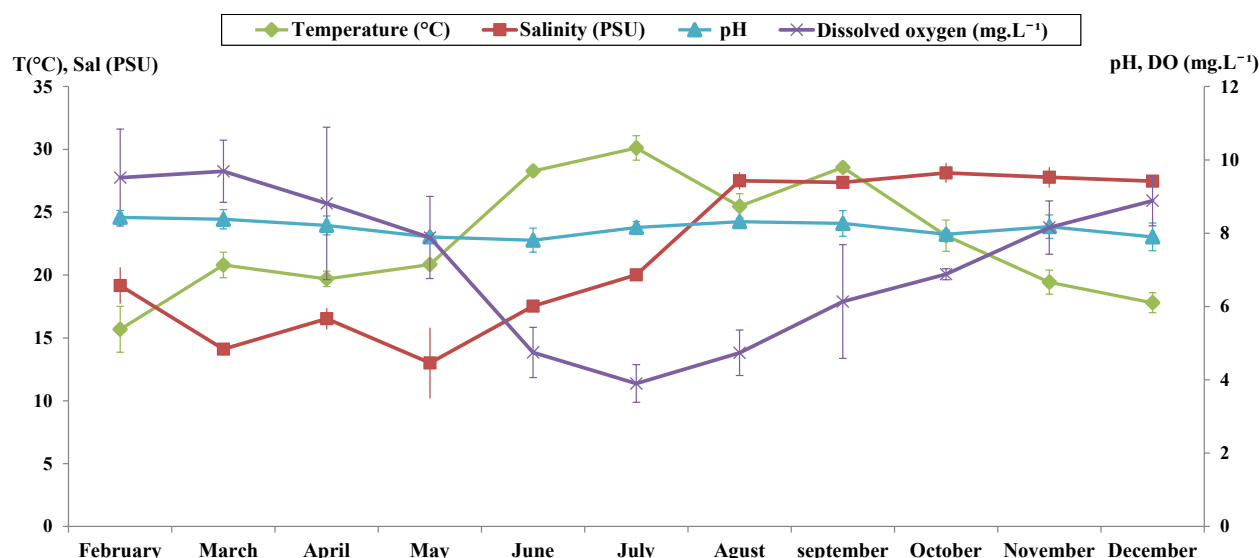
Figure 3. Mean values ( \pm SE) of temperature, salinity, dissolved oxygen and pH measured in the surface waters at the sampling stations in El Mellah Lagoon (Algeria, south-western Mediterranean Sea, see Figure 2) in 2019. T = temperature ( ^{\circ} C), Sal = salinity (PSU), DO = dissolved oxygen ( \text{mg.L}^{-1} ). N = 9 replicate measurements per month.
