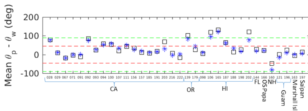
Figure 13. Average differences between wave peak direction ( \theta_p ) and wind direction ( \theta_w ) for rogue event and non-rogue cases. Rogue event data are depicted by black squares, and non-rogue data are shown as blue asterisks. Red dashed lines mark \pm 45^\circ . Green dashed lines mark \pm 90^\circ .
