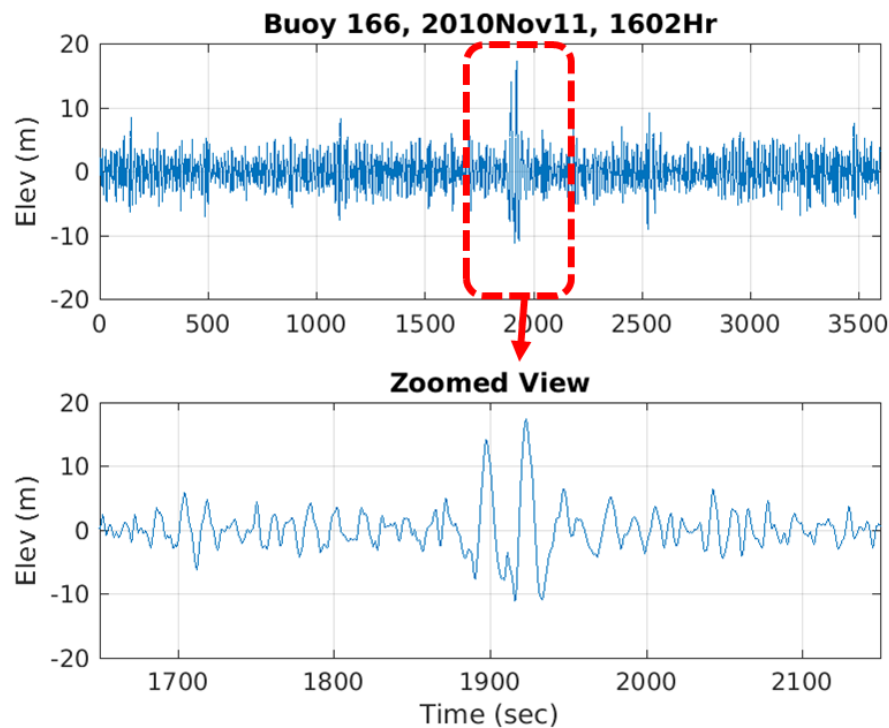
Figure 4. Top: Sample surface elevation time series from CDIP buoy 166, one hour of data beginning at 1602 UTC on Nov 11, 2010. Bottom: Zoomed view showing 500 s of data surrounding the 25.22 m rogue wave event. Ratio of H_r/H_s for the largest wave shown was 2.80.
