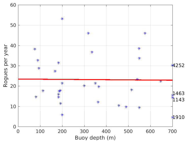
Figure 14. Rogue events per year versus water depth at each of the 34 buoy locations. Individual values plotted as blue asterisks, with best-fit shown by red line. Locations with depth greater than 700 m are plotted along the right vertical axis, with depth values listed next to each asterisk.
