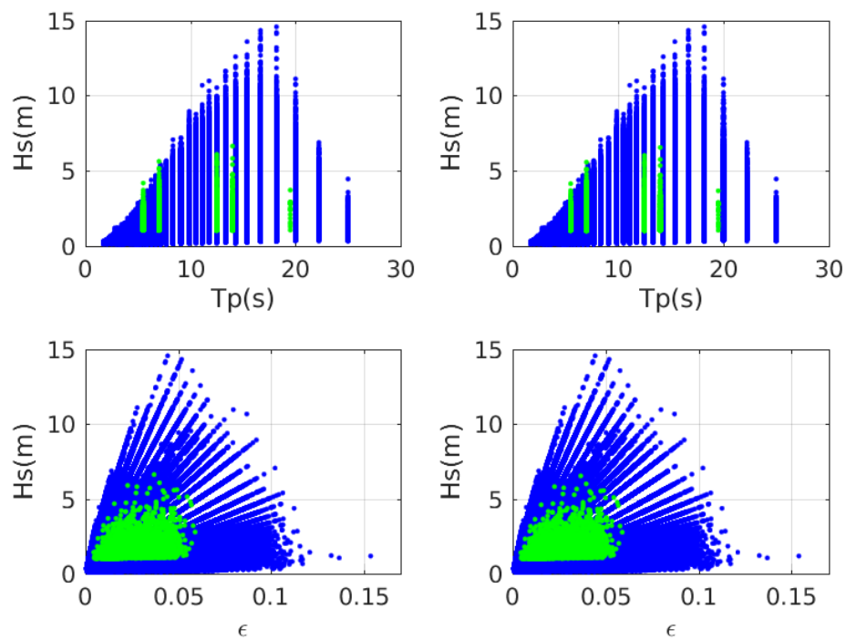
Figure 6. Comparison of H_s , T_p , and steepness ( \epsilon ) distributions for rogue (green) and non-rogue (blue) datasets. Left panels have rogue statistics computed with rogue events included in each sample. Right panels have rogue statistics computed with rogue events excluded from each sample.
