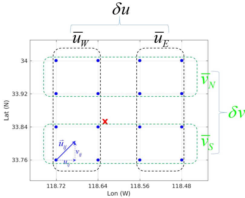
Figure 2. Determination of surface current shear, example for buoy 028 (located at red X). Velocity components \bar{u}_E, \bar{u}_W, \bar{v}_N, \bar{v}_S are averaged from groups of 8 points to E, W, N, and S of buoy location, and then shear along each Cartesian axis ( \delta u, \delta v ) is determined from these averaged velocities.
