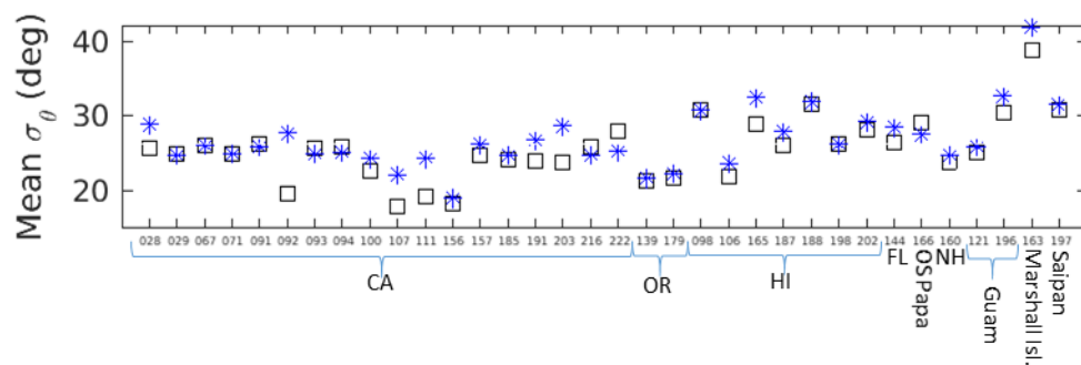
Figure 10. Average directional spread for rogue and non-rogue cases at all analyzed buoy sites. X-axis labels indicate buoy number and location. Rogue event data are depicted by black squares, and non-rogue data are shown as blue asterisks.
