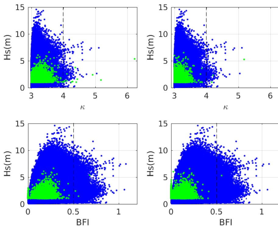
Figure 7. Comparison of H_s , kurtosis ( \kappa ), and BFI statistics for rogue (green) and non-rogue (blue) datasets. Left panels have rogue statistics computed with rogue events included in each sample. Right panels have rogue statistics computed with rogue events excluded from each sample. Heavier dashed vertical line added in each panel to better illustrate shift toward lower values when individual rogues are excluded.
