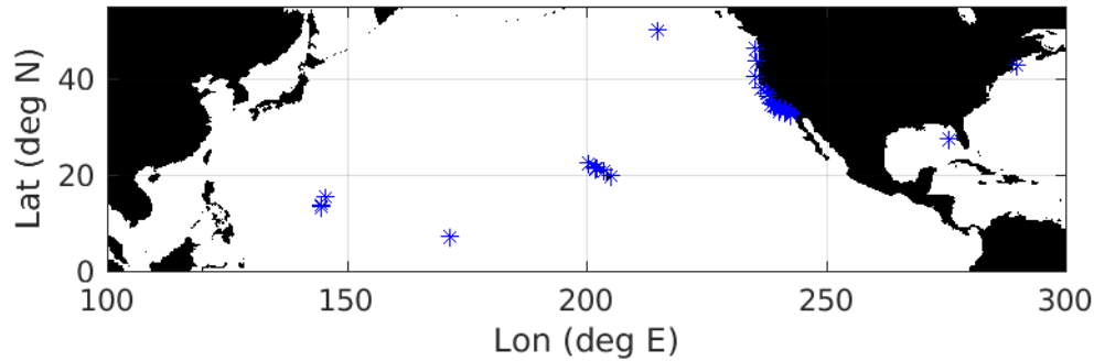
Figure 1. Locations of 34 analyzed Datawell buoys (blue asterisks).
