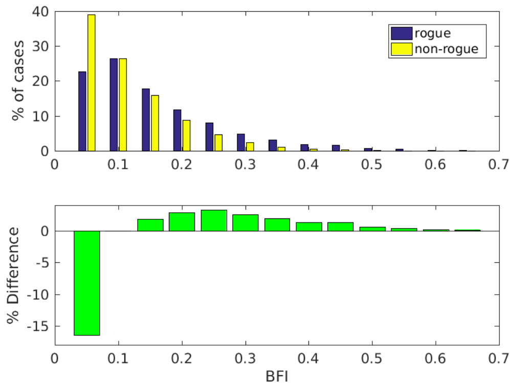
Figure 5. Comparison of BFI probability distributions for rogue and non-rogue datasets (all buoy locations combined). Top panel: Percentage of cases in selected BFI ranges for each dataset (bins centered from 0.05 to 0.65 with 0.05 width). Bottom panel: Difference in percentage of cases in selected BFI ranges. Positive values indicate a greater percentage of rogue wave events than non-rogue events for the specified BFI bin. (Values beyond 0.65 were too small to be visible on plots).
