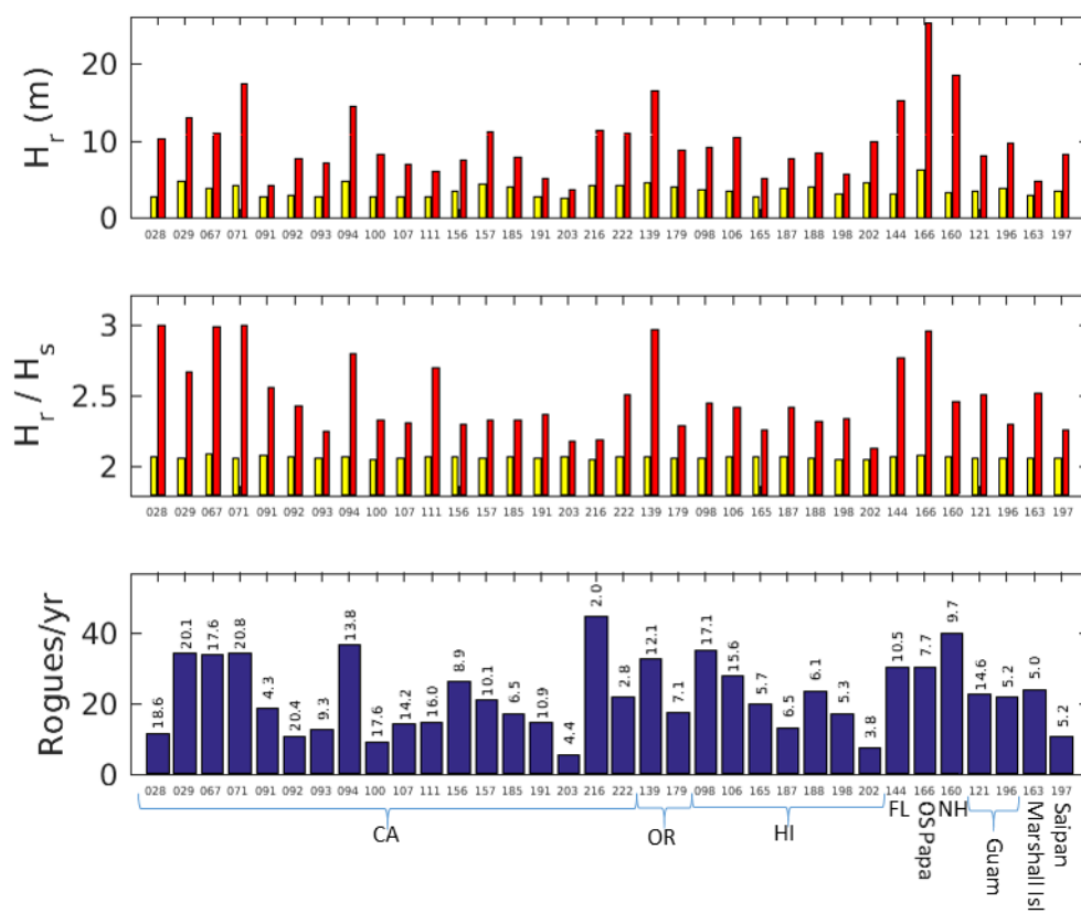
Figure 3. Rogue wave statistics at the 34 analyzed buoy locations. Top panel: Max (red bars) and Mean (yellow bars) rogue wave height. Middle panel: Max (red) and Mean (yellow) ratio of rogue height to significant wave height, as computed for each event at each buoy site. Bottom panel: Average number of rogues recorded per year at each site (values at top of each bar give total length of dataset at the site, in years). Buoy numbers are provided on the x-axis, with geographical buoy locations specified at bottom.
