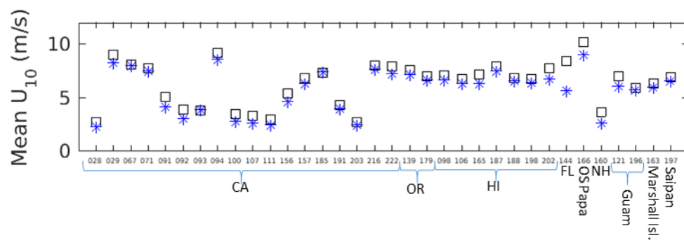
Figure 12. Average wind magnitude at each buoy location for rogue event and non-rogue cases. Rogue event data are depicted by black squares, and non-rogue data are shown as blue asterisks.
