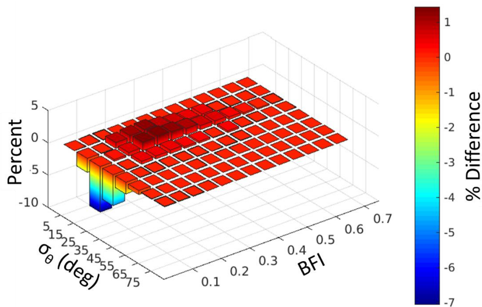
Figure 9. Combined difference histogram showing percentage difference (rogue minus non-rogue) as a function of both BFI and directional spread ( \sigma_\theta ), all buoy locations combined.
