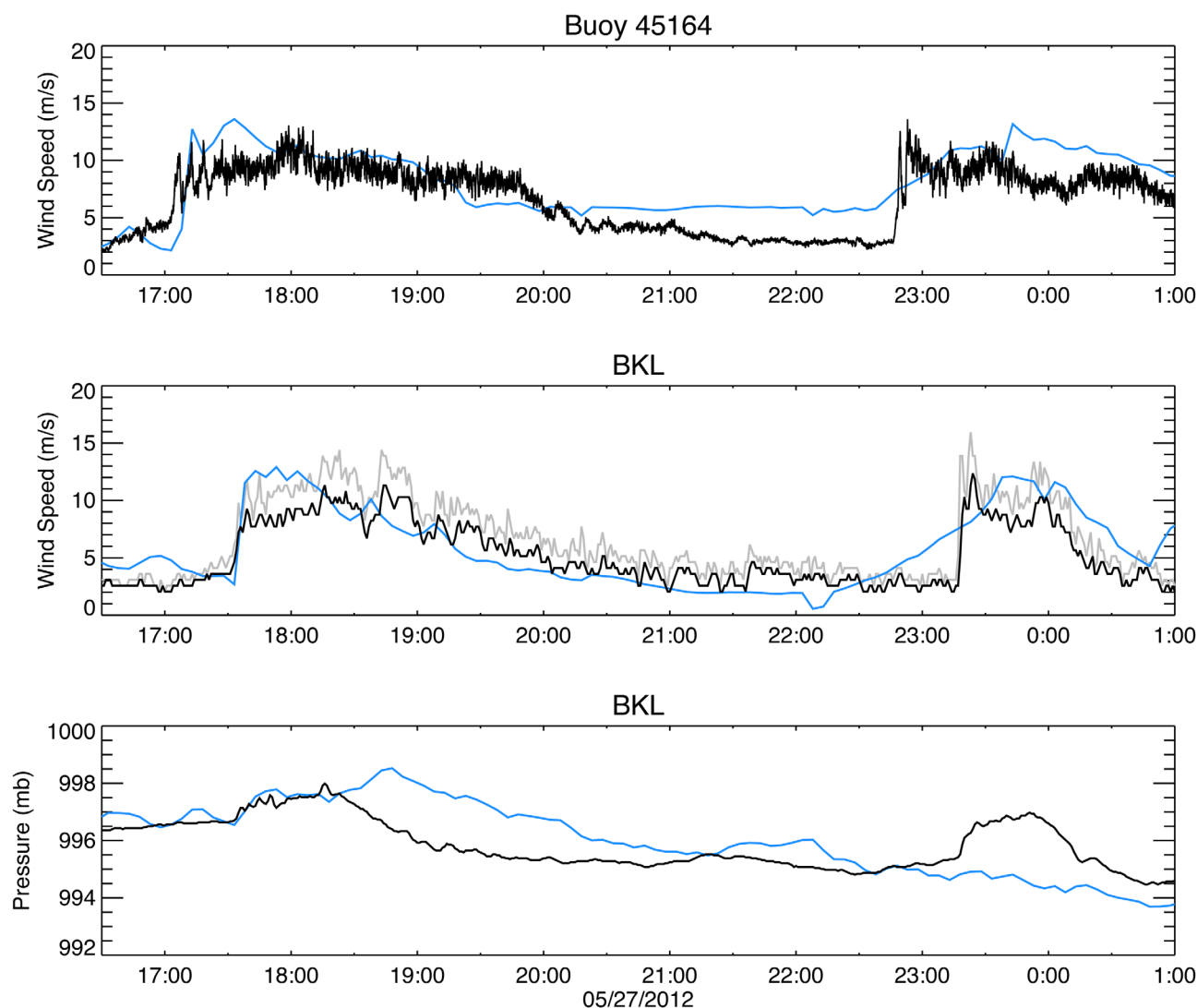
Figure 4. Observed wind speeds and barometric pressure (top) at the NDBC 45164 buoy offshore of Cleveland, OH (1 min data) and (middle and bottom) at the Burke Lakefront Airport (BKL; 2 min average). Observed station data shown in black, wind-gust shown in gray for the BKL station. Simulated 1 km WRF meteorological conditions (case ii) are shown in blue.
