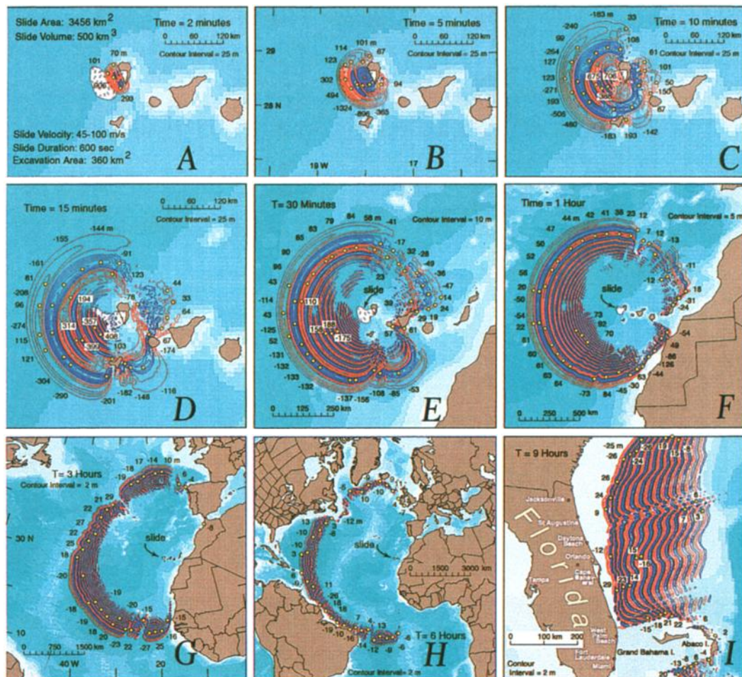
Figure 3. Evolution of the La Palma landslide tsunami from 2 minutes (a, upper left) to 9 hours (i, lower right). Red and blue contours cover elevated and depressed regions of the ocean respectively and the yellow dots and numbers sample the wave height, positive or negative, in meters. Note the strong influence of dispersion in spreading out an original impulse into a long series of waves of decreasing wavelength. See also that the peak amplitudes generally do not coincide with the first wave. Even after crossing the Atlantic, a lateral collapse of Cumbre Vieja volcano could impose a great sequence of waves of 10-25 m height on the shores of the Americas.
