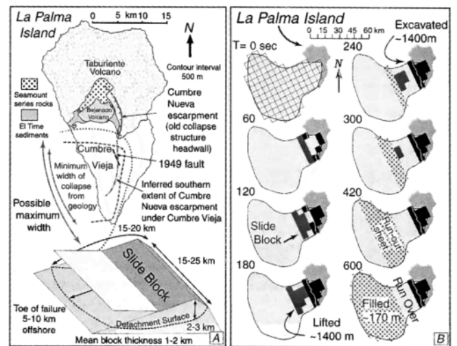
Figure 2a. Map of La Palma Island showing the major geological deposits together with the visible and inferred headscarps of the potential slide block pictured at the bottom.
