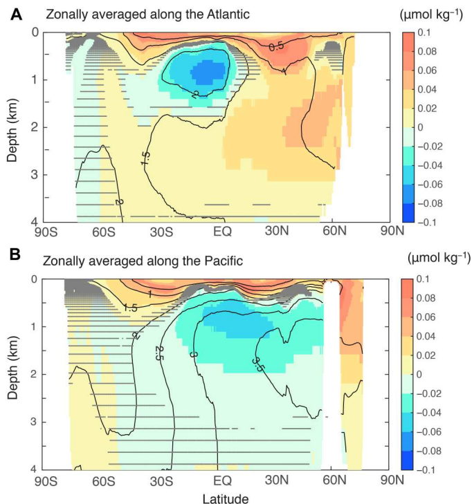
Fig. 6. Zonally averaged PO_4 difference between the variable and fixed C:P experiments, averaged over 2080–2100. The difference between the ensemble means from the variable (hyperbolic) and fixed C:P experiments is shown as shade, and the temporal mean over 2080–2100 of the variable (hyperbolic) experiment is shown as contour lines. The grid cells where the PO_4 difference does not exceed an SD across the ensemble members (indicating insignificant values with a 68% confidence interval) are marked with gray dots or stripes. (A) Zonally averaged along the Atlantic Ocean. (B) Zonally averaged along the Pacific Ocean.
