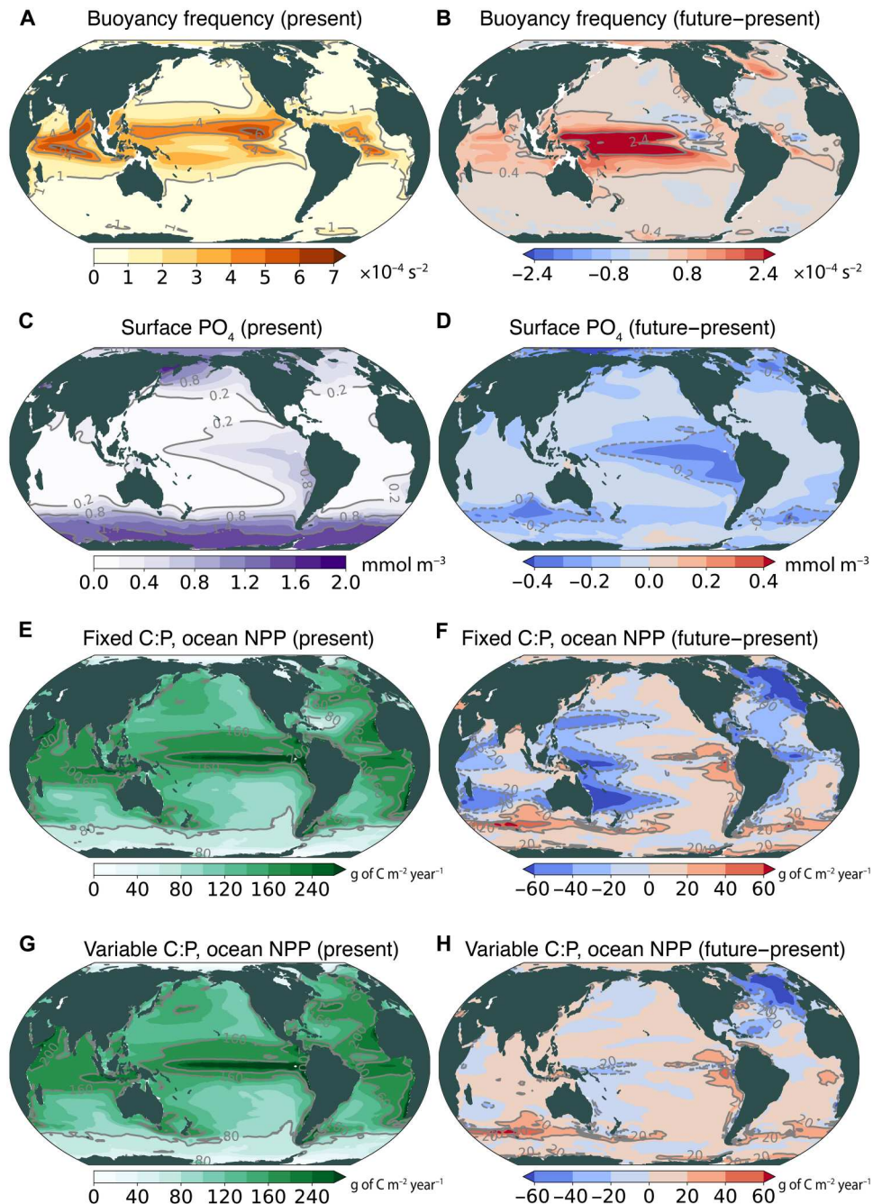
Fig. 3. Present-day means and future changes in ocean stratification, phosphate concentrations, and NPP. The panels on left column (A, C, E, G) show present-day means (1990–2010 average) and those on the right column (B, D, F, H) show future changes (2080–2100 average minus 1990–2010 average). ( A and B ) Buoyancy frequency (a measure of stratification) at 100 m. Buoyancy frequency is defined as N^2 = -g/\rho_0 \cdot (\partial\rho/\partial z) , where g is the acceleration of gravity, \rho_0 is a reference density, \rho is a local density, and z is the depth. Estimates from the fixed C:P experiment are shown. ( C and D ) Simulated surface \text{PO}_4 concentrations from the fixed C:P experiment. ( E and F ) Vertically integrated ocean NPP, simulated from the fixed C:P experiment. ( G and H ) Vertically integrated ocean NPP, simulated from the variable C:P experiment with a hyperbolic relationship between phytoplankton C:P and \text{PO}_4 concentrations.
