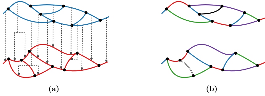
Figure 2.2: Two possible visualisations for a channel matching.
