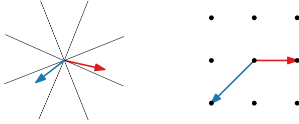
Figure 5.11: Converting a displacement vector into a directed edge.
