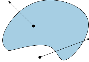
Figure 5.6: Illustration of the point-in-polygon algorithm.
