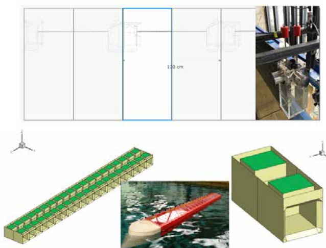
Illustration of the experimental setup of the half section of the KNSwing attenuator WEC
