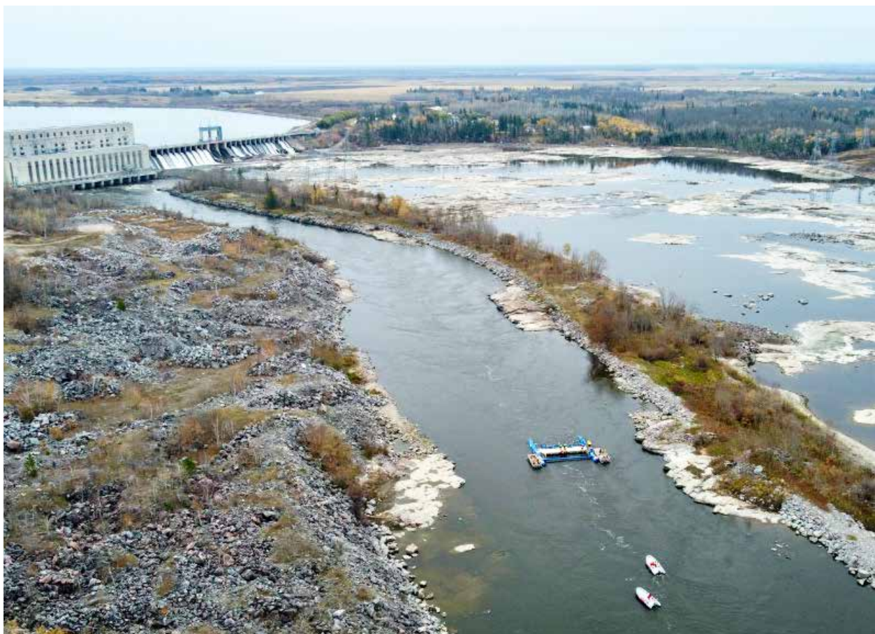
ORPC RivGen® device arriving at CHTTC project site, with Manitoba Hydro's Seven Sisters Generating Station in the background
