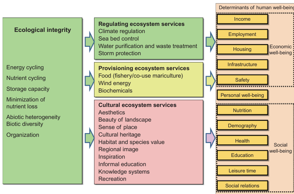
Figure 2. Marine ecosystem services potentially impacted by offshore wind farm development (direct or indirect) in the German North Sea and related determinants of human well-being. Source: Adapted from Busch et al. (2010).
