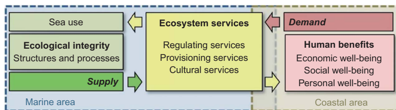
Figure 1. Conceptual model of ecosystem services in marine areas and human benefits/well-being in coastal areas (own design, Benjamin Burkhard).
