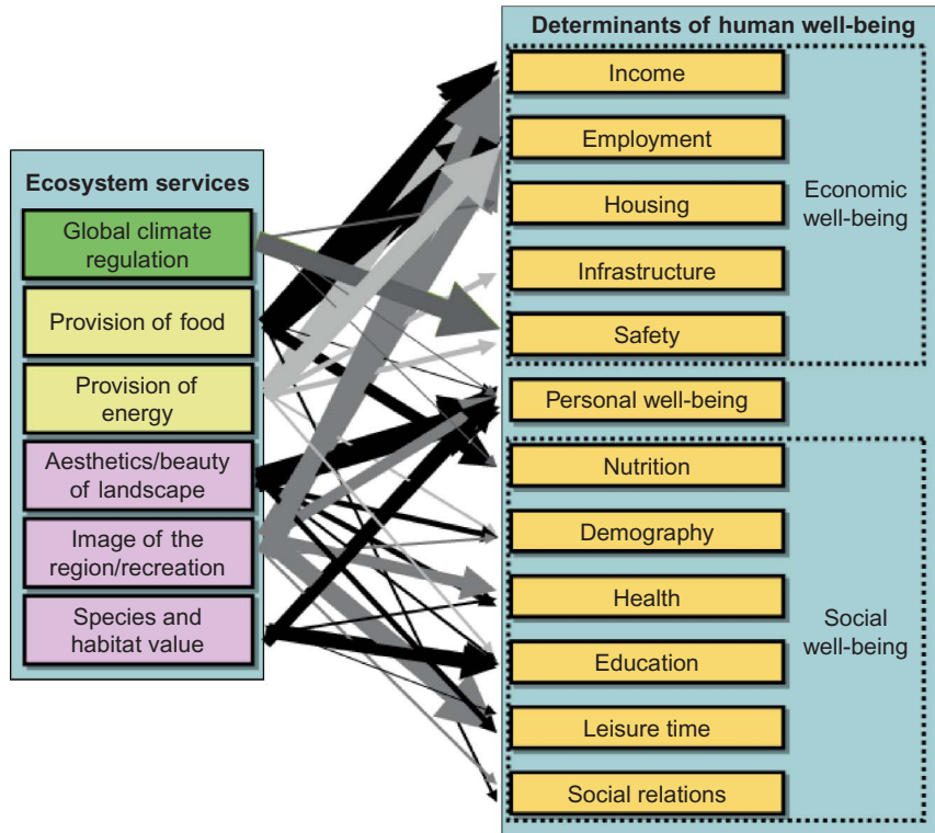
Figure 4. Identified potential linkages between ecosystem services impacted by offshore wind farming and determinants of human well-being. Source: Adapted from Busch et al. (2010).
