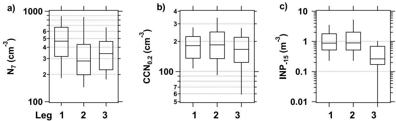
FIG. 5. Number concentrations of different particle types: (a) total particle number concentrations >7 nm ( N_7 ), (b) CCN_{0.2} , and (c) INP_{-15} at -15^\circ\text{C} for each leg. The box-and-whisker plots show the median, interquartile range, and 10th and 90th percentiles.
