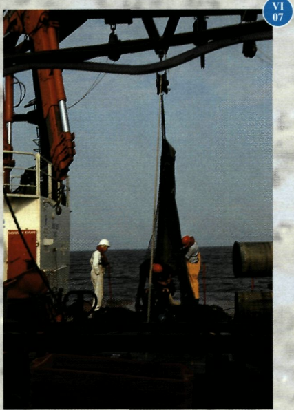
Part of a catch achieved after one night trawling over the bottom at 5000 m depth in the NE Atlantic.
