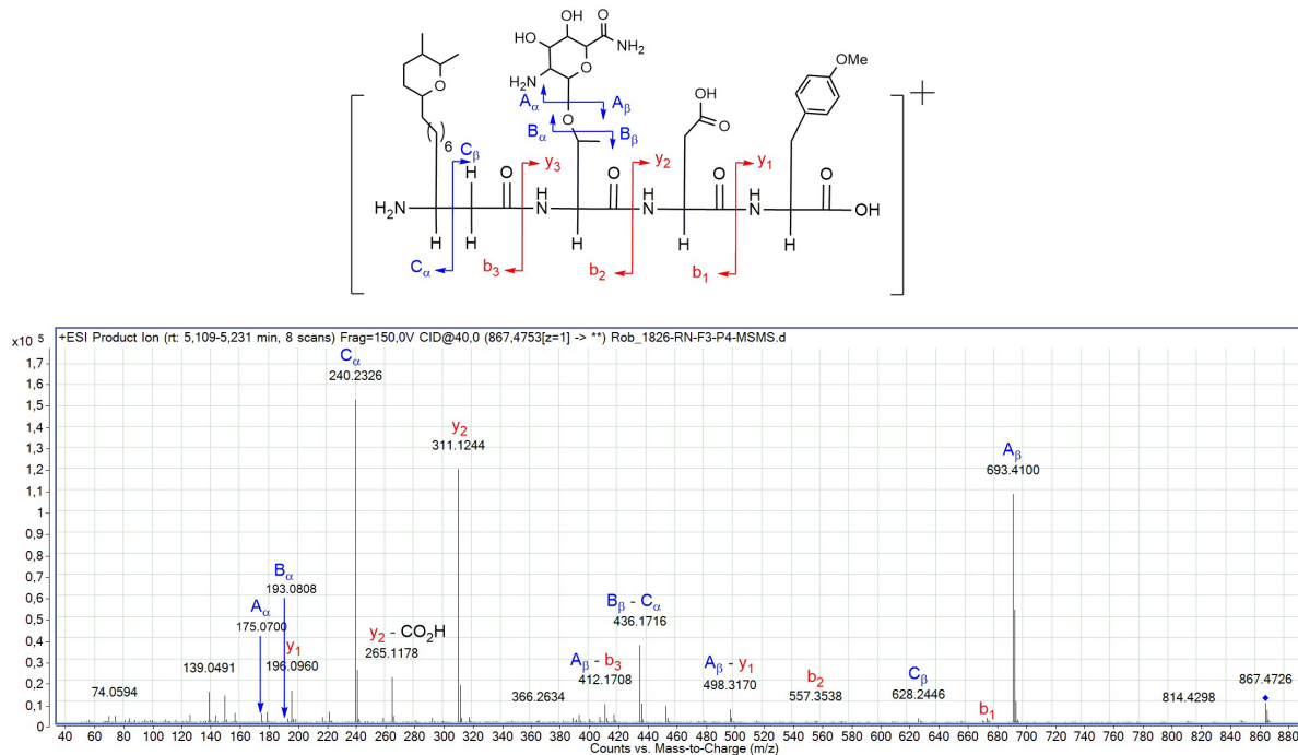
Figure 2. MS/MS analysis and fragmentation pattern of 1 and 2.
