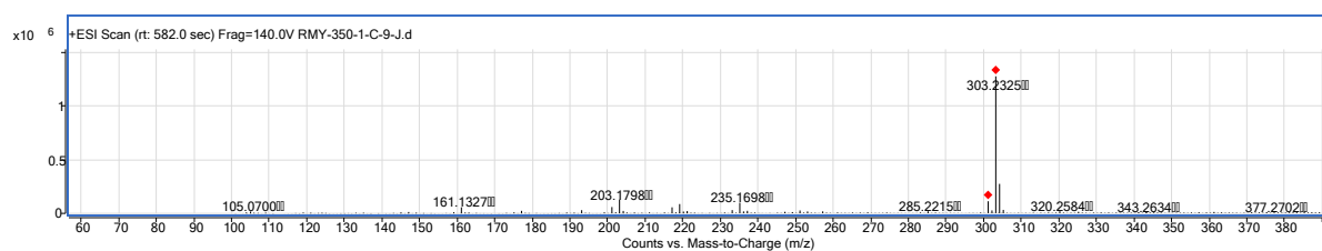
Figure S38: HRESIMS spectrum acalycigorgin E (6).
