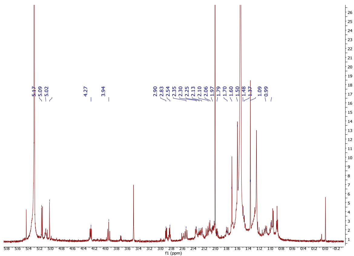
Figure S32: ^1\text{H} NMR spectrum of acalcixeniolide F ( 4 ) in \text{CDCl}_3 (600 MHz).
