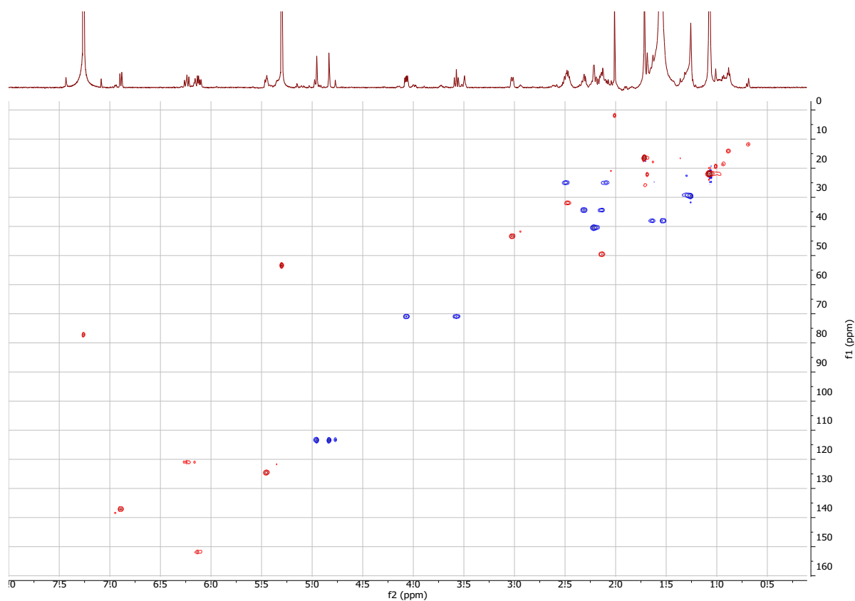
Figure S37: gHSQC NMR spectrum coraxeniolide C (5) of in CDCl 3 (600 MHz).
