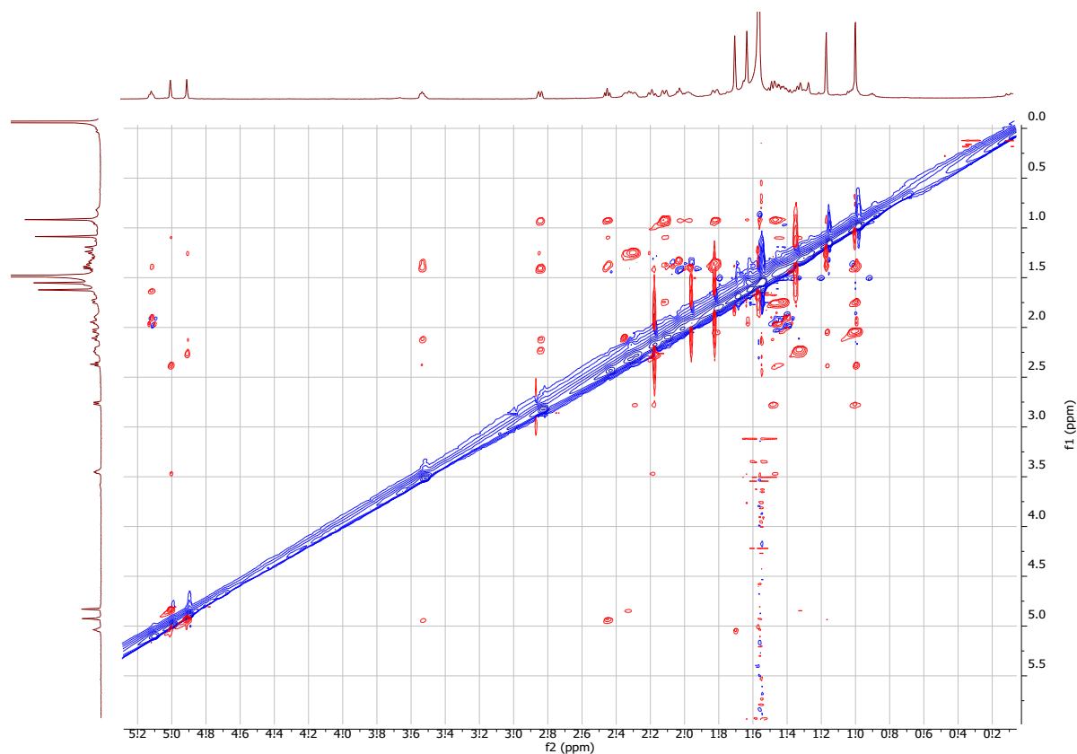
Figure S23: ROESY NMR spectrum of epoxymienol ( 2 ) in CDCl 3 (600 MHz).
