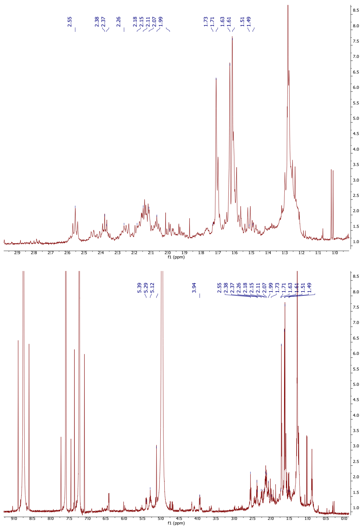
Figure S11: ^1\text{H} NMR spectrum of mienolol (1) in \text{C}_5\text{D}_5\text{N} (600 MHz).
