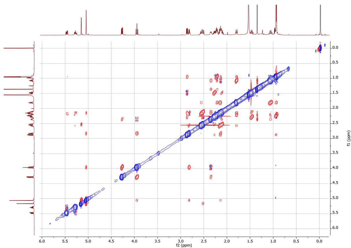
Figure S30: ROESY NMR spectrum of epoxycoraxeniolide A ( 3 ) in CDCl 3 (600 MHz).
