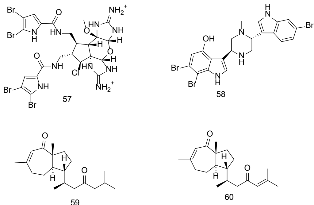
Figure 14. Secondary metabolites isolated from deep-sea sponges of the order Axinellida.
