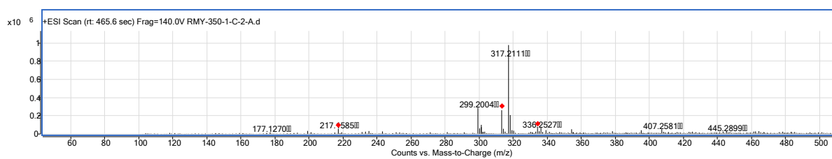
Figure S44: HRESIMS spectrum of 9-deoxyxenilide A ( 8 ).
