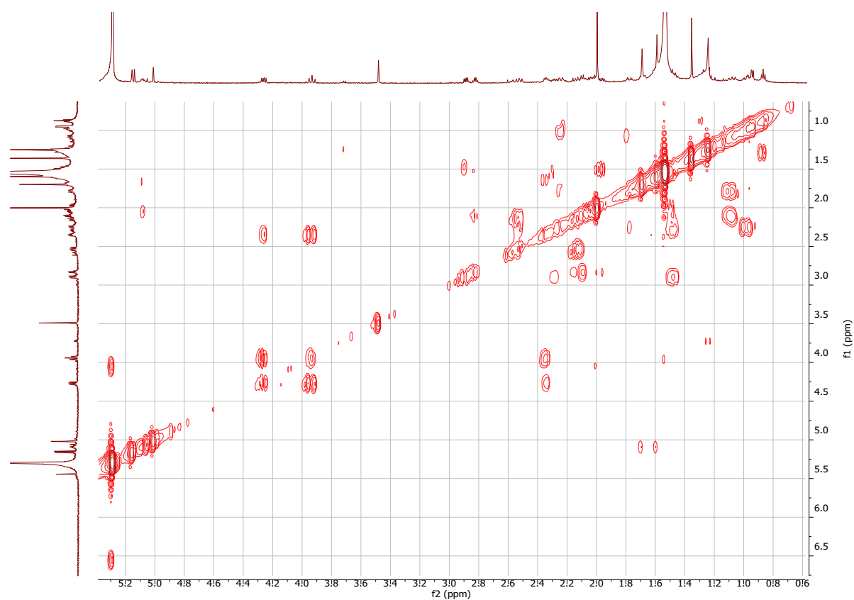
Figure S33: gCOSY NMR spectrum of acalcixeniolide F ( 4 ) in \text{CDCl}_3 (600 MHz).
