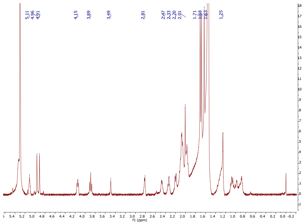
Figure S39: 1 H NMR spectrum acalycigorgin E (6) of in CDCl 3 (600 MHz).
