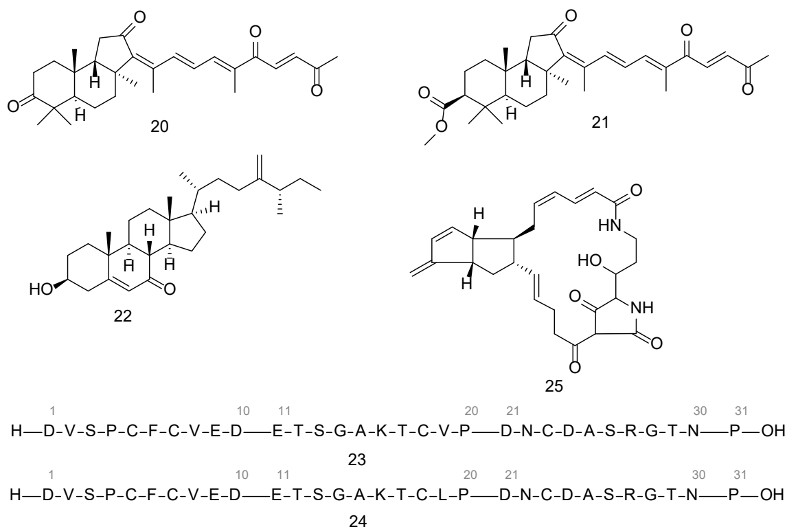
Figure 8. Chemical structures of metabolites isolated from deep-sea sponges of the order Tetractinellida.
