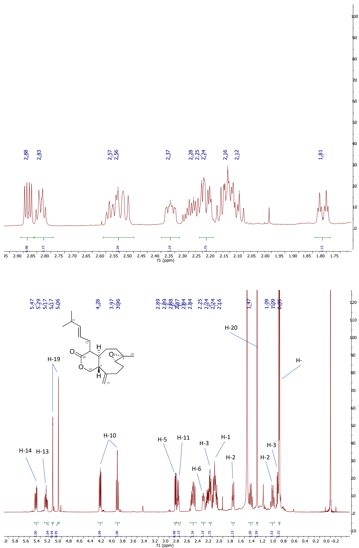
Figure S25: ^1\text{H} NMR spectrum of epoxycoraxeniolide A ( 3 ) in \text{CDCl}_3 (600 MHz).
