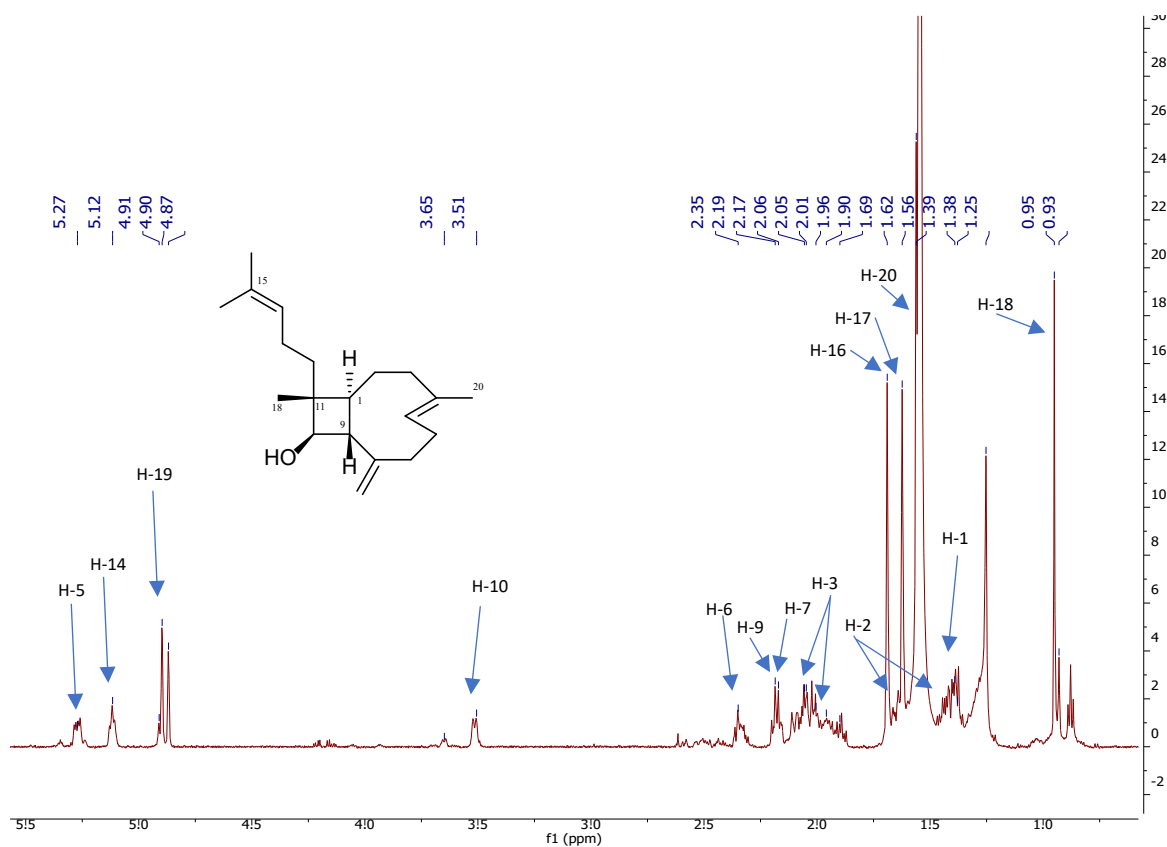
Figure S5: ^1\text{H} NMR spectrum of miolenol (1) in \text{CDCl}_3 (600 MHz).
