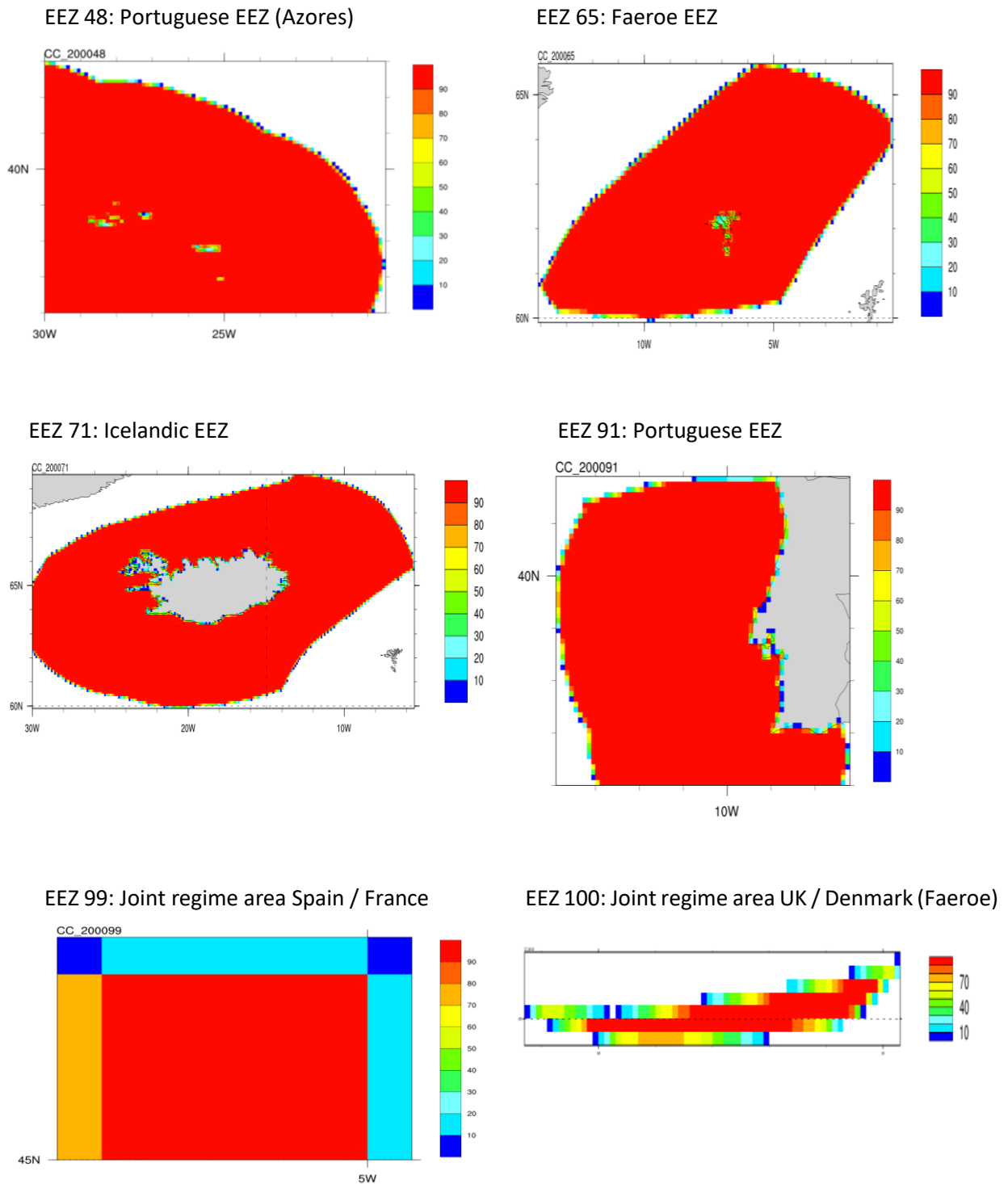
Figure 5: Visualization of EEZs in the EMEP grid. The plots show how large a percentage of each EMEP model grid cell lies within the respective EEZ. EMEP model grid cells cover 0.1^\circ\text{lon} \times 0.1^\circ\text{lat} pixels and thus appear very small in some of the plots. Red colour means that the model grid cell is fully within the EEZ. Other colours mean that the grid cell is only partly within the EEZ. Some EEZs are not fully covered by the EMEP model domain, e.g. EEZ 48 (PT/Azores) is cut at 30^\circ\text{W} , which is the western boundary of the EMEP model domain. Parts of EEZs outside the OSPAR regions are not included in the plots (and the analysis). The figure continues on the next 3 pages.
