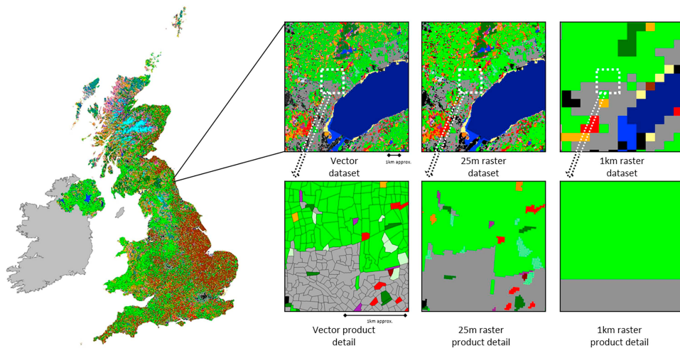
Figure 2.4 The UKCEH land cover map, 2020 (left), showing different levels of detail (right).
