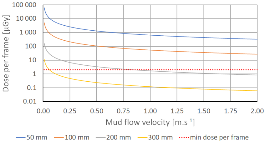
Figure 3.10: Radiation dose, originating from an X-ray 225 kV - 30 mA generator at max power, received by the detector in a setup as shown in Fig. 3.1 (A)) during the time span allowed for per image frame. The time span is expressed as mud flow velocity, where a maximum mud particle displacement of 5 mm is allowed for between two consecutive frames. Increasing mud flow velocity decreases the radiation time span for each image frame, hence the dose received per image frame. Curves for different mud layer thicknesses varying from 50 mm to 300 mm are presented. The dotted red line indicates the minimum dose required per image frame for diagnostic image quality.
