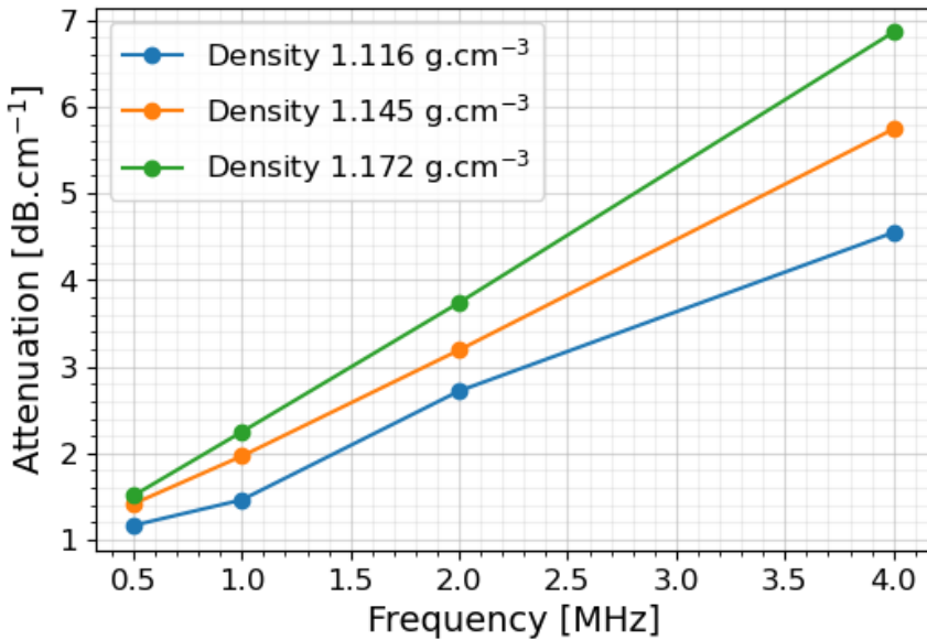
Figure 4.10: Values of attenuation deduced from the measurements with the AQUAscatt 1000R. The values of attenuation correspond to half the slope of the trendlines fitting the recordings (see Fig. 4.9).
