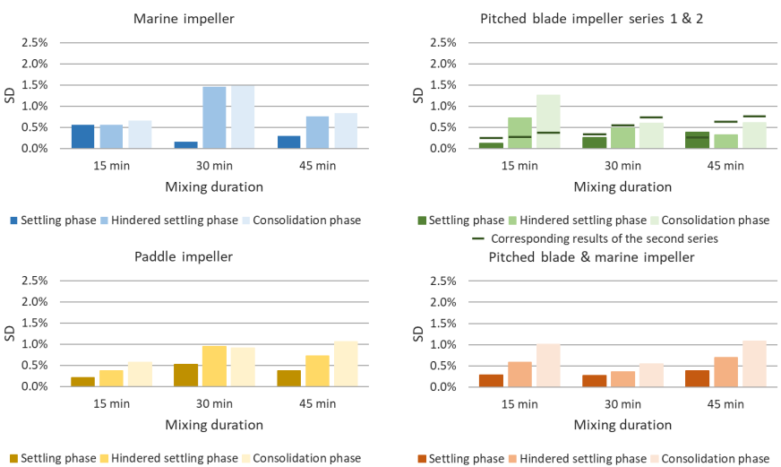
Figure 2.10: Standard deviations (SD) of the settling curves averaged per series of three repetition experiments (see Section 2.4.2 and Table 2.1), sorted per mixing technique. The chart of the pitched blade impeller shows the results of both series performed with the pitched blade impeller (see Section 2.4.2). The results of the first series are presented with the bar charts. The results of the second series with the dark green lines aligned with the corresponding bar chart. For each mixing technique, a breakdown of the applied mixing duration and phases of settlement is provided.
