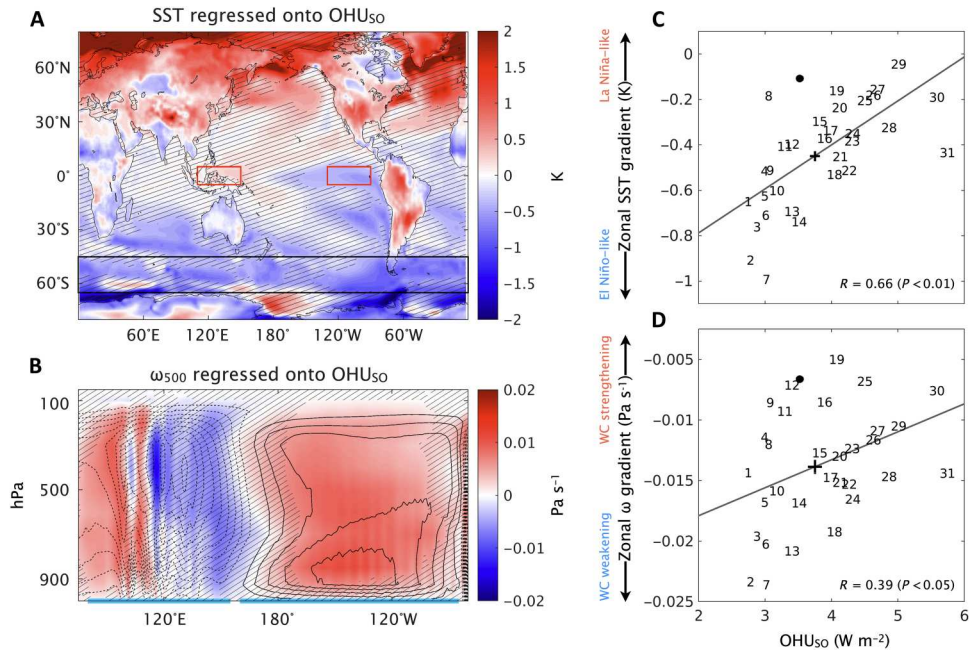
Fig. 4. CMIP6 inter-model regression. (A) Global mean removed SST response and (B) equatorial Pacific pressure velocity response, regressed onto Q_{net} changes averaged between 45°S and 65°S ( OHU_{50} ) for 31 CMIP6 abrupt-4xCO 2 simulations (model lists in table S1). The regression coefficients are multiplied by two inter-model SDs of Q_{net} changes to represent the inter-model discrepancies. The regions with the response insignificant at 95% confidence level based on the two-sided t test are hatched. Scatterplot of OHU_{50} against (C) the equatorial Pacific zonal SST gradient and (D) the Walker circulation index. Models are numbered in the ascending order of the amplitude of Southern Ocean heat uptake. The plus symbol indicates the CMIP6 MMM and the black closed circle indicates our FULL response. The comparison is made by simply halving the CMIP6 responses between 21 and 70 years after an abruptly quadrupled CO 2 as our FULL experiment is forced by a CO 2 doubling.
