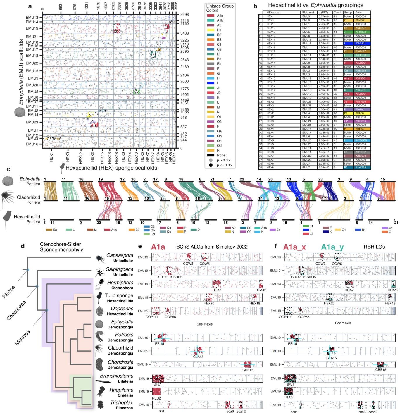
Extended Data Fig. 3 | Sponge macrosyteny. a-c. There have been many genome rearrangements since the divergence of the demosponge Ephydatia and the tulip hexactinellid genome, and they share macrosyteny of only some BCnS linkage groups ( p \leq 0.05 , Bonferroni-corrected one-sided Fisher's exact test 57 , opaque dots in a. , rows in b. , interspecies lines in c. ). d. The sponge cladogram is based on Schuster et al. 2018 38 . e. The orthologs in A1a_x and A1a_y are predominantly present on separate chromosomes in both the tulip hexactinellid and in Oopsacas minuta . f. A1a_x and A1a_y are on partly
