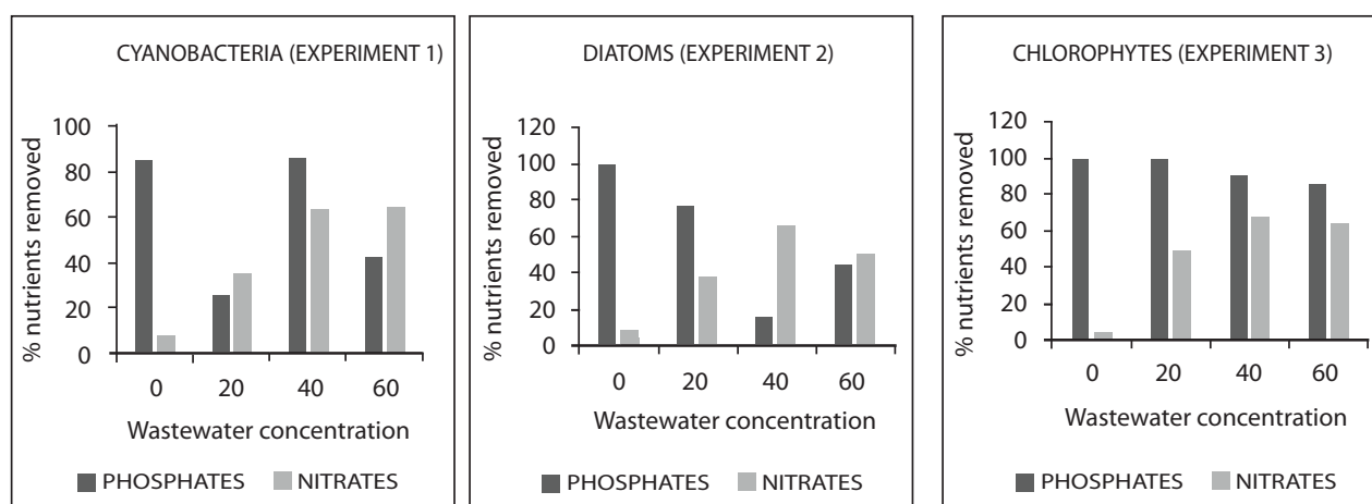
Figure 3. The percentage of nutrients ( \text{PO}_4^{3-} and \text{NO}_3^- ) removed from the wastewater cultures.
