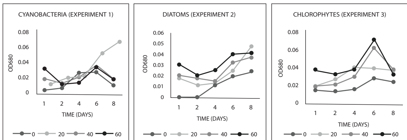
Figure 4. Microalgae growth in the different batch experiments using optical density (OD680) for the culturing period.
