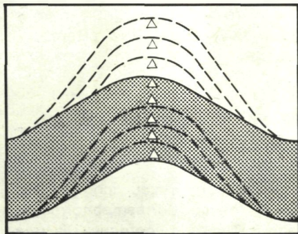
Schema meandervorming
