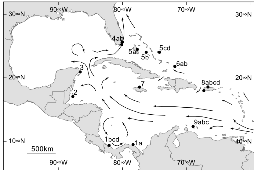
Figure 1. Collection localities from 9 regions in the Caribbean, and Bahamas, and Florida with the major surface currents (Wust 1964). (1) Panama—a. San Blas, b. Salt Creek, c. Crawl Cay, and d. Casa Blanca (Bocas del Toro); (2) Belize; (3) Yucatan; (4) Florida—a. Florida Keys, b. Fort Lauderdale; (5) Bahamas—a. Andros Island, b. Lee Stocking Island, c. North San Salvador Island, and d. Southwest San Salvador Island; (6) South Caicos, Turks and Caicos—a. Montastraea Reef, b. Patch Reef; (7) Discovery Bay, Jamaica; (8) Puerto Rico—a. San Juan, b. San Cristobal, c. Media Luna, d. Guanica; (9) Curacao—a. Jan Thiel, b. Fuik, c. Spaanse Water.
