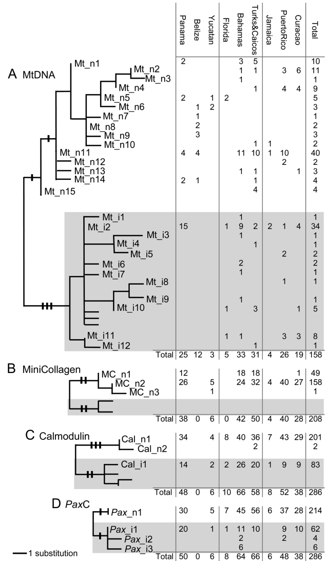
Figure 2. ML trees for (A) mitochondrial control region (Mt), (B) MiniCollagen (MC), (C) Calmodulin (Cal), and (D) PaxC ( Pax ) showing the geographic distribution of alleles across 9 regions in the Caribbean, Bahamas, and Florida. Native alleles are in white and introgressed alleles are highlighted in gray (from Vollmer SV, Palumbi SR, in preparation). Alleles found in Acropora cervicornis are labeled and coded with a gene abbreviation (e.g., MiniCollagen as MC) and a code for whether it was native (n) or introgressed (i). Unlabeled branch tips represent alleles that were observed in Acropora palmata or hybrid A. prolifera , but not Acropora cervicornis . Tick marks along major branches indicate substitutions. (A) MtDNA ML tree constructed using a general time reversible + \Gamma + I model (1 of 6 trees, ln score = 1537.7). (B) MiniCollagen ML tree constructed using a Jukes-Cantor model (ln score = 575.7). (C) Calmodulin ML tree constructed using a GTR model (ln score = 477.9). (D) PaxC ML tree constructed using an F81 model (ln score = 733.7). Sequences are available on GenBank.
