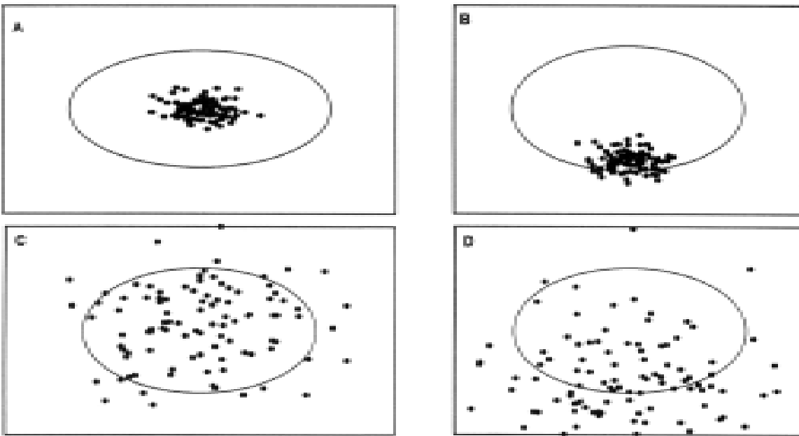
Figure 1. Shot patterns on targets demonstrating (A) precise and accurate (non-biased) shots, (B) precise but inaccurate shots, (C) imprecise but accurate shots, and (D) imprecise and inaccurate shots. (Source: White et al., 1982).
