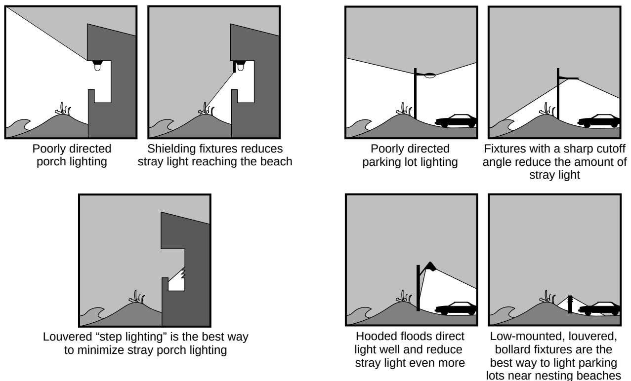
Figure 1. Light management techniques for building and pole-mounted lighting near sea turtle nesting beaches.
