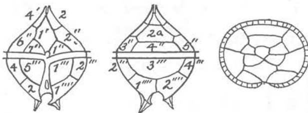
Fig. 122. P. pallidum Ostenfeld. Ventral, dorsal and apical views. X 350.
