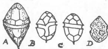
Fig. 90. P. triqueta (Stein). A, X 600; B and C, X 500; D, spore X 500.
