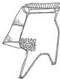
Fig. 63. Dinophysis tripos Gouret X 300.
