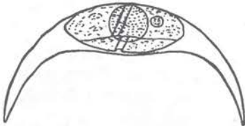
Fig. 44. G. bicornis K. & S. Cyst containing fully developed cell. X 400.
