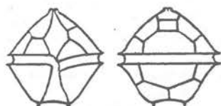
Fig. 120. P. brevipes Paulsen X 500.
