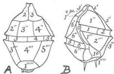
Fig. 74. Arrangement and numbering of the plates in the genus Gonyaulax ; A, G. polygramma dorsal view; B, G. spinifera ventral view. After Kofoid.
