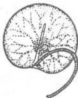
Fig. 34. Noctiluca scintillans (Macartney) X 75.
