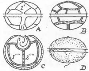
Fig. 83. P. asymmetrica Mangin. A, ventral; B, dorsal; C, antapical view; D, dorsal view of living specimen. X 300.
