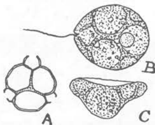
Fig. 24. Ebria tripartita (Schum.) A, skeleton X 450; B, and C dorsal and side view of living cell X 600.
