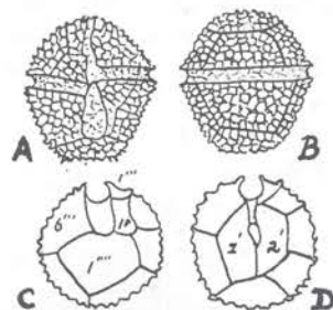
Fig. 73. Protoceratium reticulatum C. & L. A, ventral; B, dorsal; C, antapical; D, apical views. X 400.
