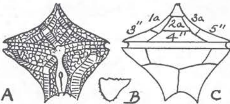
Fig. 115. P. crassipes Kofoed. A, ventral; B, side view of antapical spine; C, dorsal view. X 350.
