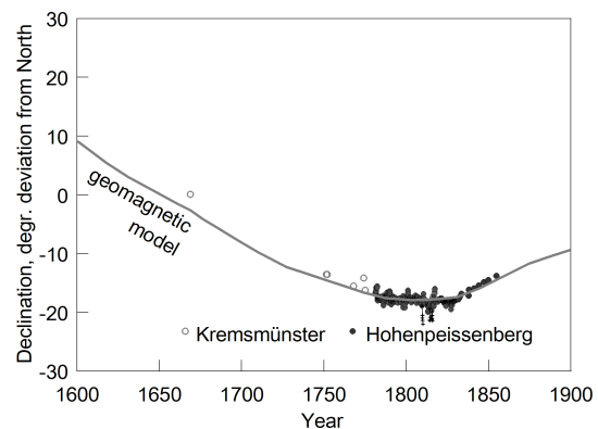
Figure 11. Secular variation of the magnetic declination (model and observations) adapted from Korte et al. (2009). Crosses mark unreliable measurements, because the declinometer deviated from the northern direction.
