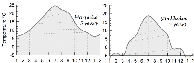
Figure 10. Average yearly cycles of temperature at Marseille and Stockholm according to Schön (1818). The y scales, missing in the original, have been supplemented and harmonized, and the units have been changed to °C. Schön connected months with the same solar elevation by inclined lines, in order to visualize the asymmetry of the yearly course of the temperature in relation to the sun's elevation.
