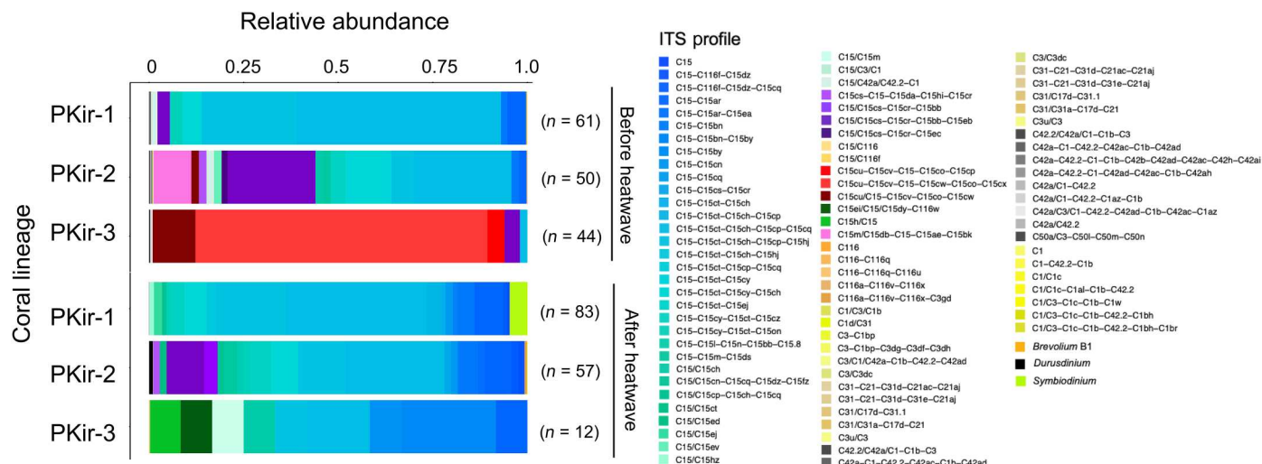
Fig. 4. The relative abundances of ITS2 profiles across all colonies of each lineage before and after the heatwave. Sample sizes indicate the number of colonies. Only samples with >500 sequence reads were included.
