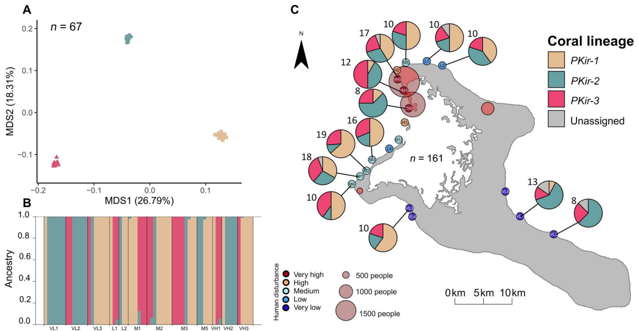
Fig. 1. Cryptic lineages of massive Porites across foreereef sites on Kiritimati. (A) Principal coordinate analysis (PCoA) of 2b-RAD data (using 1-Pearson correlation matrices through ANGSD) showing three population clusters. (B) Results of ADMIXTURE analysis showing the assignment of colonies to one of three lineages, arranged by collection site. (C) Map with pie charts showing the relative abundance of each lineage at each site before the heatwave. Numbers indicate the number of colonies sampled and sequenced with either 2b-RAD or ITS2 metabarcoding. Circles labelled with site names represent sites colored by level of human disturbance. Semi-transparent red circles indicate the location of villages, scaled by human population size.
