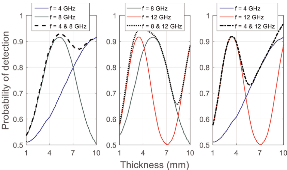
Figure 4. Comparison between the probability of detection and the oil thickness (in mm) for different detector algorithms: Single-frequency detectors at 4 GHz, 8 GHz, and 12 GHz, and dual-frequency detectors using combinations of these frequencies.
