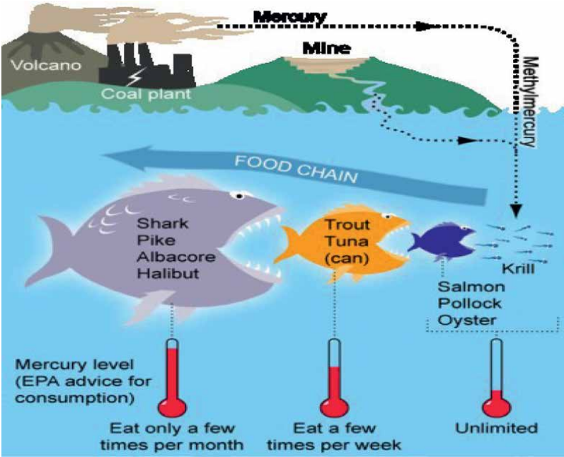
Figure 5. Methyl mercury concentrations within the fishes.
