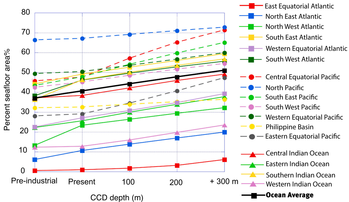
Fig. 4. The changes in percent area of ocean exposed to corrosive bottom waters in 17 different ocean regions in pre-industrial times (–100 m), at present and resulting from a hypothetical shoaling of the CCD in three, 100 m increments. The slope of lines gives a relative indication of change in area below the CCD with CCD shoaling. Estimated error (not shown) for present CCD is as per Table 1.
