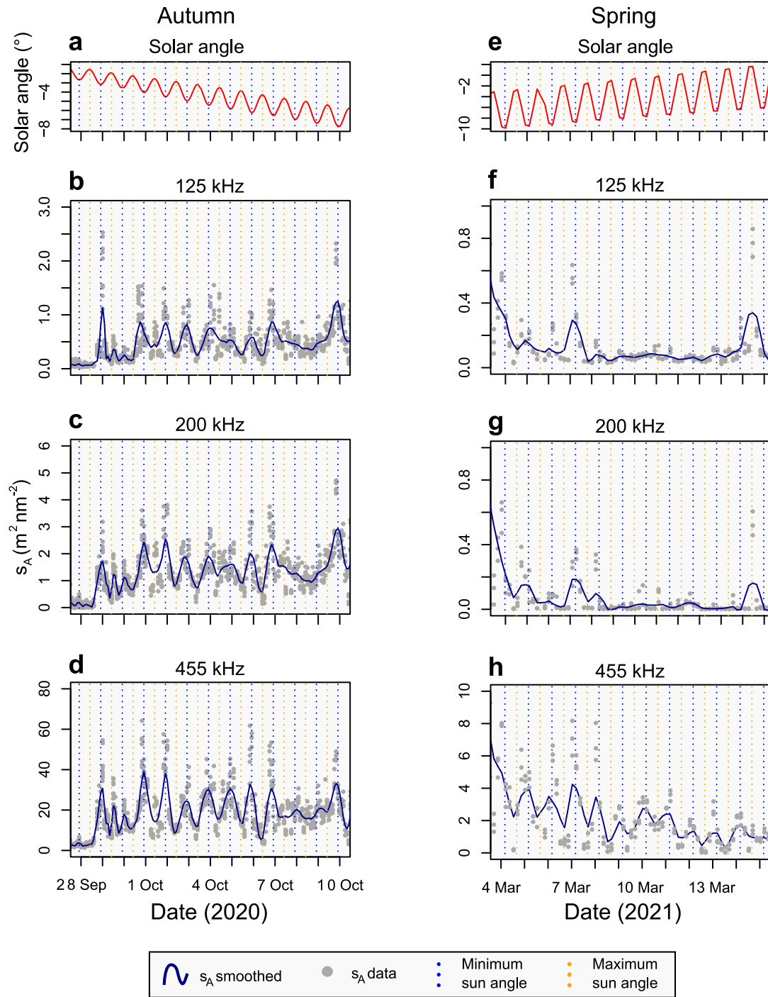
Extended Data Fig. 2 | Diel variability of depth-integrated backscatter during the autumn and spring twilight periods. Solar angle and nautical area scattering coefficient ( s_A , m^2 nmi^{-2} ) at 125, 200 and 455 kHz above the surface
