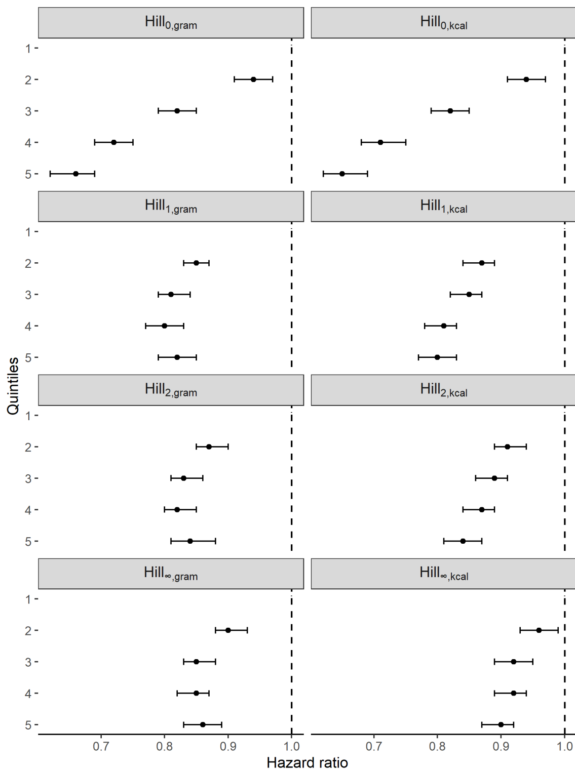
Figure A7: Hazard ratios for the Hill numbers using the overall mortality dataset (n=451,390).
