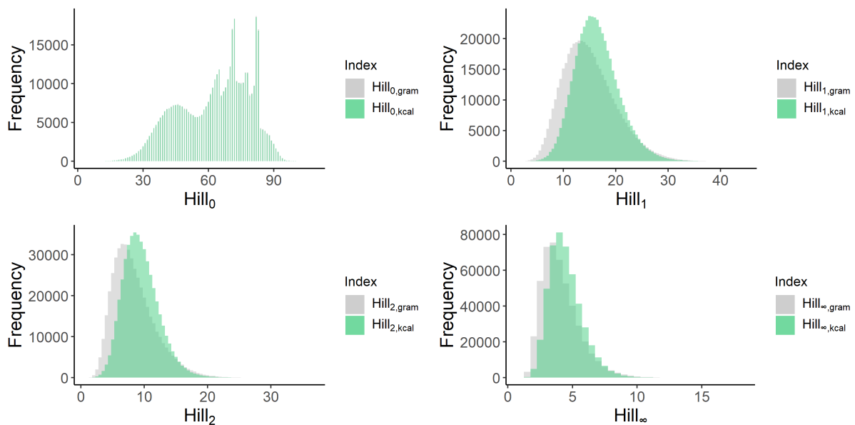
Figure 4.1: Overview of the distribution of the weight- and energy-based indices using the full dataset ( n=476,768 ). The graphs of Hill_{0,gram} and Hill_{0,kcal} coincide.
