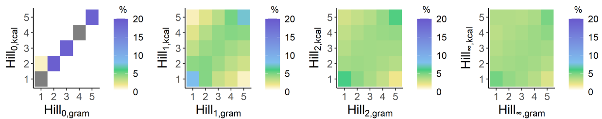
Figure 4.11: Energy-based compared to weight-based Hill numbers, represented by quintiles using the full dataset ( n=476,768 ). The colour code represents the percentage of the whole cohort classified in a given quintile for the index on the x-axis and a given quintile for the index on the y-axis.
