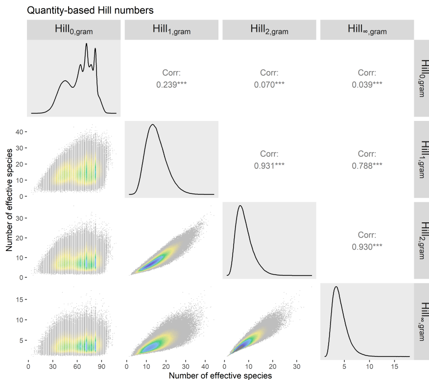
Figure 4.4: Relationships between weight-based Hill numbers and Pearson correlation coefficient (Corr) using the full dataset (n=476,768).
