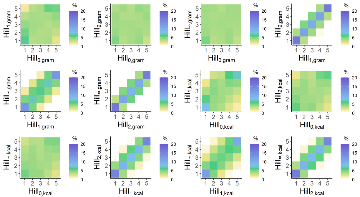
Figure 4.6: Comparative analysis of quintile divisions for different indices using the full dataset ( n=476,768 ). The colour code represents the percentage of the whole cohort classified in a given quintile for the index on the x-axis and a given quintile for the index on the y-axis.
