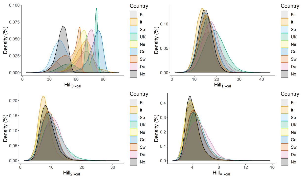
Figure 4.3: Association between energy-based indices and respondent's country of residence using the full dataset (n=476,768). Fr: France, It: Italy, Sp: Spain, UK: United Kingdom, Ne: The Netherlands, Ge: Germany, Sw: Sweden, De: Denmark and No: Norway.
