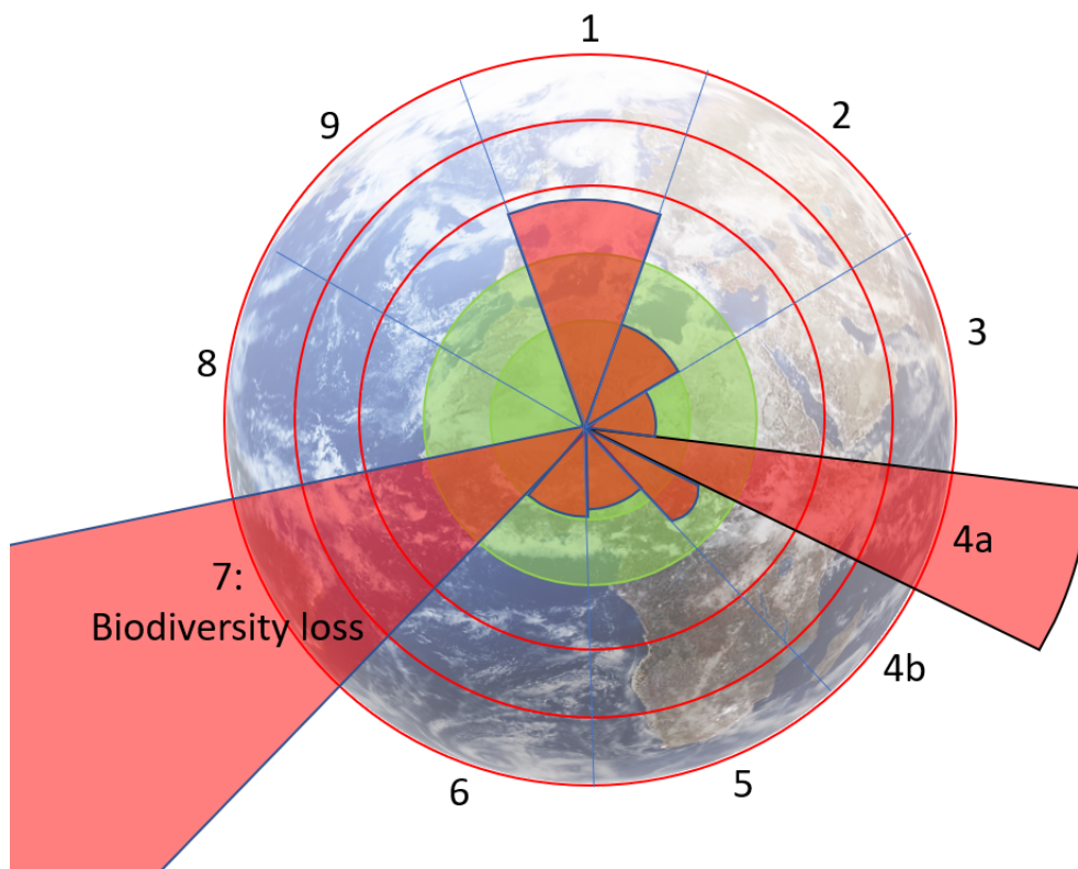
Figure 1.1: The nine planetary boundaries defined by Rockström et al. (2009), indicating biodiversity loss is occurring at an alarming rate. 1: climate change, 2: ocean acidification, 3: stratospheric ozone depletion, 4a: nitrogen cycle, 4b: phosphorus cycle, 5: freshwater use, 6: change in land use, 7: biodiversity loss, 8: atmospheric aerosol loading (not yet quantified) and 9: chemical pollution (not yet quantified). Adapted from Rockström et al. (2009).
