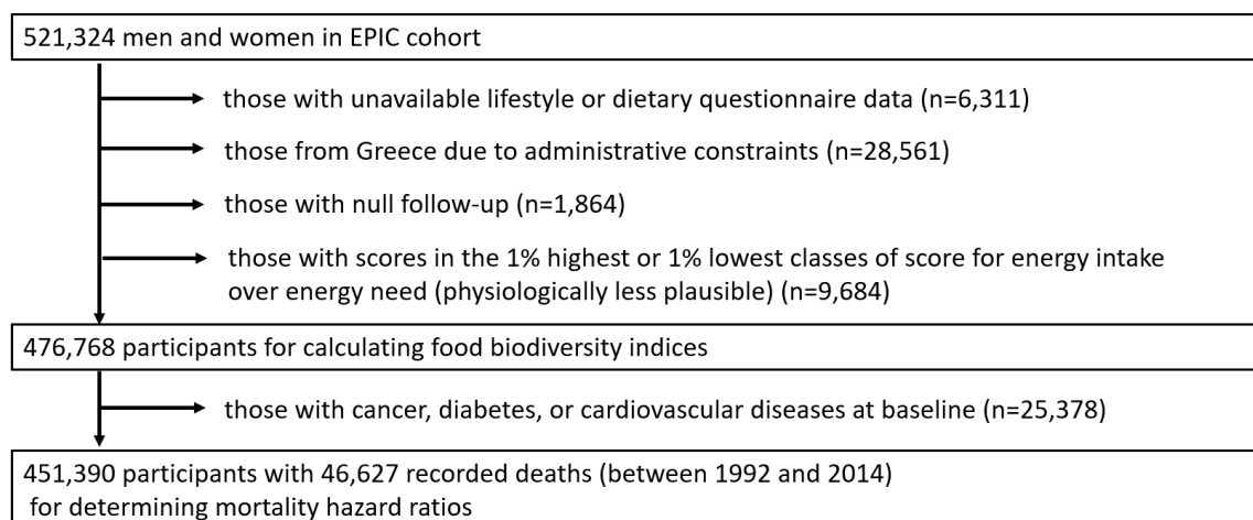
Figure 3.1: Flowchart of exclusion of the data obtained from the EPIC study.
