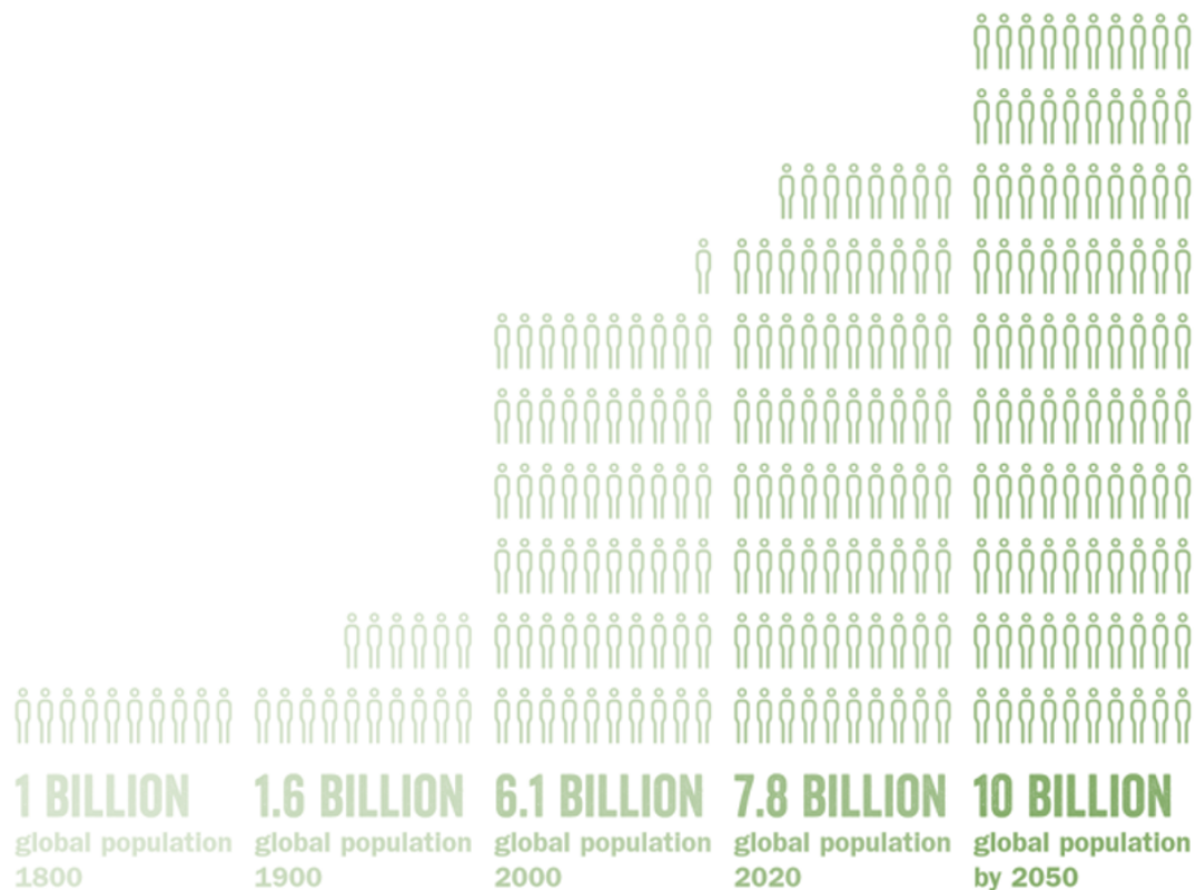
Figure 2.3: The trend of the exponentially growing world population. From Antonelli et al. (2020).
