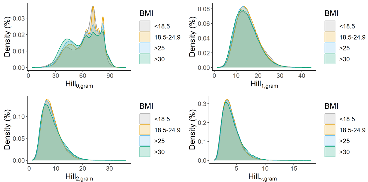
Figure A5: Association between weight-based indices and body mass index (BMI) using the full dataset (n=476,768).
