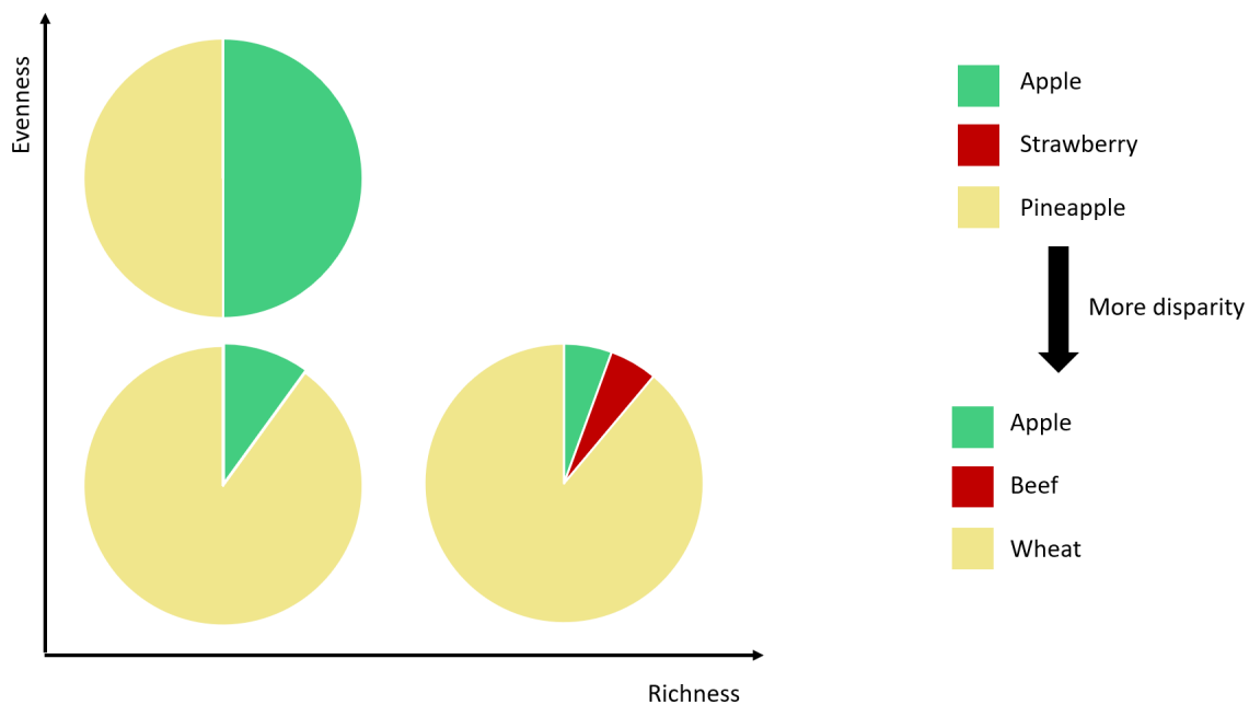
Figure 2.4: Three components of food biodiversity: richness, evenness, and disparity.
