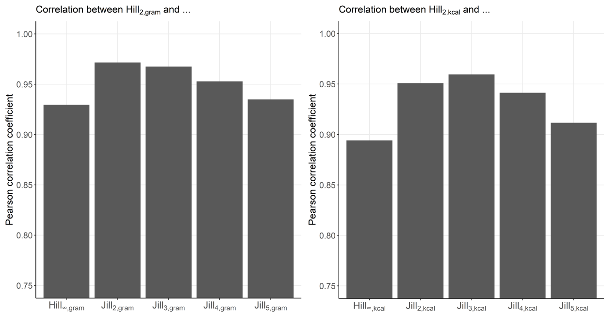
Figure 4.10: Pearson correlation coefficients between Hill_2 and Hill_\infty (reference) and between Hill_2 and a newly created index Jill_x using the full dataset ( n=476,768 ).
