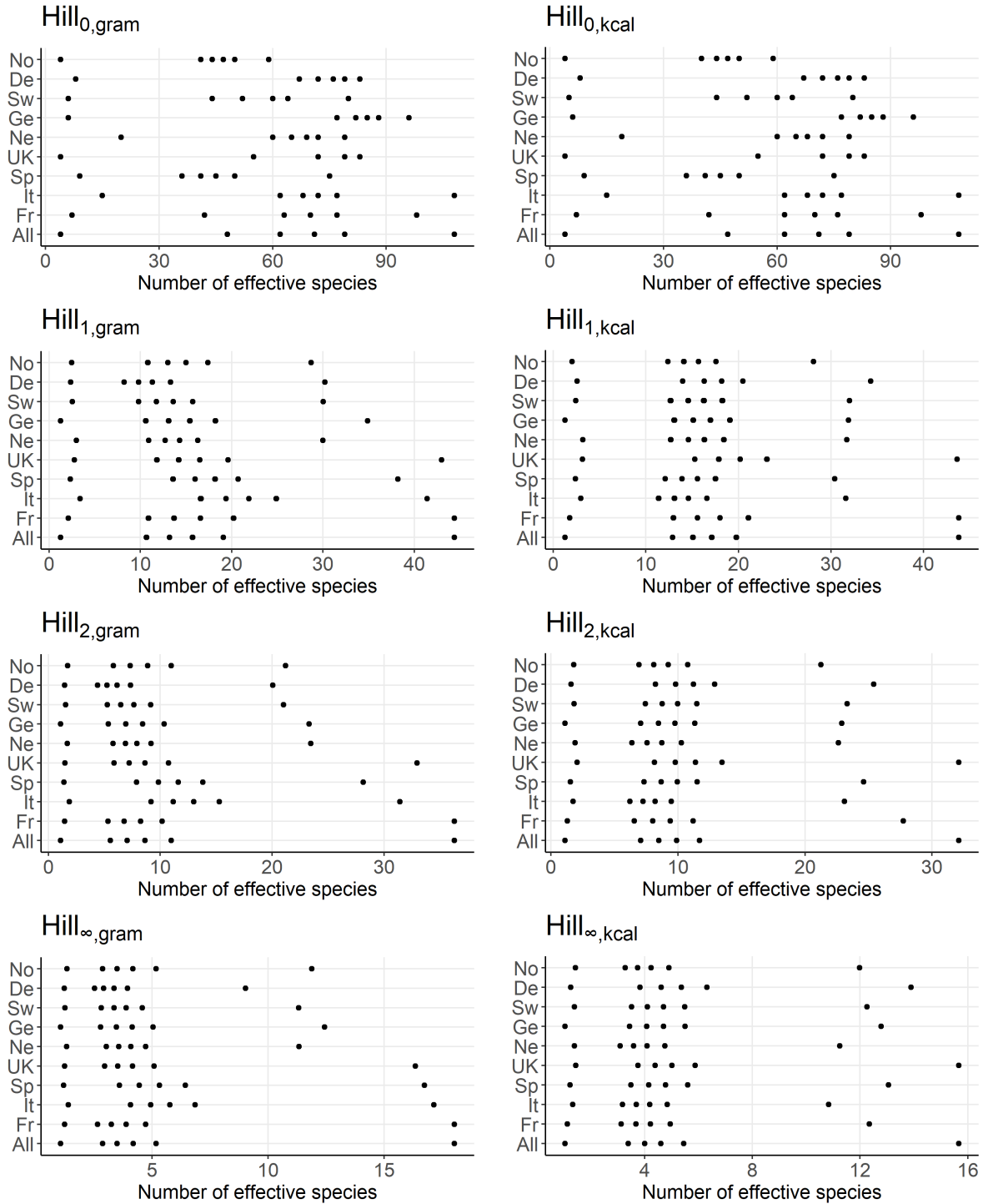
Figure 4.7: Boundaries of the quintiles per index and per country using the full dataset (n=476,768). Fr: France, It: Italy, Sp: Spain, UK: United Kingdom, Ne: The Netherlands, Ge: Germany, Sw: Sweden, De: Denmark and No: Norway.
