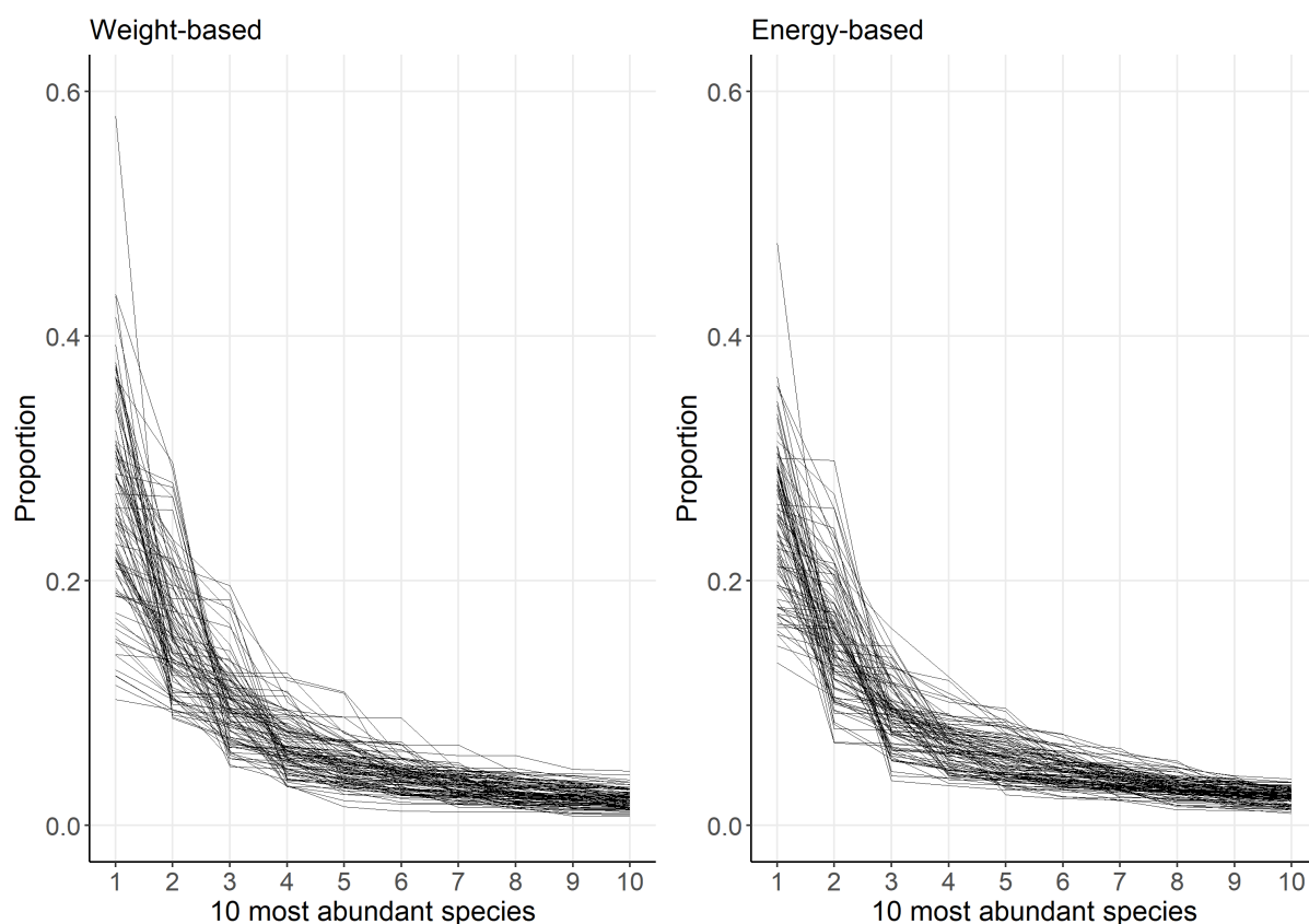
Figure 4.9: Abundance of the ten most abundant species per person using the test dataset ( n=93 ).
