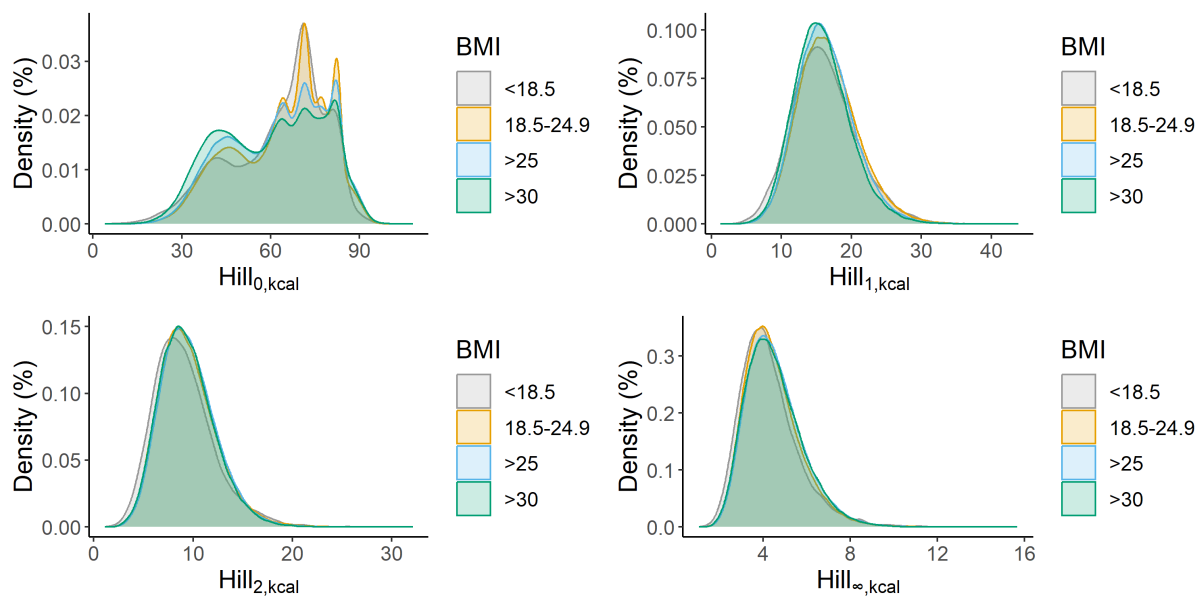
Figure A6: Association between energy-based indices and body mass index (BMI) using the full dataset (n=476,768).
