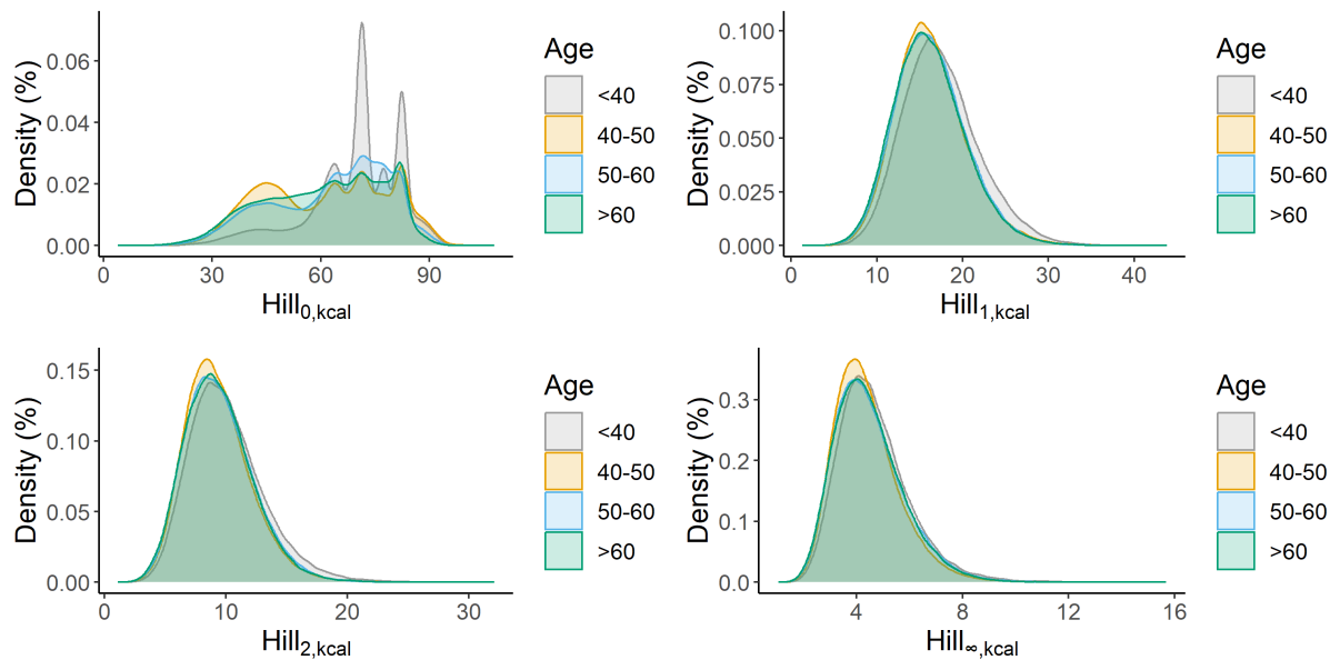
Figure A4: Association between energy-based indices and age at recruitment using the full dataset (n=476,768).
