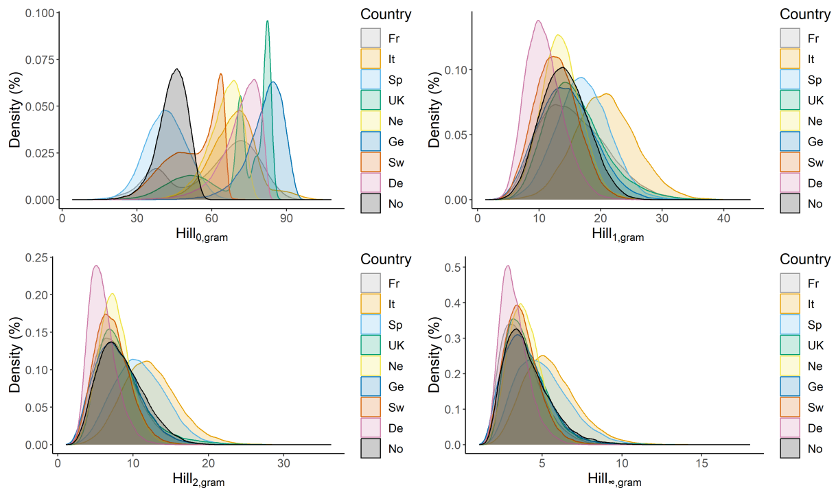
Figure 4.2: Association between weight-based indices and respondent's country of residence using the full dataset (n=476,768). Fr: France, It: Italy, Sp: Spain, UK: United Kingdom, Ne: The Netherlands, Ge: Germany, Sw: Sweden, De: Denmark and No: Norway.
