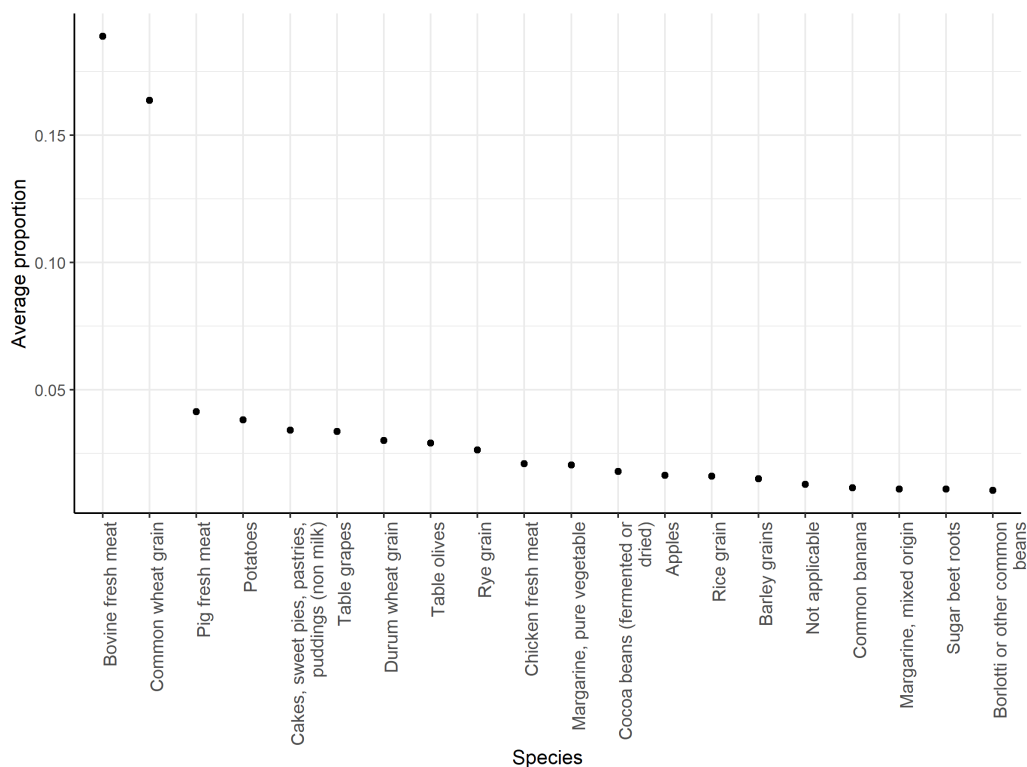
Figure 4.13: Abundance curve of the average energy that the twenty most abundant species contributed to the diet of a person using the full dataset (n=476,768).
