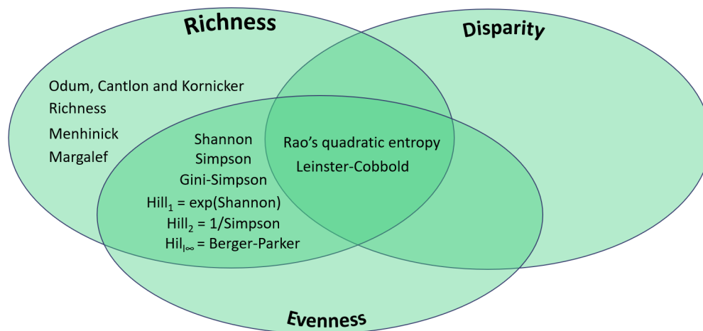
Figure 4.15: All possible indices in this thesis represented by Venn diagram based on the components of biodiversity they incorporate.
