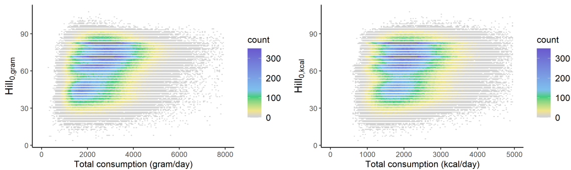
Figure 4.14: Hill_{0,gram} and Hill_{0,kcal} based on total consumption using the full dataset ( n=476,768 ).
