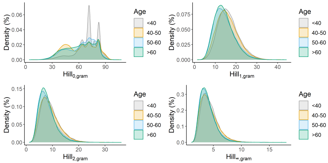
Figure A3: Association between weight-based indices and age at recruitment using the full dataset (n=476,768).
