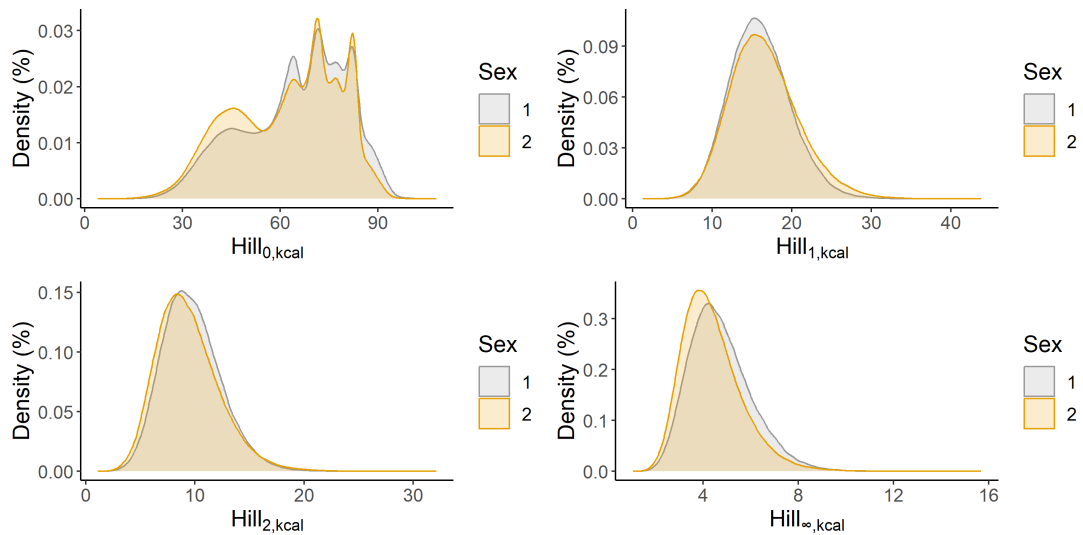
Figure A2: Association between energy-based indices and gender using the full dataset (n=476,768).
