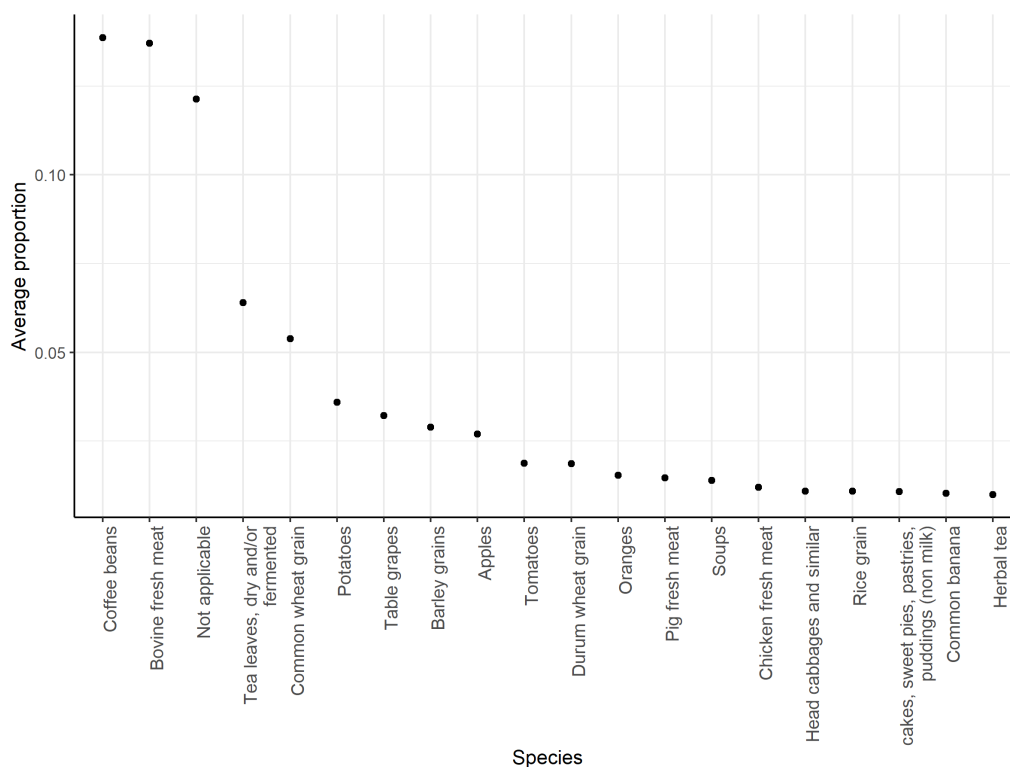
Figure 4.12: Abundance curve of average amount that the twenty most abundant species contributed to the diet of a person using the full dataset ( n=476,768 ).
