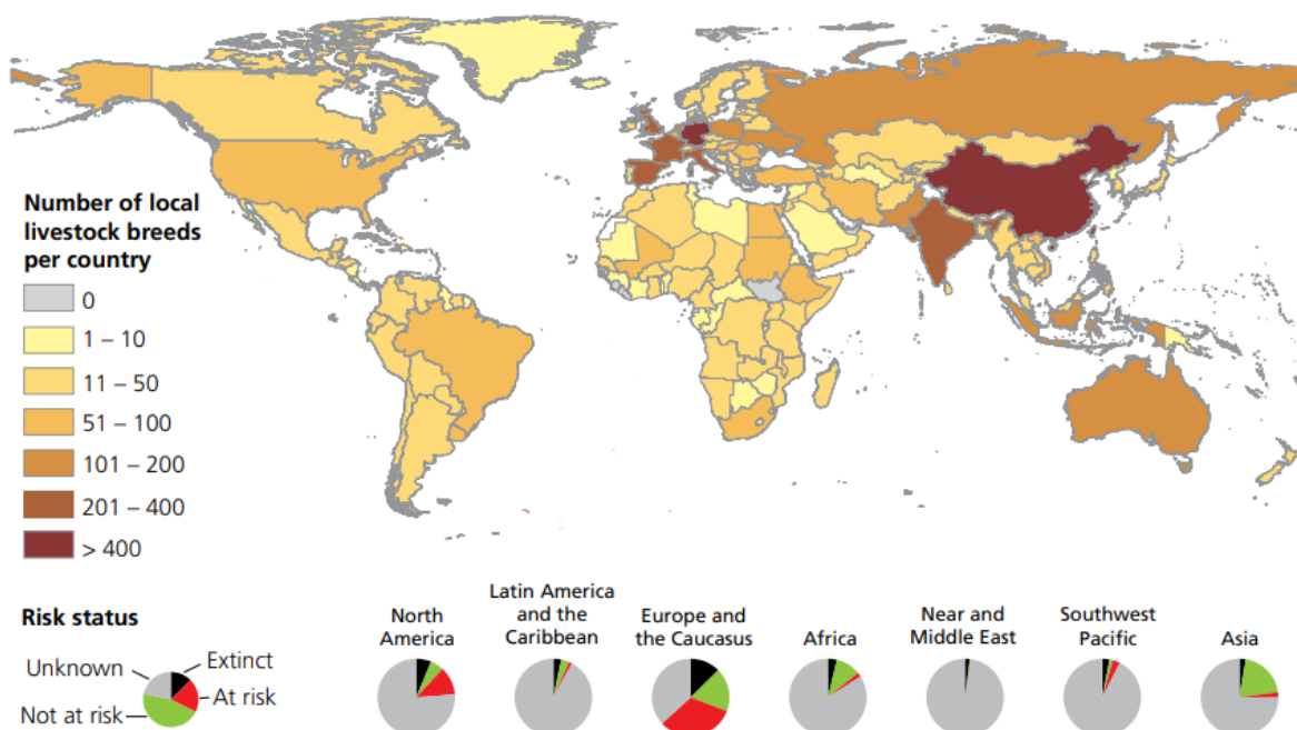
Figure 2.2: Global map with threat status of livestock breeds. From CGRFA (2015b).
