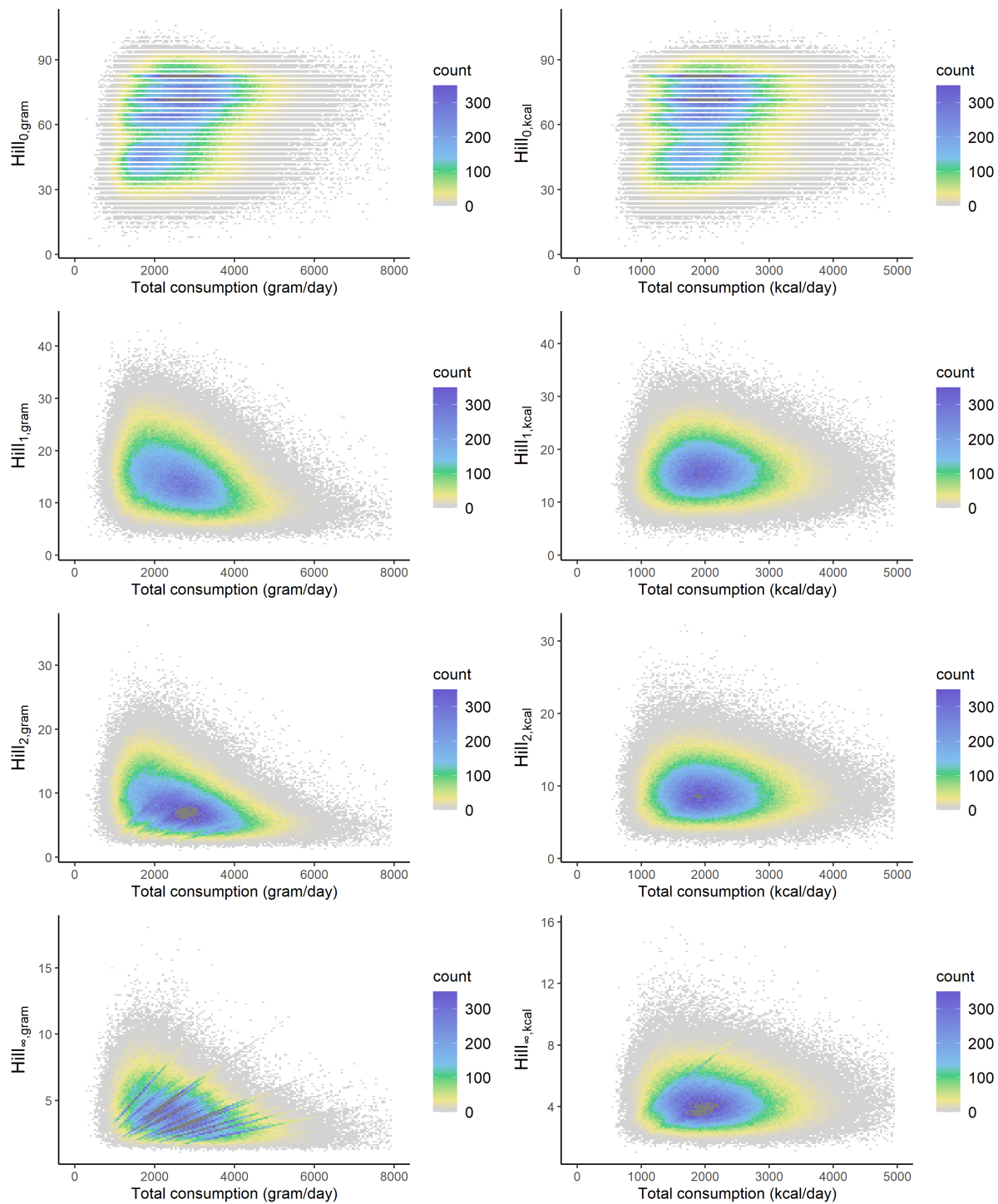
Figure A8: Weight-based and energy-based Hill numbers based on total consumption per day (n=476,768).
