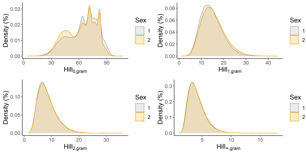
Figure A1: Association between weight-based indices and gender using the full dataset (n=476,768).
