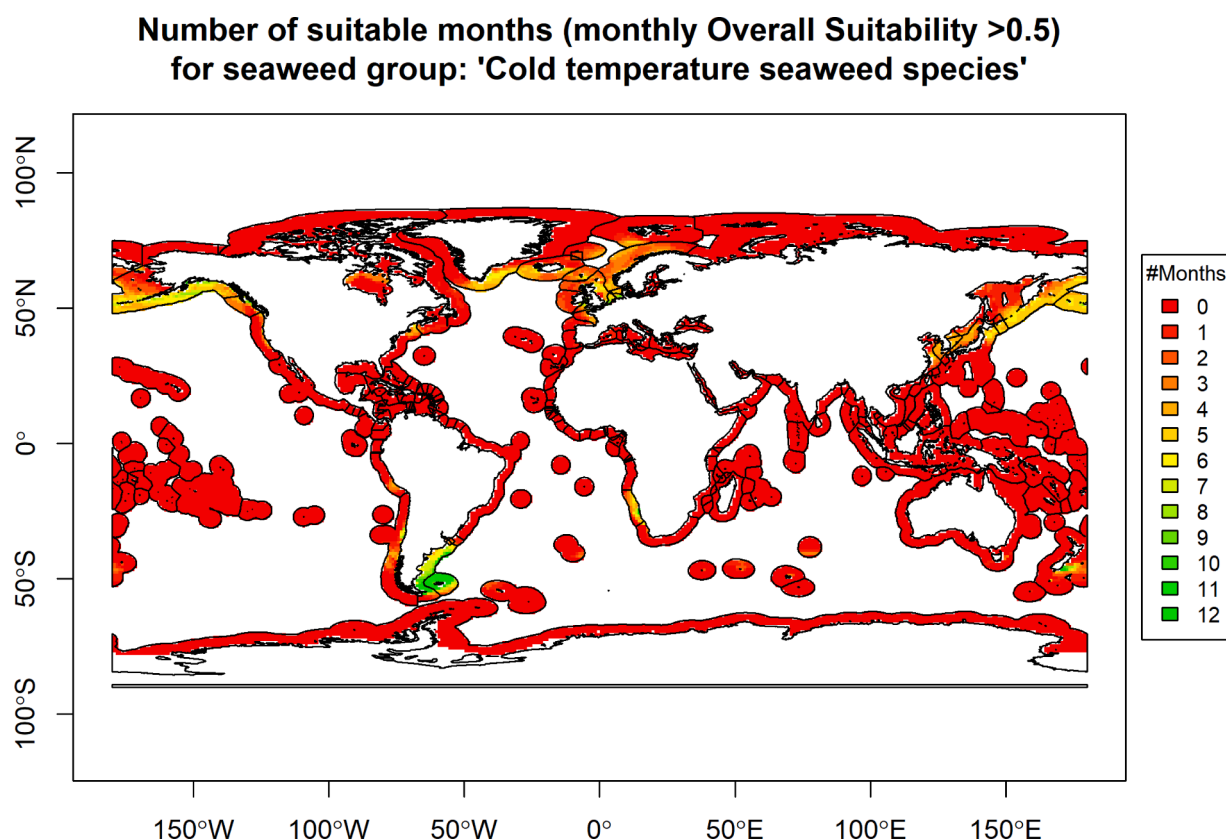
Fig. 8. Months with overall monthly suitability > 0.5 for the cold temperature seaweeds group inside the EEZ. Scenario with suitability dependent on Significant Wave height.
