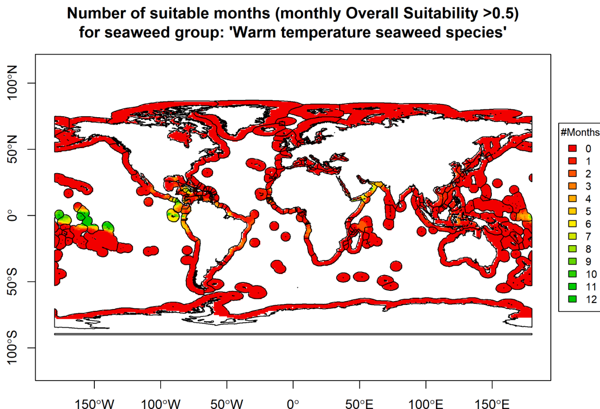
Fig. 10. Months with overall monthly suitability > 0.5 for the warm temperature seaweeds group. Optimistic nutrient uptake scenario. The black line 200 nautical miles out of shore is the EEZ.
