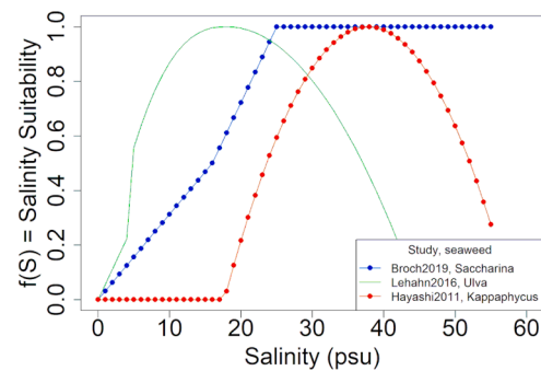
Fig. 6. Salinity response function. Colours refer to seaweeds with different temperature niches: cold (blue), intermediate (green) and warm (red). Lines marked with solid dots were used for global modelling (For interpretation of the references to color in this figure legend, the reader is referred to the web version of this article.).
