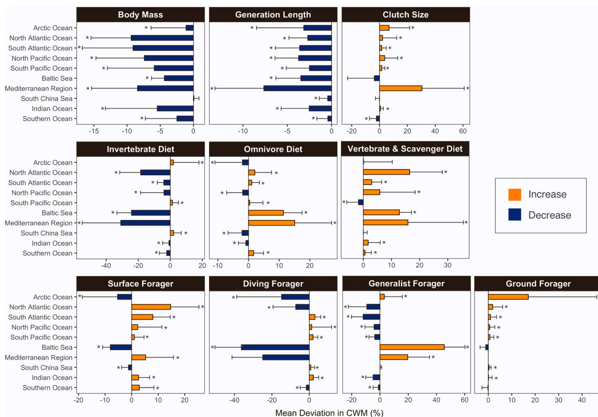
Fig. 3. Mean ( \pm standard deviation) shift in community weighted mean (CWM) within each marine region following removal of 146 bycatch-threatened species in areas where their distributions overlap with fishing activity. Orange represents a positive shift (increase in average trait value or frequency), and blue a negative shift (decrease in average trait value or frequency) in the CWM following removal of species threatened from bycatch. The marine region of South China Sea refers to South China and Eastern Archipelagic Seas. Stars indicate significantly nonzero averages.
