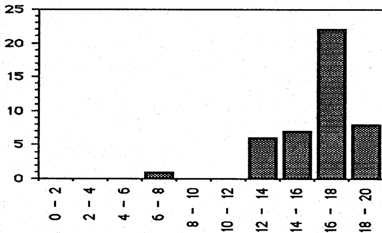
Figure 9. Speed of the ship at the time of observation (kts): (a) mean value for each ship (b) numbers of ships with mean speeds in the ranges shown.
