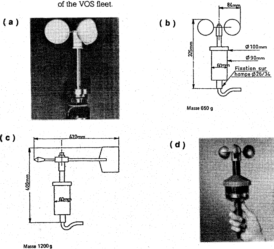
Figure 13 Types of anemometer used by the VSOP-NA ships. (a - c) Anemometer and wind vane of the "Pommar" met system (France). (d) Handheld anemometer (France).
