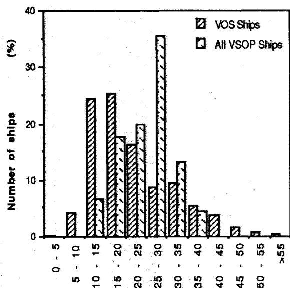
Figure 8. Histograms of the distribution of temperature measurement heights on the VSOP-NA ships and of the observing platform height on the VOS ships.
