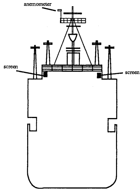
Midship - Front View
