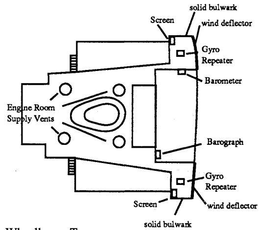
Wheelhouse Top
