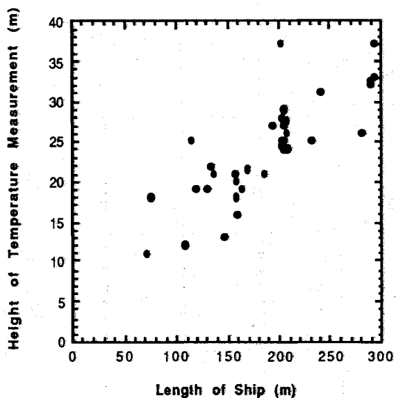
Figure 7 Relationship between the height of the temperature measurement and the length of the ship.
