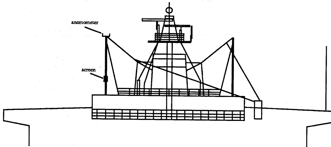
Wheelhouse - Front View
