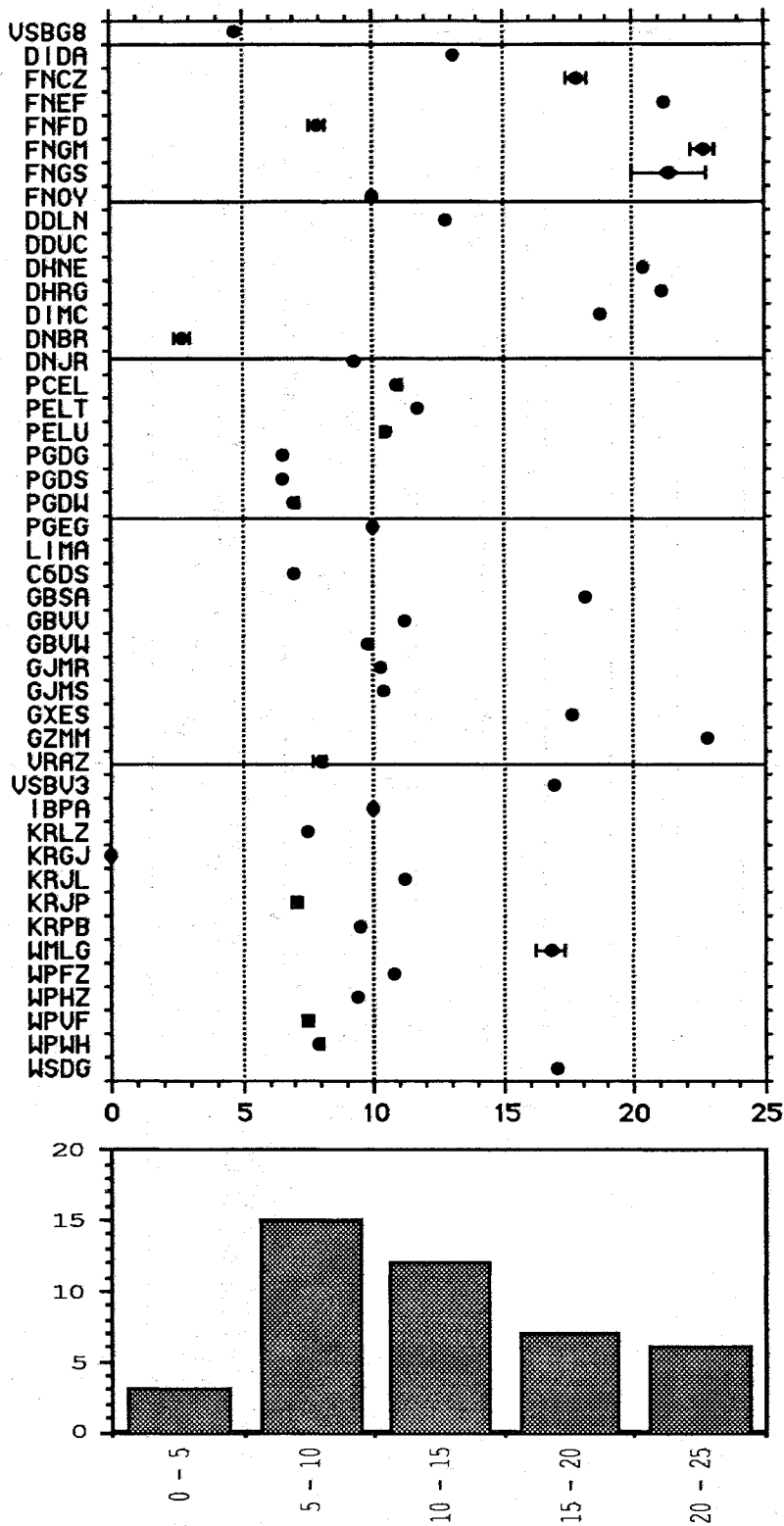
Figure 10. Height of cargo above main deck (m): (a) height and reported variation for each ship (b) numbers of ships with cargo heights in the ranges shown.
