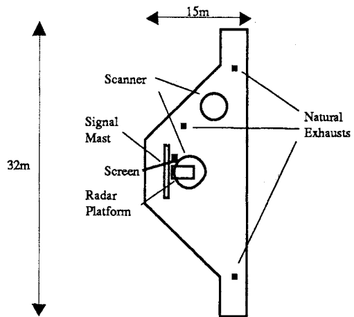
Plan of Wheelhouse Top
