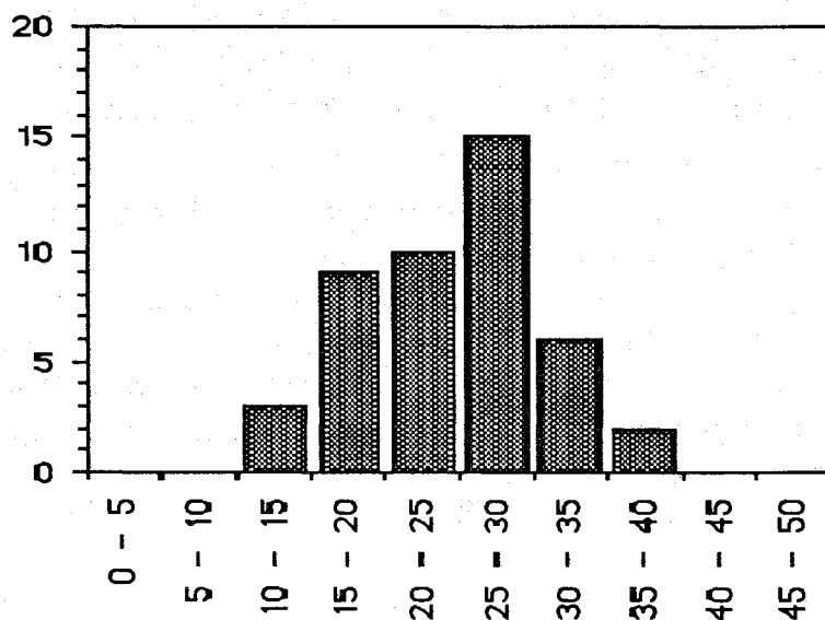
Figure 14 Height of the temperature and humidity measurements (m): (a) height for each ship (b) numbers of ships with measurement heights in the ranges shown.
