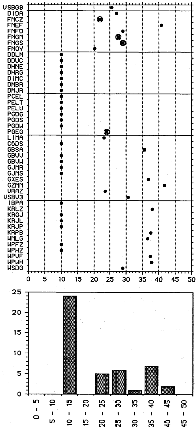
Figure 11 Height of the anemometer (m) or effective height of visual wind estimate: (a) height and reported variation for each ship (b) numbers of ships with wind measurement heights in the ranges shown. Visual estimates are shown at 10m, handheld anemometers are ringed.
