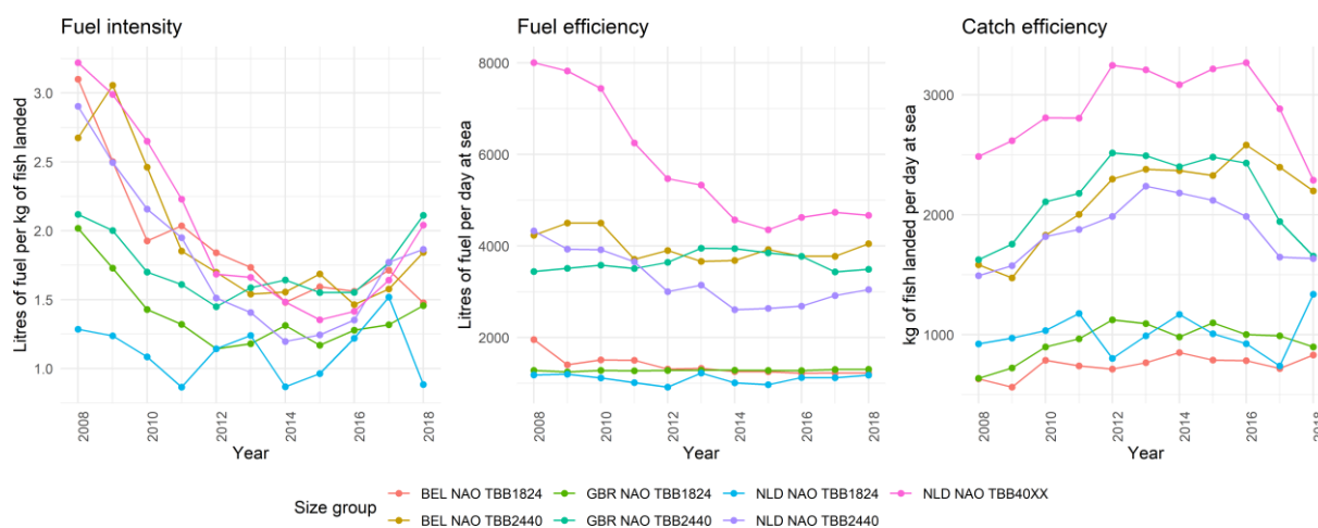
Figure 5-2: Re-construction of fuel intensity (fuel use to catch one kg of fish), fuel efficiency (liters fuel used per unit of effort) and catch efficiency (Bastardie, Feary, Brunel et al. 2022).
