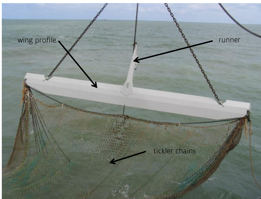
Figure 2-6: Illustration of the wing profile of the Sumwing (ILVO).
