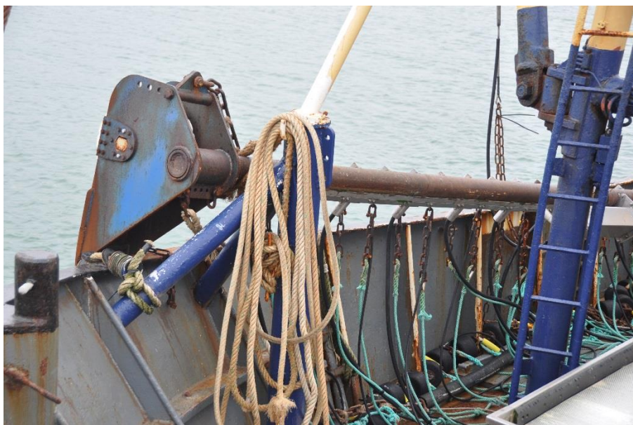
Figure 2-13: Illustration of a shrimp pulse trawl (ILVO).
