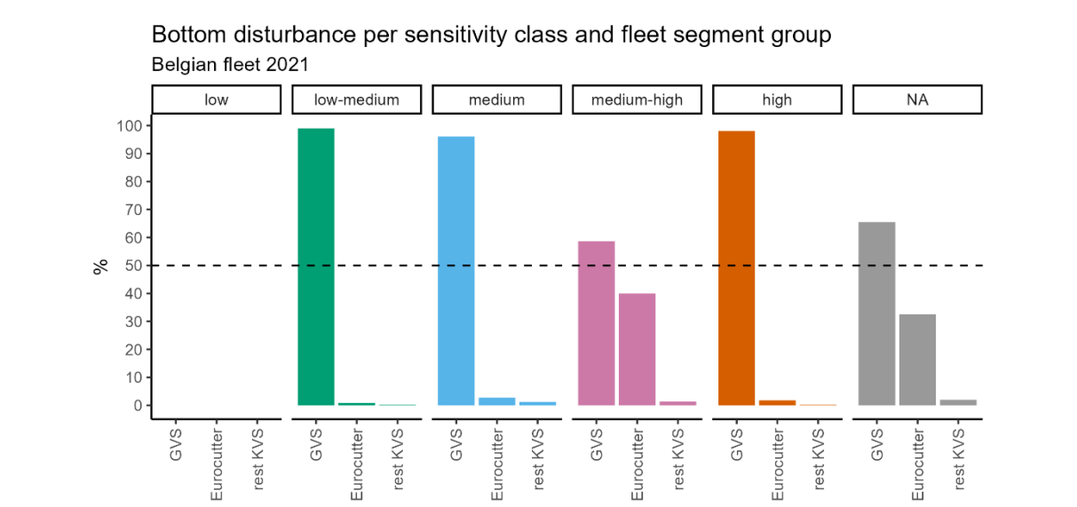
Figure 4-5: Share of the total bottom disturbance (in %) contributed by each fleet segment group for the different sensitivity classes. NA represents missing sensitivity.
