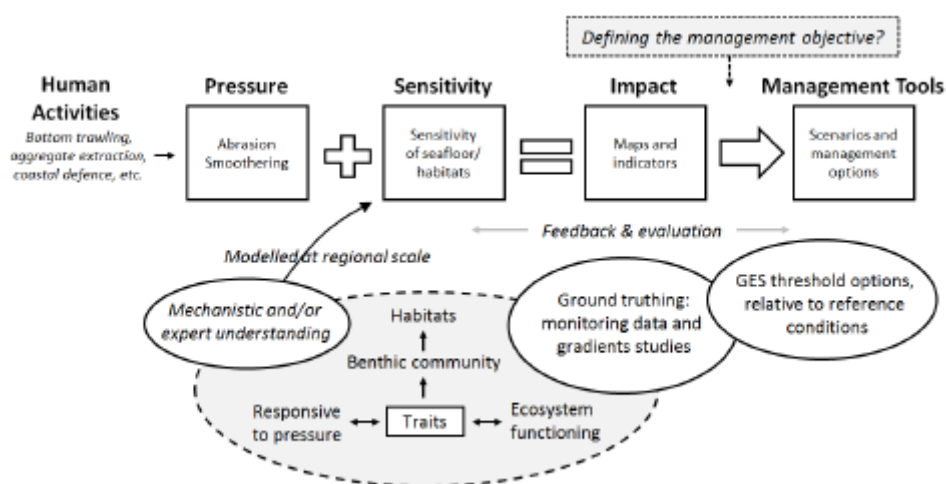
Figure 3-8: Conceptual diagram of the steps taken in developing management tools for assessing pressure and impact on the seafloor from human activity
