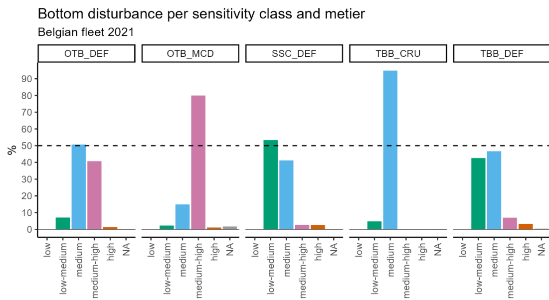
Figure 4-7: Share of the total bottom disturbance (in %) per sensitivity classes for the different métiers. DRB_MOL was omitted. NA represents missing sensitivity.
