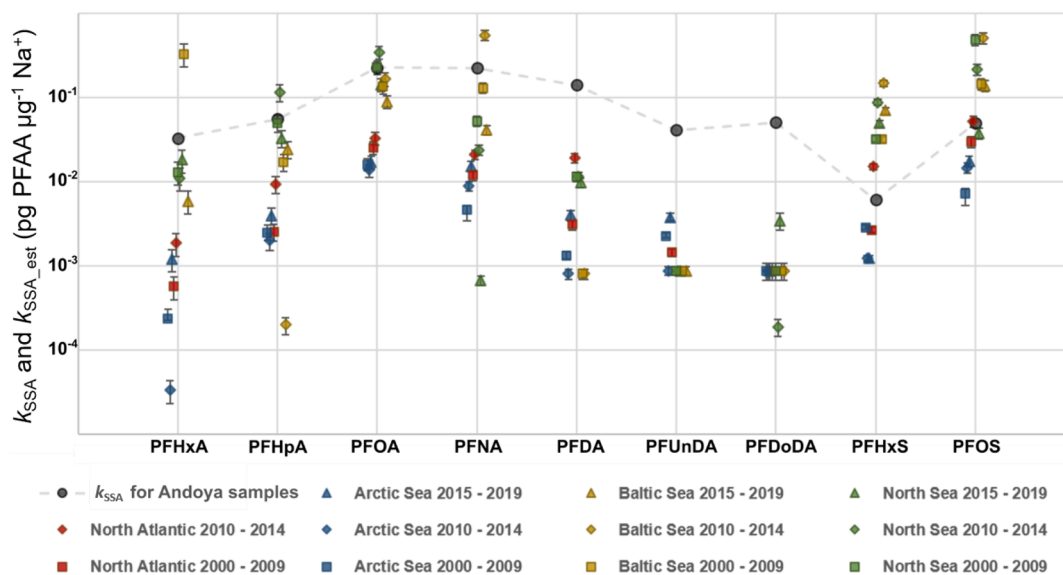
Figure 4. Comparison between the k_{SSA} determined by the linear fit ( \log_{10}[\text{PFAA}] = \log_{10}(k_{SSA} \times [\text{Na}^+] + [\text{PFAA}]_{\text{other}} ) and the estimation, k_{SSA\_est} based on previous laboratory results and median PFAA seawater concentrations from the literature. The error bar represents the standard deviation of k_{SSA\_est} [\text{PFAA}]_{\text{seawater}} \times (\text{EF}_{\text{Mean}} \pm \text{SD}) .
