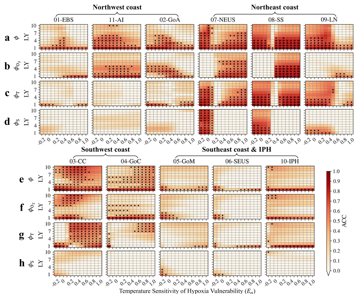
Fig. 7 | Differences in predictability of habitat viability ( \phi ) among different E_o (temperature sensitivity of hypoxia vulnerability) species and those of the oxygen ( \phi_{O_2} ), temperature ( \phi_T ), and salinity ( \phi_S ) components, in the upper-200 m of the eleven Large Marine Ecosystems (LMEs) using the decadal prediction system. a Difference in predictability of the \phi assessed as Anomaly Correlation Coefficient (ACC) among different E_o species in the northwest and northeast coast LMEs. The x-axis of each panel represents the E_o trait ranging from
