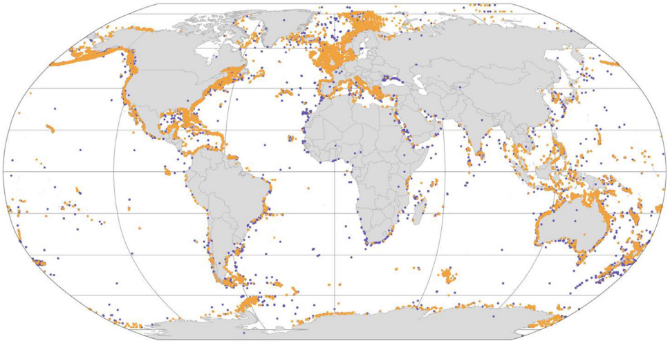
Fig. 1. Global map of demersal sponge records. Points in orange represent occurrences that are flagged as correct, while points in purple indicate potentially inaccurate records based on their known vertical and bathymetric ranges and/or on land.
