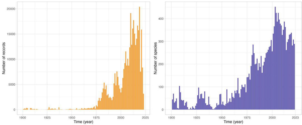
Fig. 2. Number of demersal sponge (a) records and (b) species available in the demersal sponge dataset per year (data are available since the year 1776. To improve visualization, the few records before 1900 were removed from the graph).
