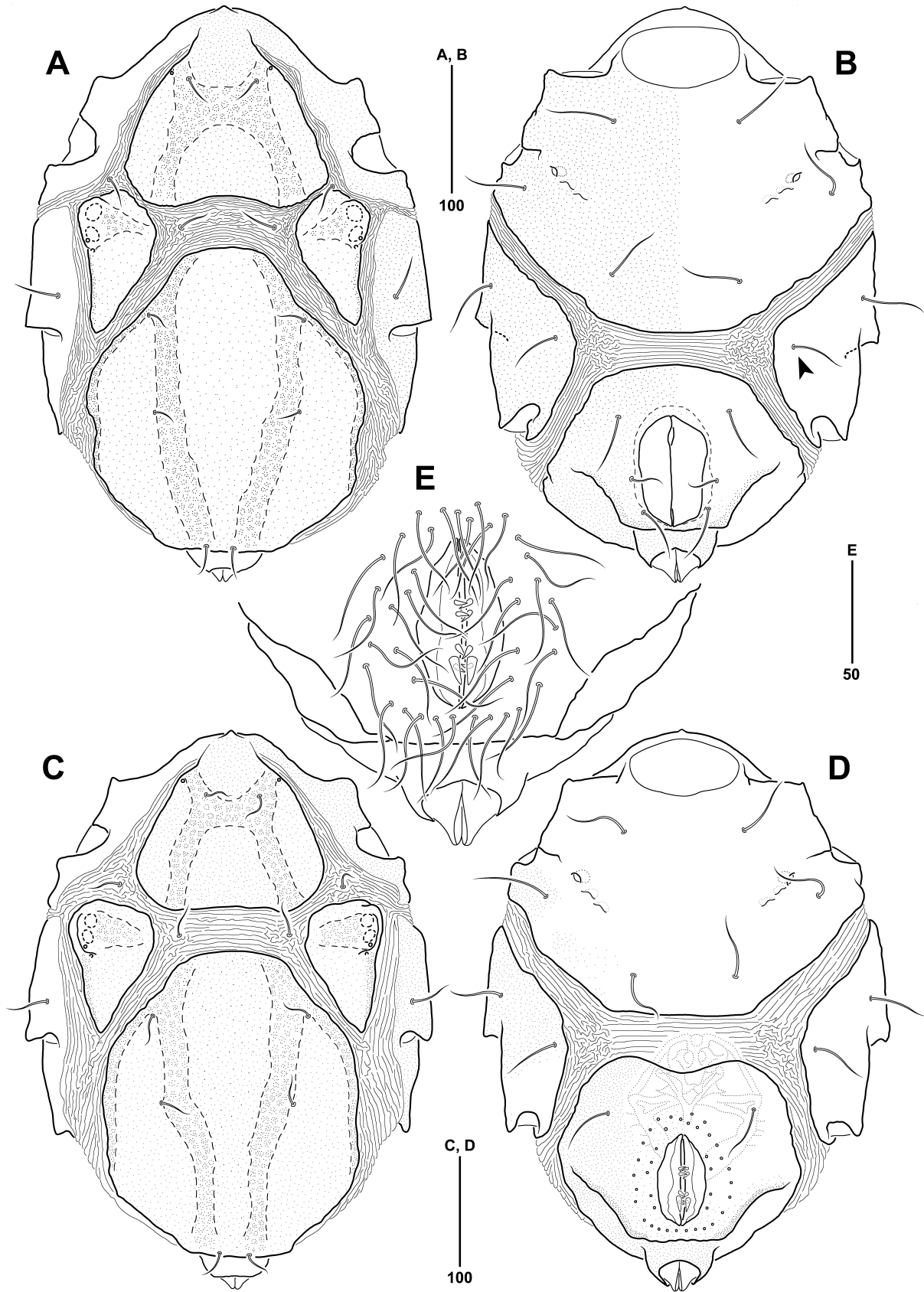
Figure 1 Agauopsis bisetosa n. sp. A, B, female (HNIBRIV11667): A – Idiosoma, dorsal; B – Idiosoma, ventral. C–E, male (HNIBRIV11668): C – Idiosoma, dorsal; D – Idiosoma, ventral; E – pgs and sgs on GA.
