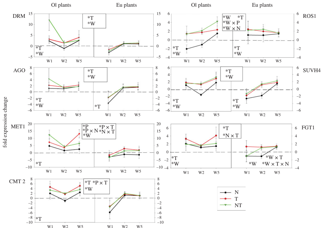
Figure 2. Expression dynamics of GOIs involved in de novo DNAm (DRM and AGO) and its maintenance (MET1 and CMT2), DNA demethylation (ROS1) and histone methylation (SUVH4) measured in both OI and Eu plants under different stress conditions (N = nutrients; T = temperature, NT = nutrients + temperature) compared to control (dashed line). Significant differences resulting from three-way RM-GLM are reported in the central square, while results of two-way RM-GLM performed individually for OI and Eu plants are shown in the bottom left corner of each graph. Data are mean \pm s.e. ( n = 3 ).
