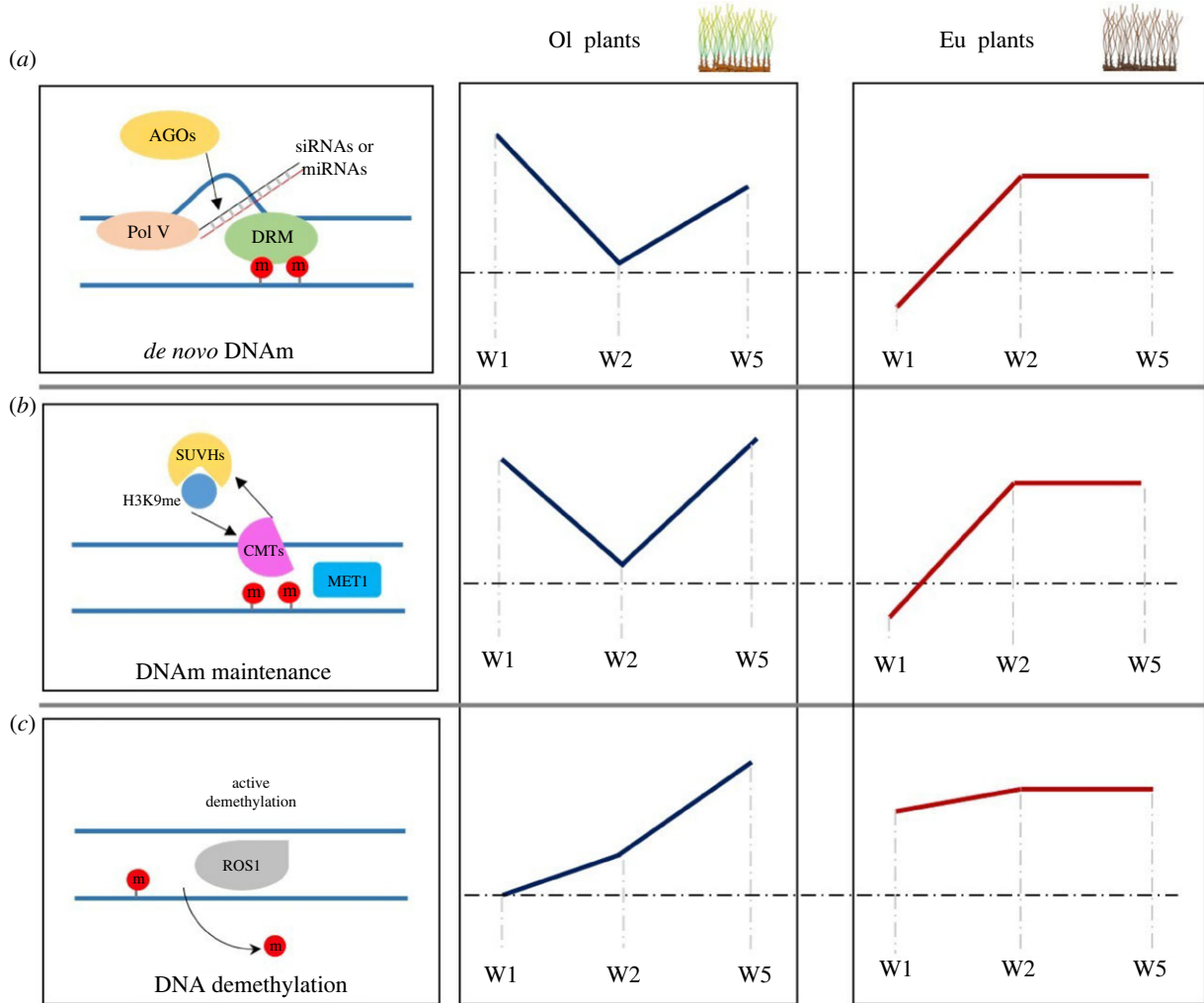
Figure 3. Graph showing gene expression patterns observed in OI and Eu plants during the exposure phases (W1 = one week; W2 = two weeks; W5 = five weeks). (a) De novo DNAm involves a plant-specific RNA polymerase V (Pol V) which produces non-coding RNA transcripts that act as a scaffold to recruit AGOs and DRM through base-pairing of associated siRNAs; (b) DNAm maintenance operated by DNA methyltransferase 1 (MET1) and chromomethylases (CMTs) through the interaction with H3K9-specific methyltransferases (SUVHs); (c) DNA active demethylation is mediated by repressor of silencing 1 (ROS1) which is a bifunctional 5-mC DNA glycosylase inducing the excision of the 5-mC base from the DNA backbone. Blue (OI plants) and red (Eu plants) lines refer to the general expression patterns of analysed genes under different experimental conditions over time. The horizontal dashed line represents the control (expression of reference genes).
