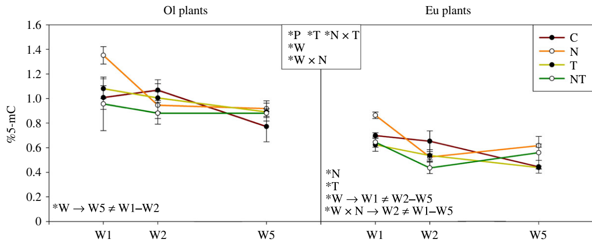
Figure 1. Global % of methylated cytosine (% 5-mC) measured in OI and Eu plants (P) during the course of the experiment (W1 = one week; W2 = two weeks; W5 = five weeks of the exposure) for the different treatments (N = nutrients; T = temperature; NT = nutrients + temperature). Significant differences resulting from three-way RM-GLM are reported in the central square, while results of two-way RM-GLM and post hoc tests performed individually for OI and Eu plants, are shown in the bottom left corner of each graph. Data are mean \pm s.e. ( n = 3 ).
