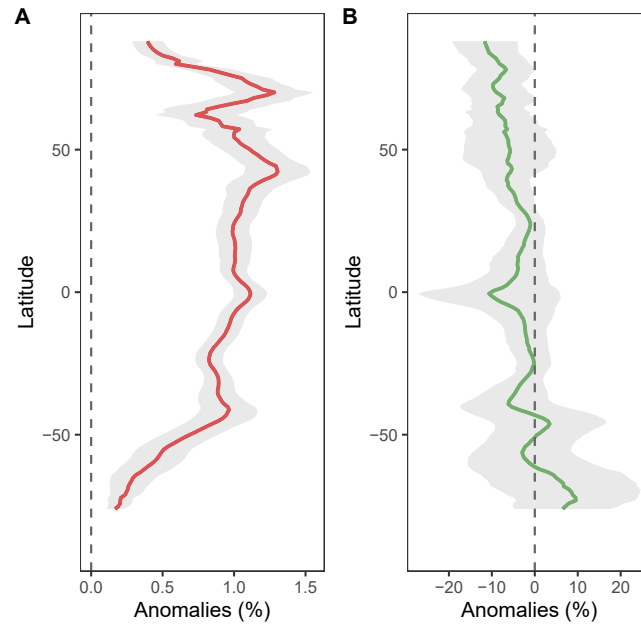
Figure S11. Projected Latitudinal Changes in SST and chl a, Related to Figures 4 and S12
