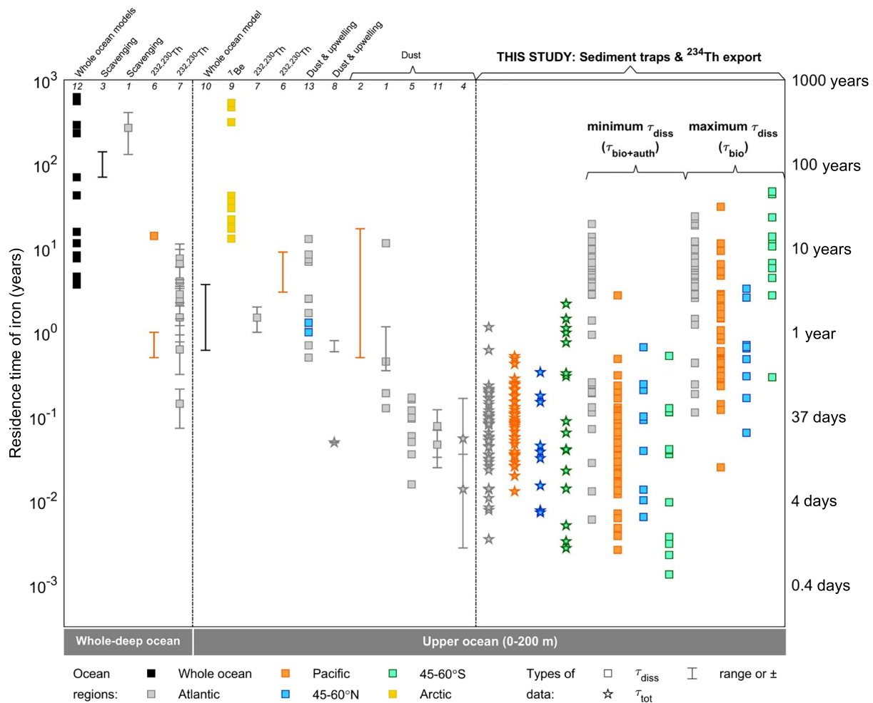
Figure 3. Compilation of iron residence times in the global ocean. Each symbol represents an estimate from a unique location or a depth layer (e.g., 500–5,000 m). The upper x-axis lists the methods for determining \tau , including direct measurements of inputs or processes (e.g., upwelling), models, and isotope tracer of dust and scavenging ( ^{232}\text{Th} , ^{230}\text{Th} , ^{234}\text{Th} , ^{238}\text{U} ). Previously published upper ocean residence times (left and center panels) are generally \tau_{\text{diss}} (squares) and restricted to the Atlantic. This study quadruples the existing dataset, adding new export-based \tau_{\text{tot}} (stars) and \tau_{\text{diss}} (right panel). These new \tau are from diverse regions and are shorter, on average, than prior upper ocean estimates (center panel). Minimum \tau_{\text{diss}} and maximum \tau_{\text{diss}} are determined with respect to removal by biological and abiotic processes ( F_{\text{bio+auth}} , Equation 5) and biological processes alone ( F_{\text{bio}} , Equation 4). Reference numbers are indicated along the upper axis (1-Bergquist & Boyle, 2006; 2-Boyle et al., 2005; 3-Bruland et al., 1994; 4-Buck et al., 2010; 5-Croot et al., 2004; 6-Hayes et al., 2015; 7-Hayes, Anderson, et al., 2018; 8-Jickells, 1999; 9-Kadko et al., 2019; 10-Moore et al., 2004; 11-Sarthou et al., 2003; 12-Tagliabue et al., 2016; 13-Ussher et al., 2013).
