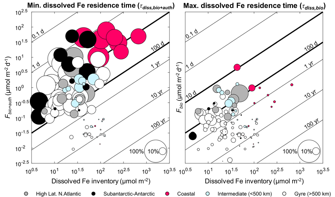
Figure 4. Residence times of dissolved iron. Upper ocean residence times (diagonal lines) for this study were determined using semi-simultaneously measured dissolved Fe inventories, Fe export ( F_{\text{tot}} ), and element ratios from sinking particles (i.e., Fe:P and Fe:Al). The minimum (left) and maximum (right) bounds on the residence time of dissolved Fe are shown with respect to Fe removal via biological and authigenic Fe export (left, \tau_{\text{bio+auth}} ) and via biological processes only (right, \tau_{\text{bio}} ). In the left panel, the marker diameter represents F_{\text{bio+auth}}/F_{\text{tot}} or the percentage of the total Fe export that is biological Fe or authigenic Fe. In the right panel, the marker diameter is F_{\text{bio}}/F_{\text{tot}} . The data shown ( n = 99 for each panel) represent the locations where F_{\text{bio}} and F_{\text{bio+auth}} are calculable. Due to the sequence of determination for the flux fractions, estimates of F_{\text{auth}} are the most uncertain and in some cases are zero.
