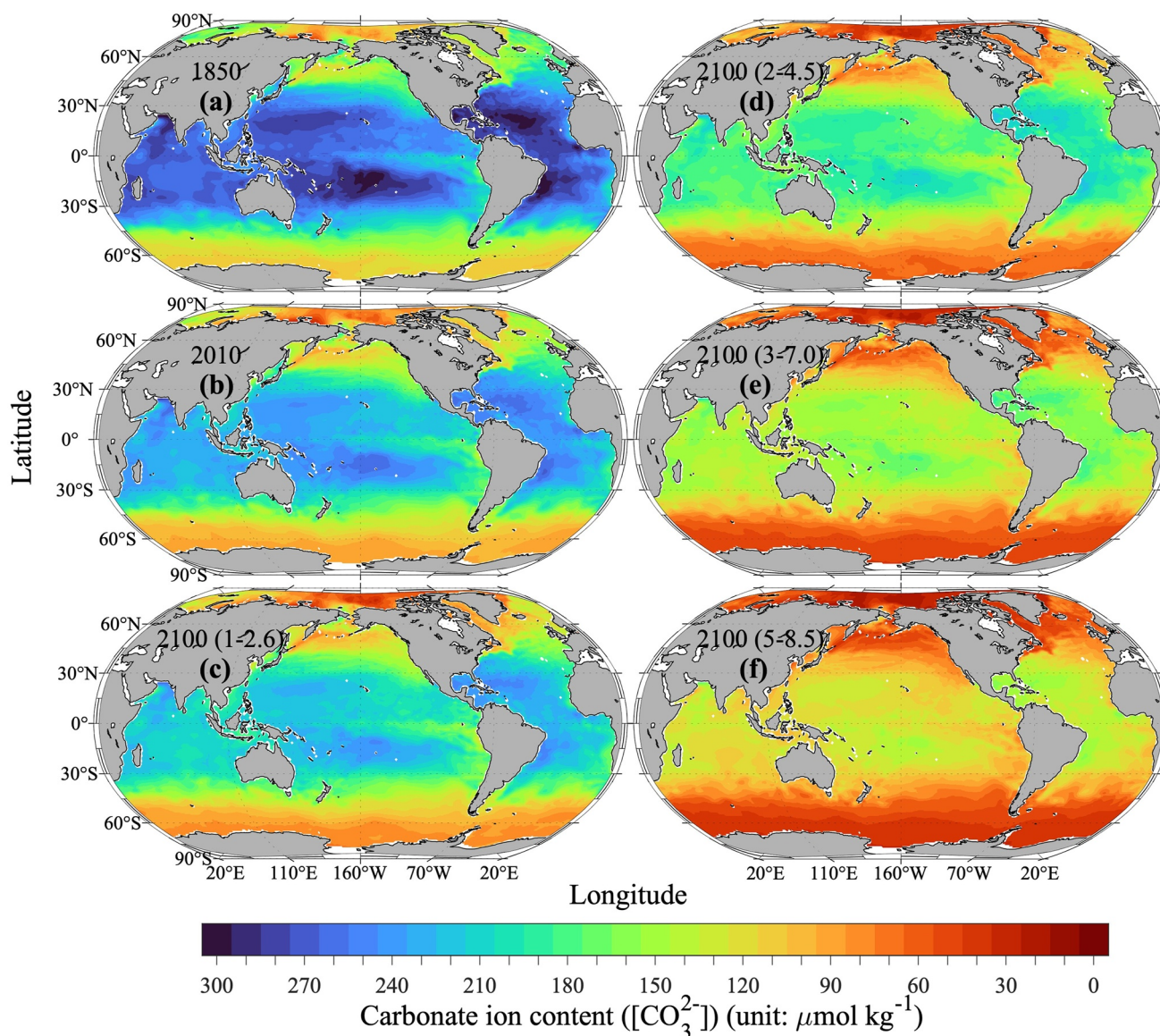
Figure 8. Surface ocean carbonate ion content ( [CO_3^{2-}] , inter-model median) in the decades around (a) 1850, (b) 2010, (c) 2100 (SSP1-2.6), (d) 2100 (SSP2-4.5), (e) 2100 (SSP3-7.0), and (f) 2100 (SSP5-8.5). SSP is short for Shared Socioeconomic Pathway.
