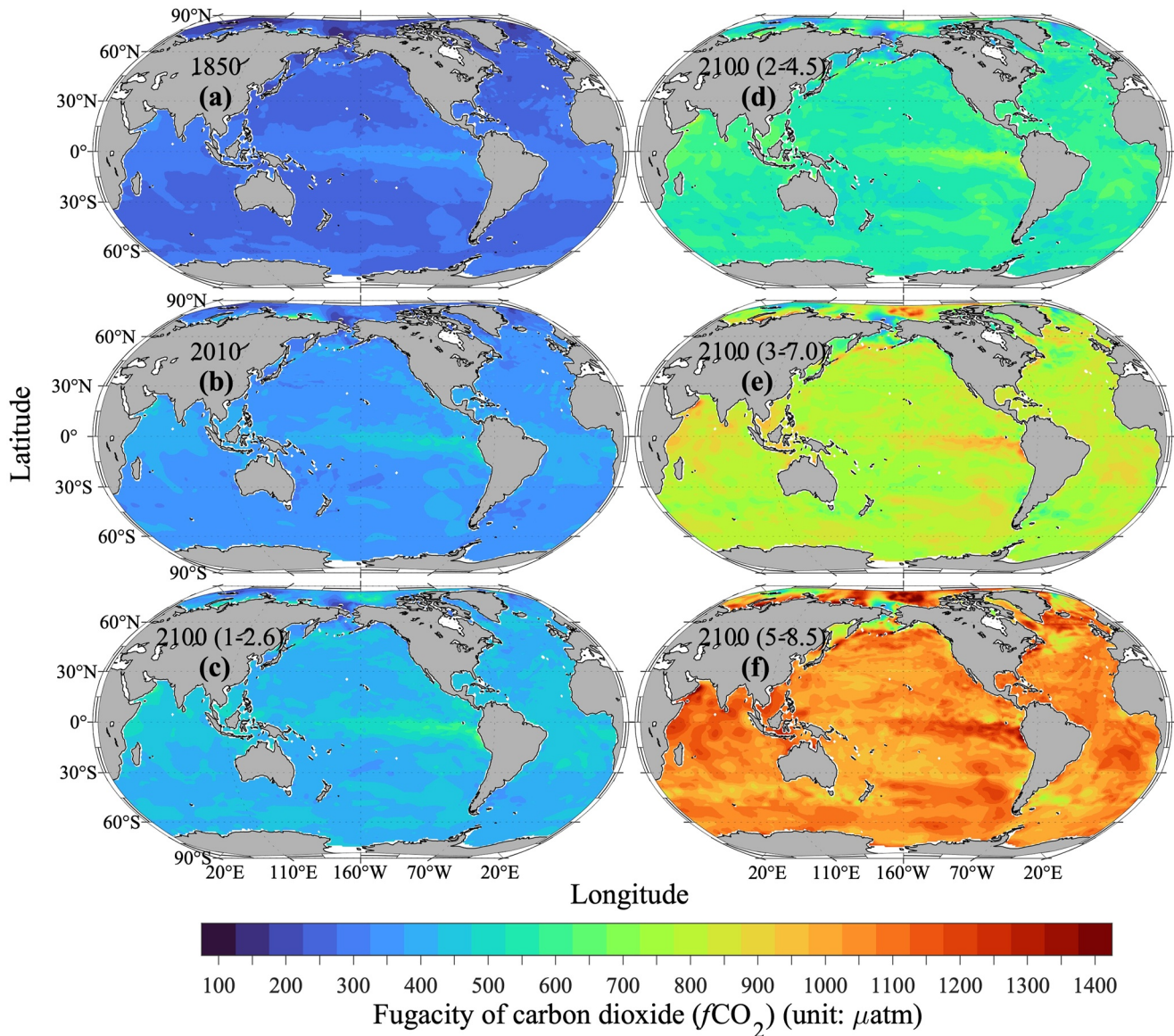
Figure 5. Surface ocean fugacity of carbon dioxide ( f\text{CO}_2 , inter-model median) in the decades around (a) 1850, (b) 2010, (c) 2100 (SSP1-2.6), (d) 2100 (SSP2-4.5), (e) 2100 (SSP3-7.0), and (f) 2100 (SSP5-8.5). SSP is short for Shared Socioeconomic Pathway.
