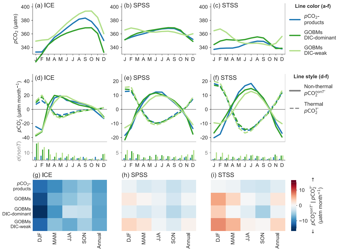
Figure 7. (a–c): The climatological seasonal cycle of p\text{CO}_2 on a monthly scale. (d–f): Seasonal cycle of the rate of change of the thermal ( p\text{CO}_2^{\text{T}} , dashed lines) and non-thermal ( p\text{CO}_2^{\text{nonT}} , solid lines) components of ocean surface p\text{CO}_2 on monthly time scales given in \mu\text{atm month}^{-1} (Equation 2). The bars on the bottom show standard deviations of the non-thermal component. Models have been grouped into DIC-dominant/weak, where the DIC-weak models have a thermal contribution > 0 for the mean of the subtropical seasonally stratified and subpolar seasonally stratified (shown in panel (g–i); see Figure S11 in Supporting Information S1 for individual global and regional ocean biogeochemistry models, and Table S2 in Supporting Information S1 for the DIC-dominant/weak model groups). (g–i): \lambda p\text{CO}_2 , the difference of the thermal and non-thermal (dissolved inorganic carbon [DIC]) components of ocean surface p\text{CO}_2 as in Mongwe et al. (2018). When \lambda p\text{CO}_2 > 0 (red) indicates temperature dominance, and \lambda p\text{CO}_2 < 0 (blue) indicates that the non-thermal component (i.e., DIC) is dominant. The MPI model is excluded in this analysis.
