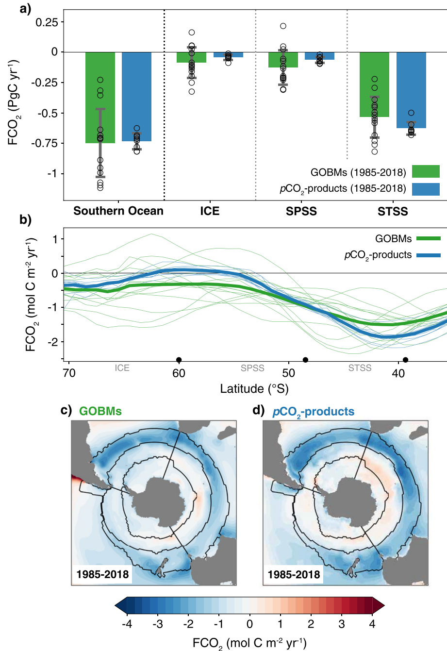
Figure 2. Temporal average of the Southern Ocean CO 2 net flux (FCO 2 ). A positive flux denotes outgassing from ocean to atmosphere. The temporal average is calculated over the period 1985 to 2018 for the global ocean biogeochemistry models (GOBMs) and pCO 2 -products (Tables 1 and 2). (a) The green and blue bar plots show the ensemble mean of the GOBMs and pCO 2 -based data-products, and open circles indicate the individual GOBMs and pCO 2 -products. The ensemble standard deviation (1σ) is shown by the error bars. The river flux adjustment added to the GOBMs is small (0.04 PgC yr -1 ), its distribution over the biomes is described in Section 2.3.1. (b) Zonal mean flux density of the different data sets. Thick green and blue lines show the ensemble means, and thin green and blue lines show the individual GOBMs and pCO 2 -products. Approximate boundaries for biomes are marked with black points on the x-axis. (c, d) Maps of spatial distribution of net CO 2 flux for ensemble means of GOBMs, and pCO 2 -products.
