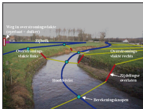
Figuur 1: Quasi-2D hydrodynamische overstromingsmodellering.
