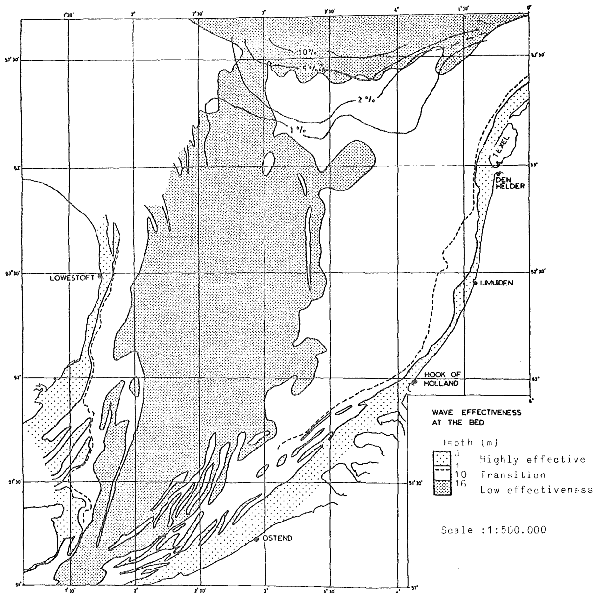
fig. 12.- Regions of high, transitional and low wave effectiveness at the bed (Southern Bight of the North Sea). Between 53°N and 53°40'N contours of percent mud ( \% < 50 \mu ) in the bottom sediments are shown. There is a fairly rapid increase in mud percent in the region of low wave effectiveness. From McCave (1971).
