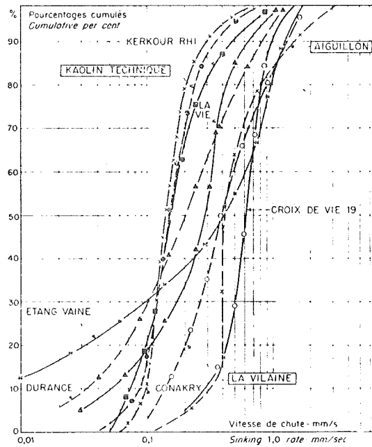
fig. 2.- Examples of sinking rate curves for flocculant media. From Migriot (1968).
