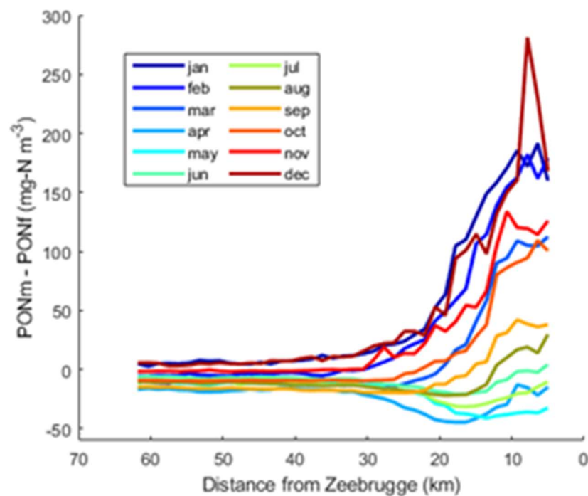
Figure 3.3: Monthly values of PON_m - PON_f as a function of the distance from the coast (Zeebrugge) along the transect of Figure 2.1 (monthly values are a multiyear average from 2017 to 2021).
