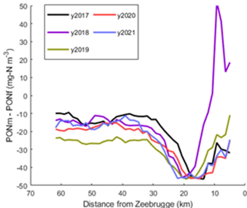
Figure 3.2: April values of PON_m - PON_f along the transect for years 2017 to 2021.
