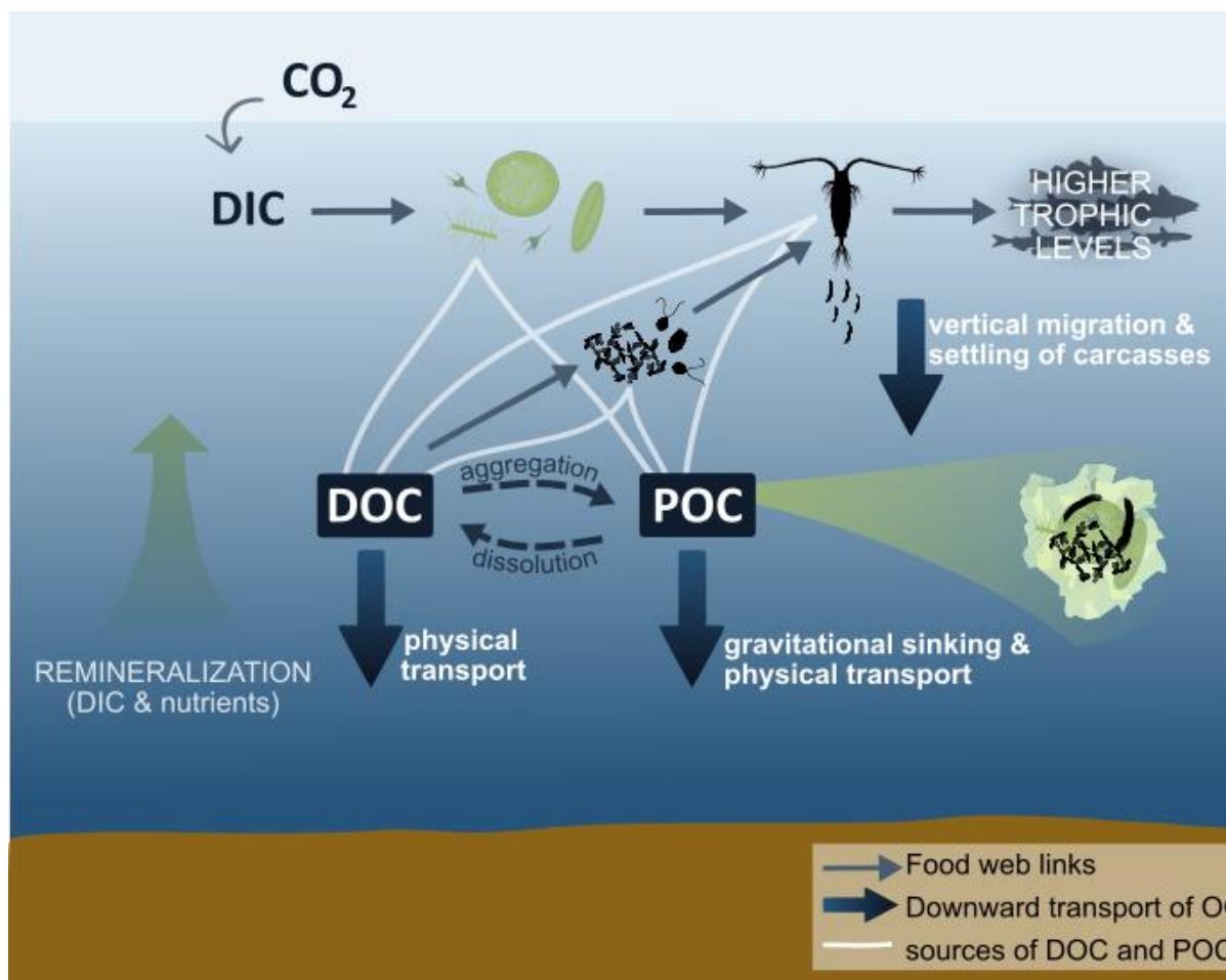
Figure 1: Carbon pathways within the biological carbon pump. \text{DIC} is fixed by phytoplankton through photosynthesis and converted to particulate organic carbon ( \text{POC} ), which is taken up by zooplankton and further channeled through higher trophic levels via the classical food web. Dissolved organic carbon ( \text{DOC} ) is produced additionally by phytoplankton through excretion or cell lysis, or by other organisms through feeding, excretion, or senescence. Carbon is “returned” to the food web by the microbial loop through the uptake of \text{DOC} by bacteria. \text{DOC} and \text{POC} pools are in constant exchange through aggregation and dissolution processes. Several mechanisms lead to the export of organic carbon from surface layers and the escape of its remineralization in the food web: gravitational sinking or physical transport of aggregates; physical transport or aggregation, and subsequent downward transport of \text{DOC} ; vertical migration and settling of carcasses of zooplankton and higher trophic levels.
